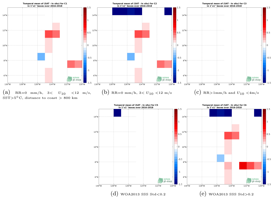
Figure 12: Temporal mean gridded over spatial boxes of size 1^\circ \times 1^\circ of \Delta SSS (SMAP SSS L2 v5.0 (JPL) - TSG (SAMOS)) for 5 different subdatasets corresponding to:RR=0 mm/h, 3 < U_{10} < 12 m/s, SST >5^\circ\text{C} , distance to coast > 800 km (a), RR=0 mm/h, 3 < U_{10} < 12 m/s (b), RR >1 mm/h and U_{10} < 4 m/s (c), WOA2013 SSS Std <0.2 (d), WOA2013 SSS Std >0.2 (e).
