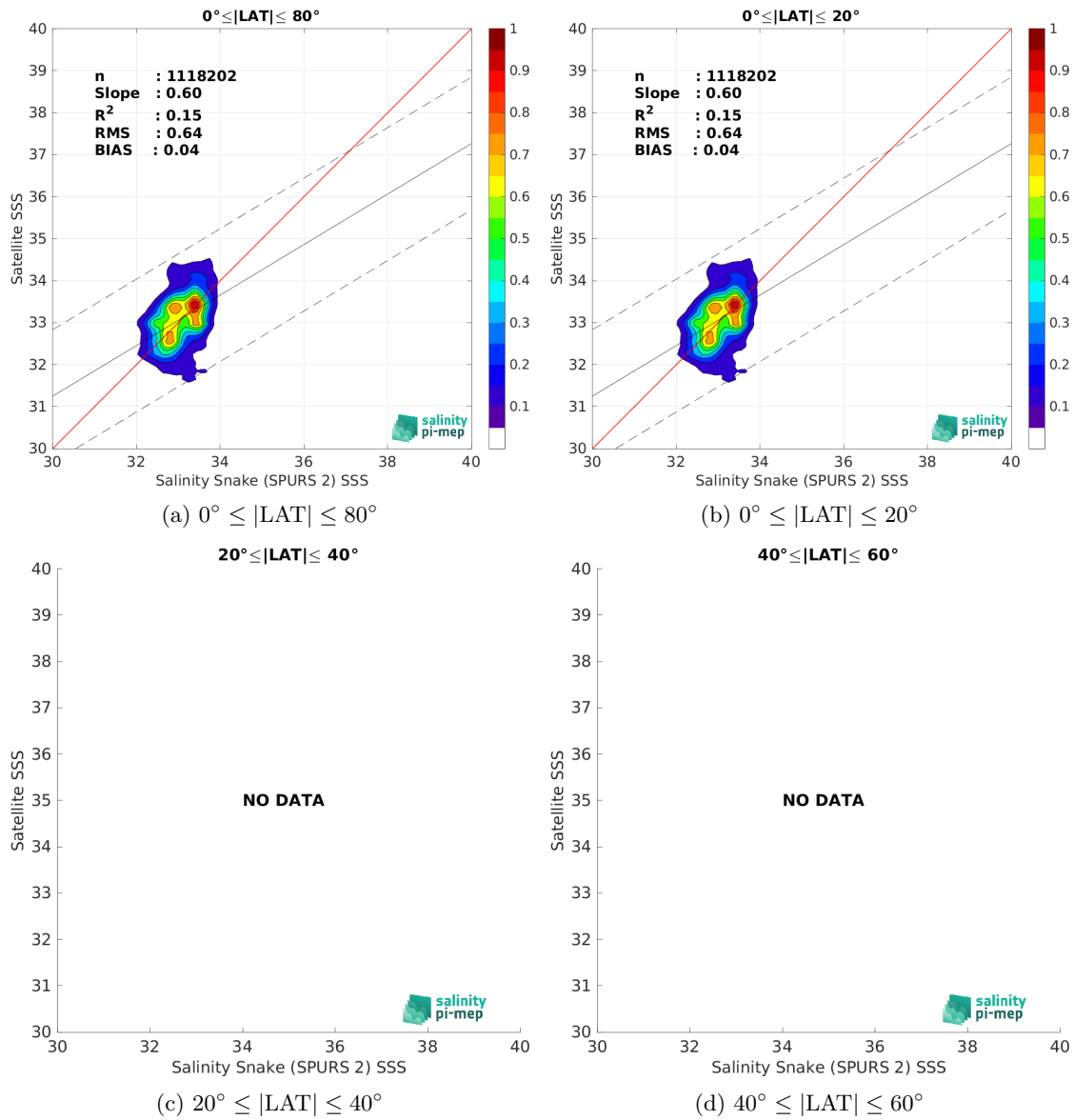
Figure 10: Contour maps of the concentration of SMAP SSS L2 v5.0 (JPL) SSS (y-axis) versus Salinity Snake (SPURS 2) SSS (x-axis) at match-up pairs for different latitude bands. For each plot, the red line shows x=y . The black thin and dashed lines indicate a linear fit through the data cloud and the \pm 95\% confidence levels, respectively. The number match-up pairs n , the slope and R^2 coefficient of the linear fit, the root mean square (RMS) and the mean bias between satellite and in situ data are indicated for each latitude band in each plots.
