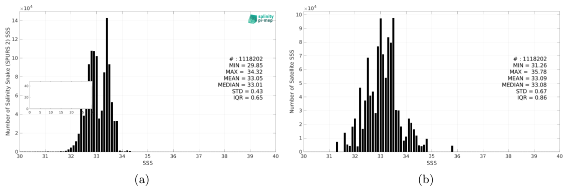
Figure 3: Histograms of SSS from Salinity Snake (SPURS 2) (a) and SMAP SSS L2 v5.0 (JPL) (b) considering all match-up pairs per bins of 0.1 over the SPURS 2 Pi-MEP region and for the full satellite product period.
