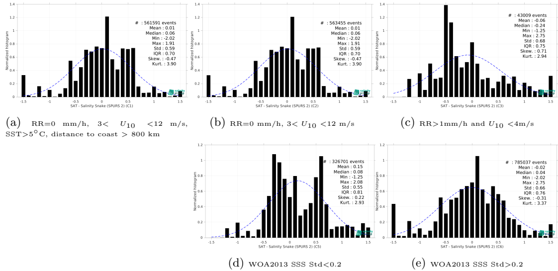
Figure 15: Normalized histogram of \Delta SSS (SMAP SSS L2 v5.0 (JPL) - Salinity Snake (SPURS 2)) for 5 different subdatasets corresponding to: RR=0 mm/h, 3 < U_{10} < 12 m/s, SST > 5°C, distance to coast > 800 km (a), RR=0 mm/h, 3 < U_{10} < 12 m/s (b), RR > 1mm/h and U_{10} < 4 m/s (c), WOA2013 SSS Std < 0.2 (d), WOA2013 SSS Std > 0.2 (e).
