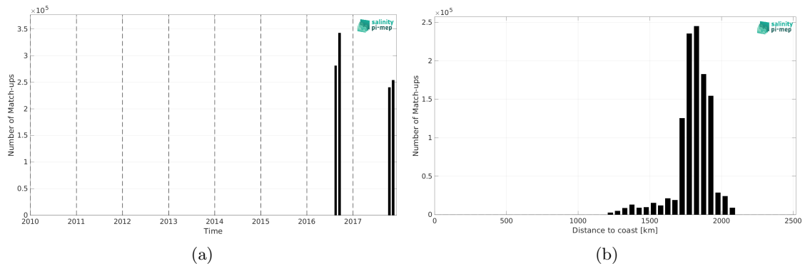
Figure 2: Number of match-ups between Salinity Snake (SPURS 2) and SMAP SSS L2 v5.0 (JPL) SSS as a function of time (a) and as function of the distance to coast (b) over the SPURS 2 Pi-MEP region and for the full satellite product period.
