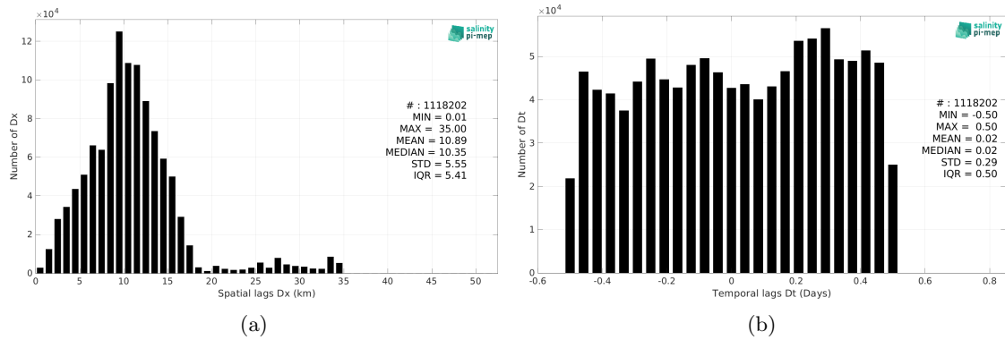
Figure 6: Histograms of the spatial (a) and temporal (b) lags between the location/time of the Salinity Snake (SPURS 2) measurement and the date of the corresponding SMAP SSS L2 v5.0 (JPL) SSS pixel.
