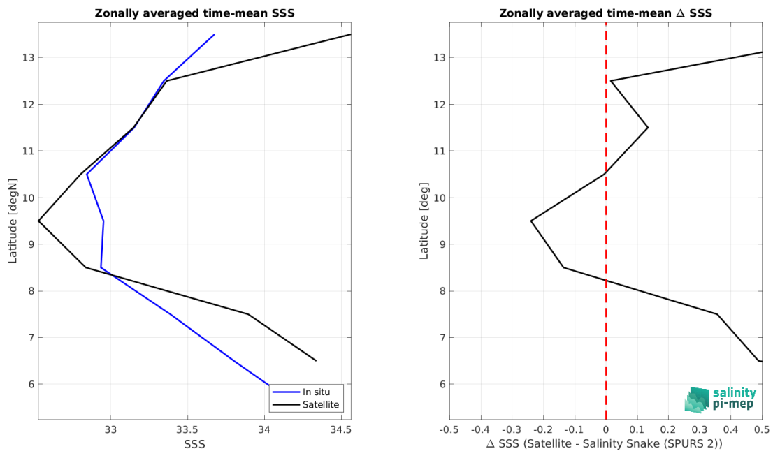
Figure 9: Left panel: Zonal mean SSS from SMAP SSS L2 v5.0 (JPL) satellite product (black) and from Salinity Snake (SPURS 2) (blue). Right panel: Zonal mean of \Delta SSS (Satellite - Salinity Snake (SPURS 2)) for all the collected Pi-MEP match-up pairs estimated over the full satellite product period.
