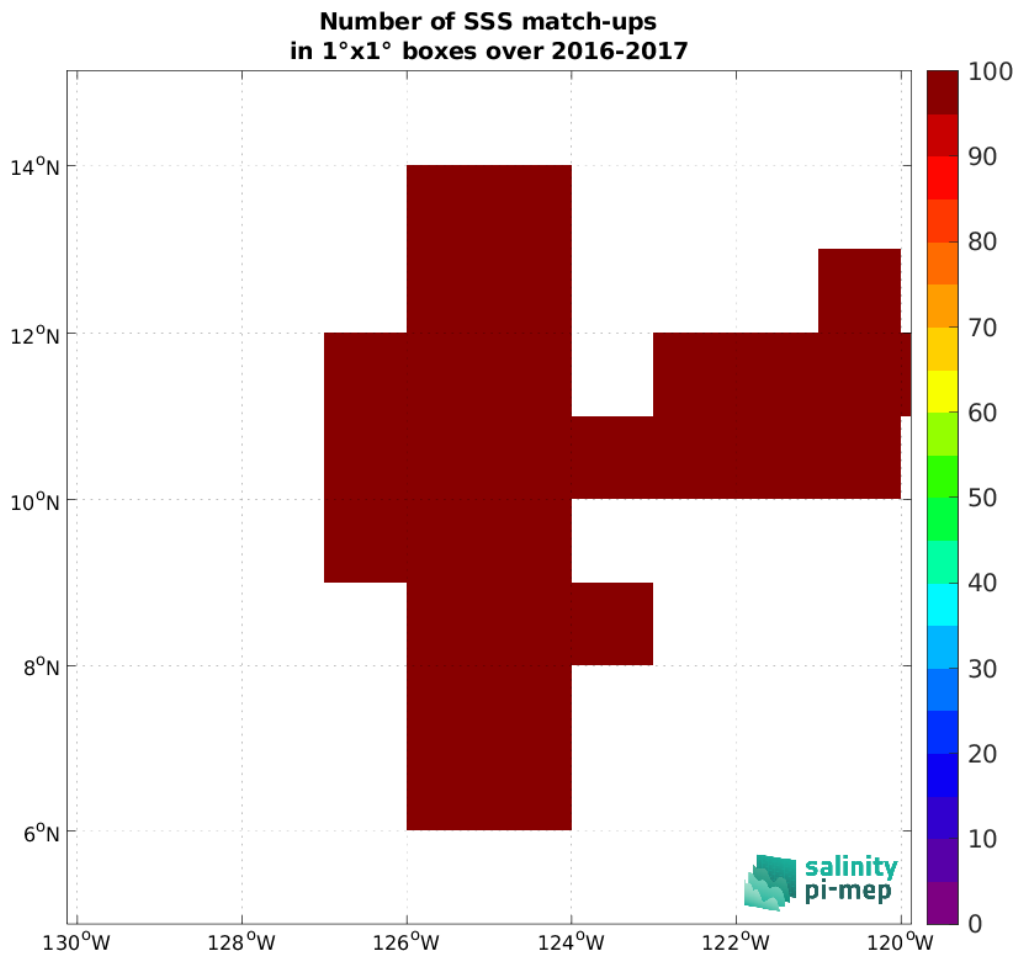
Figure 5: Number of SSS match-ups between Salinity Snake (SPURS 2) SSS and the SMAP SSS L2 v5.0 (JPL) SSS product for the SPURS 2 Pi-MEP region over 1°x1° boxes and for the full satellite product period.
