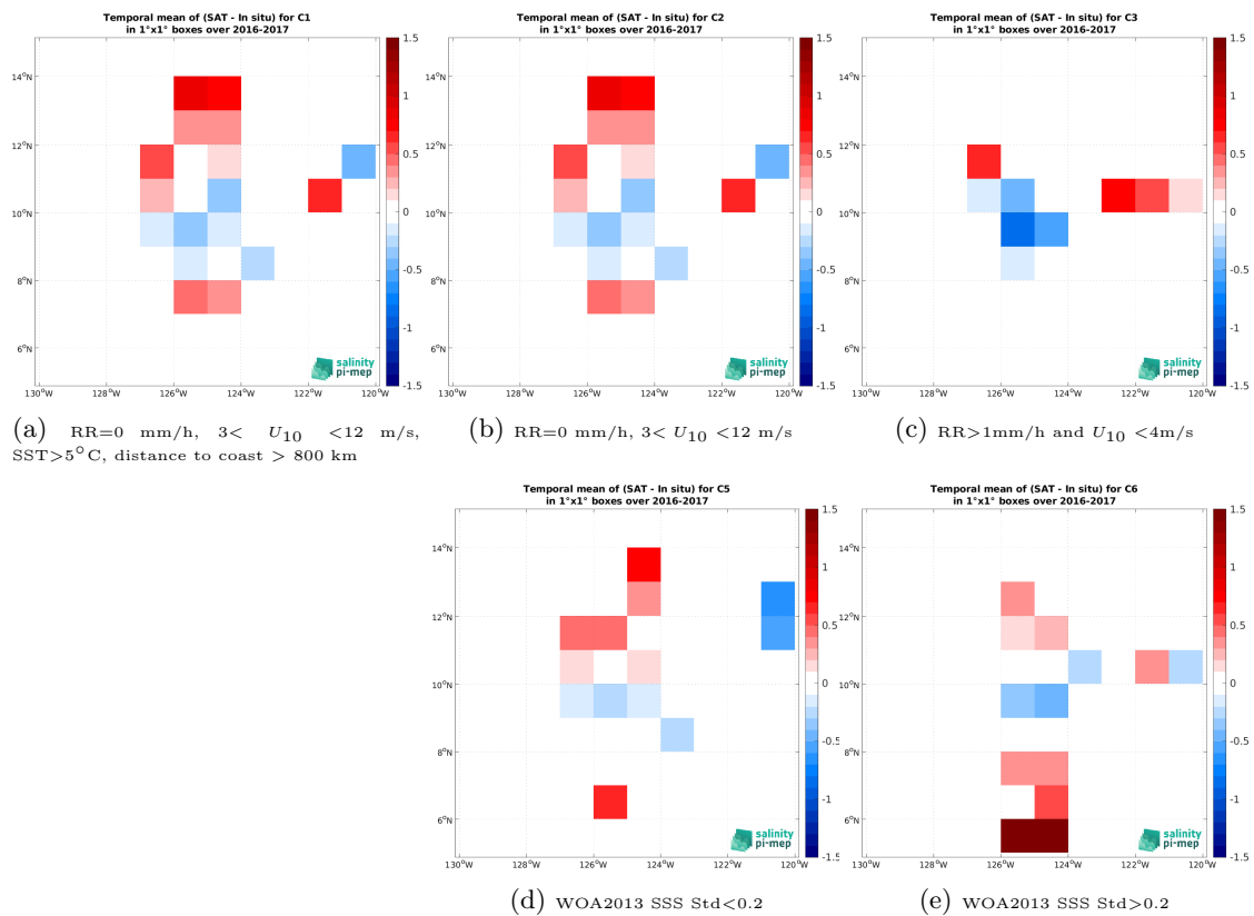
Figure 14: Temporal mean gridded over spatial boxes of size 1^\circ \times 1^\circ of \Delta\text{SSS} (SMAP SSS L2 v5.0 (JPL) - Salinity Snake (SPURS 2)) for 5 different subdatasets corresponding to: RR=0 mm/h, 3 < U_{10} < 12 m/s, SST > 5°C, distance to coast > 800 km (a), RR=0 mm/h, 3 < U_{10} < 12 m/s (b), RR > 1mm/h and U_{10} < 4 m/s (c), WOA2013 SSS Std < 0.2 (d), WOA2013 SSS Std > 0.2 (e).
