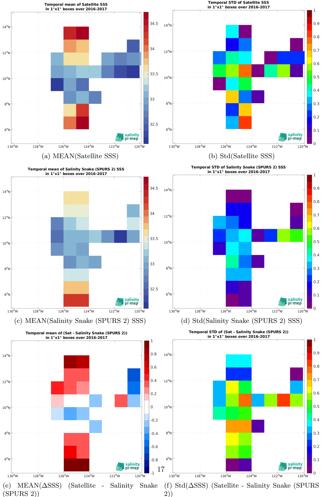
Figure 7: Temporal mean (left) and Std (right) of SSS from SMAP SSS L2 v5.0 (JPL) (top), Salinity Snake (SPURS 2) (middle), and of \Delta SSS (Satellite - Salinity Snake (SPURS 2)). Only match-up pairs are used to generate these maps.
