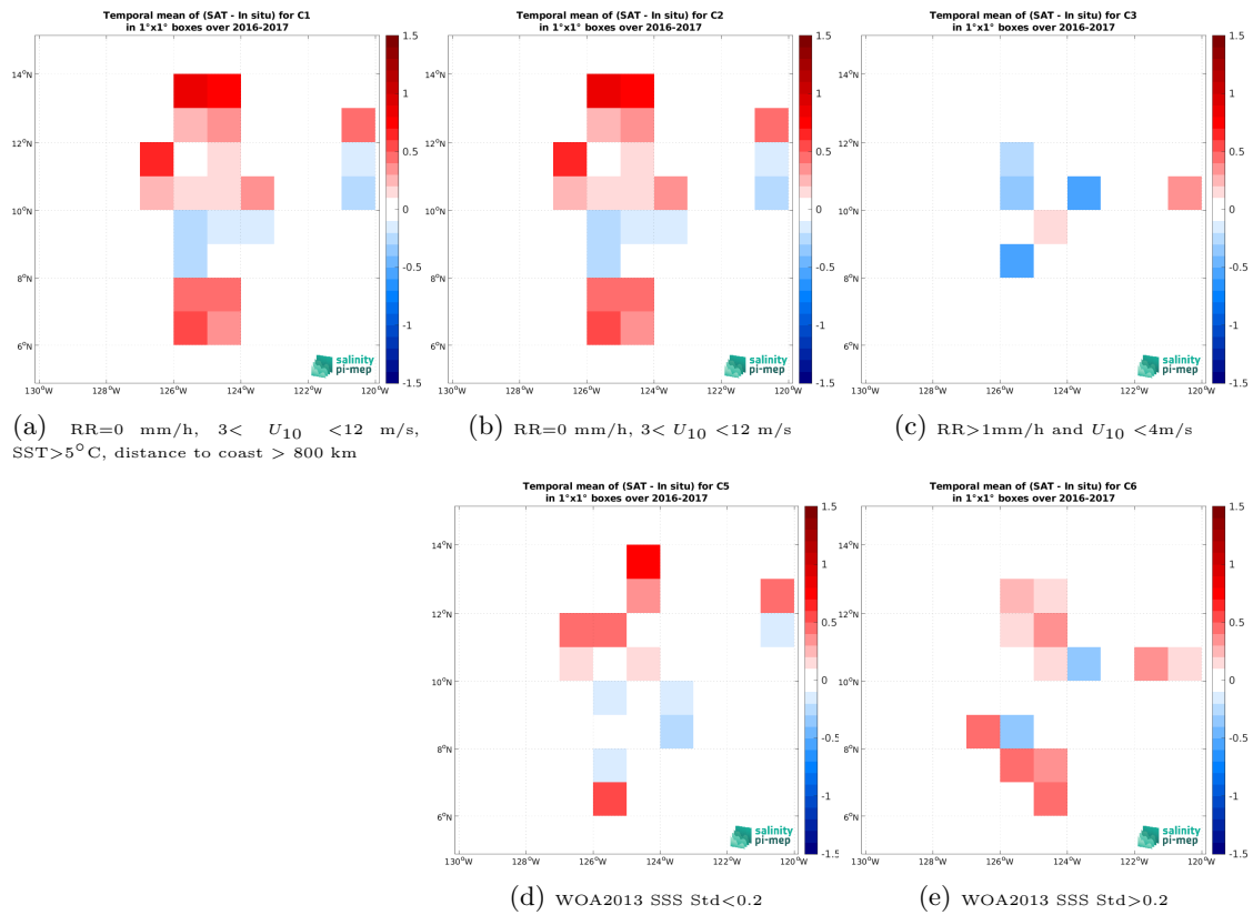
Figure 12: Temporal mean gridded over spatial boxes of size 1^\circ \times 1^\circ of \Delta\text{SSS} (SMAP SSS L2 v5.0 (JPL) - Salinity Snake (SPURS 2)) for 5 different subdatasets corresponding to: RR=0 mm/h, 3 < U_{10} < 12 m/s, SST > 5°C, distance to coast > 800 km (a), RR=0 mm/h, 3 < U_{10} < 12 m/s (b), RR > 1mm/h and U_{10} < 4 m/s (c), WOA2013 SSS Std < 0.2 (d), WOA2013 SSS Std > 0.2 (e).
