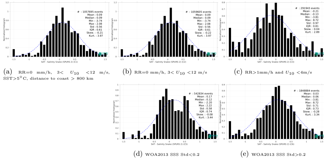
Figure 13: Normalized histogram of \Delta SSS (SMAP SSS L2 v5.0 (JPL) - Salinity Snake (SPURS 2)) for 5 different subdatasets corresponding to: RR=0 mm/h, 3 < U_{10} < 12 m/s, SST>5°C, distance to coast > 800 km (a), RR=0 mm/h, 3 < U_{10} < 12 m/s (b), RR>1mm/h and U_{10} < 4 m/s (c), WOA2013 SSS Std<0.2 (d), WOA2013 SSS Std>0.2 (e).
