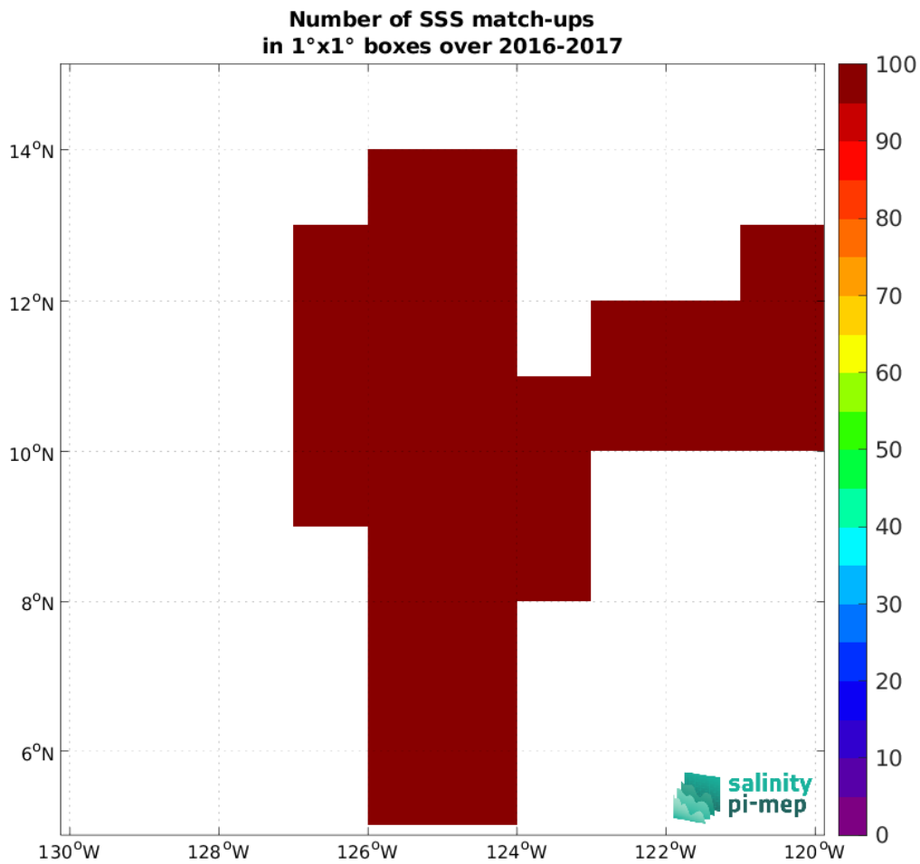
Figure 4: Number of SSS match-ups between Salinity Snake (SPURS 2) SSS and the SMAP SSS L2 v5.0 (JPL) SSS product for the SPURS 2 Pi-MEP region over 1^\circ \times 1^\circ boxes and for the full satellite product period.
