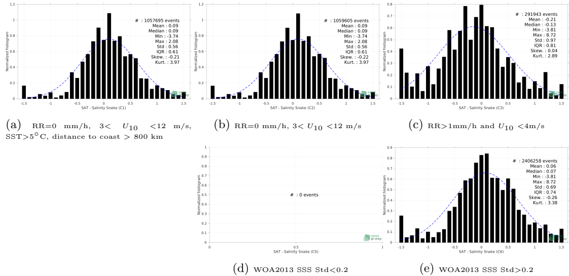
Figure 13: Normalized histogram of \Delta SSS (SMAP SSS L2 v5.0 (JPL) - Salinity Snake) for 5 different subdatasets corresponding to: RR=0 mm/h, 3 < U_{10} < 12 m/s, SST > 5°C, distance to coast > 800 km (a), RR=0 mm/h, 3 < U_{10} < 12 m/s (b), RR > 1mm/h and U_{10} < 4 m/s (c), WOA2013 SSS Std < 0.2 (d), WOA2013 SSS Std > 0.2 (e).
