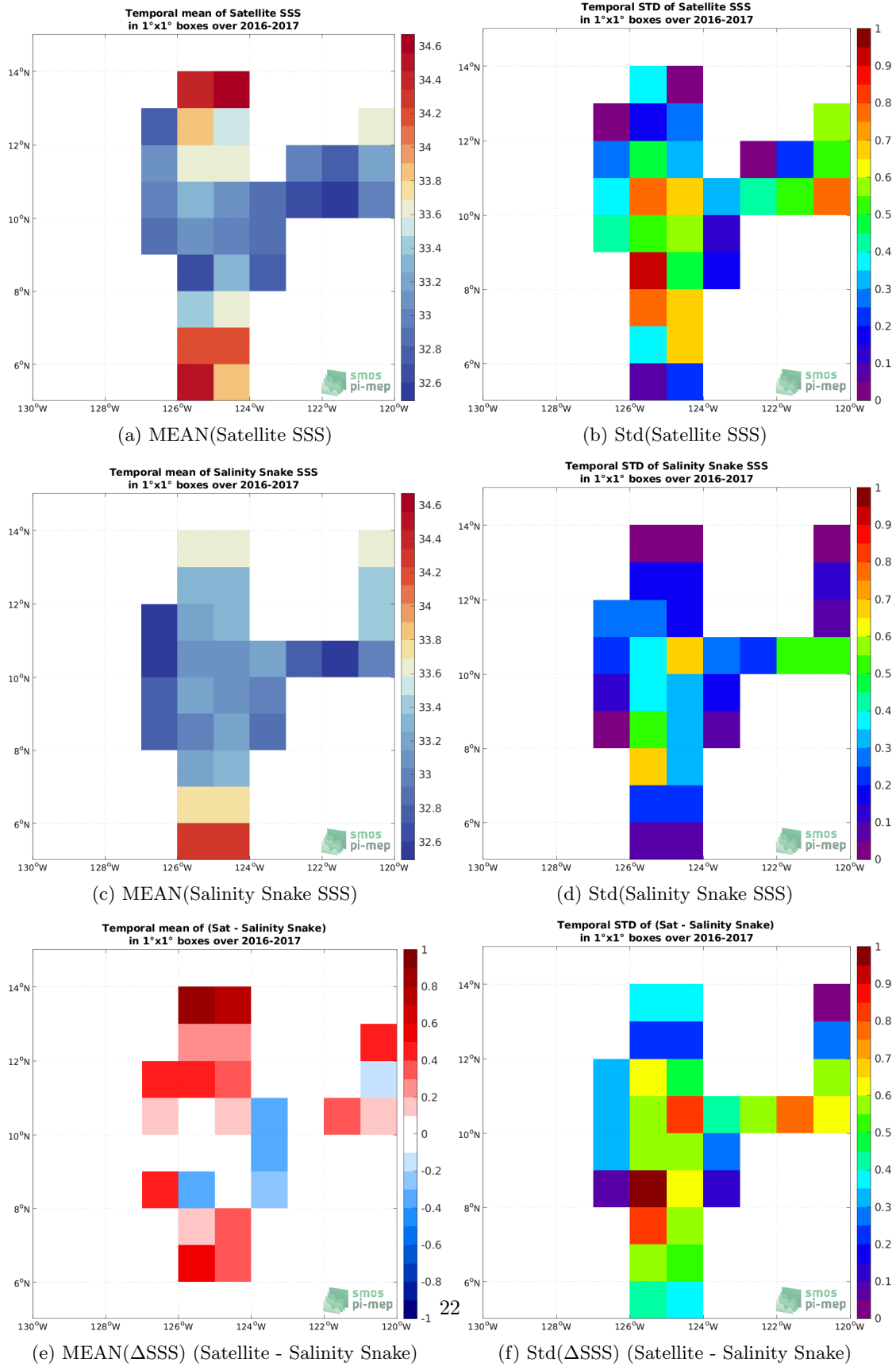
Figure 6: Temporal mean (left) and Std (right) of SSS from SMAP SSS L2 v5.0 (JPL) (top), Salinity Snake (middle), and of \Delta SSS (Satellite - Salinity Snake). Only match-up pairs are used to generate these maps.
