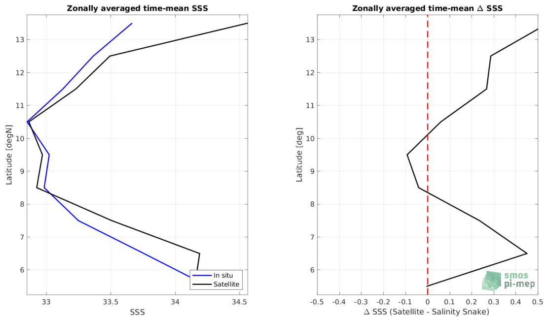
Figure 8: Left panel: Zonal mean SSS from SMAP SSS L2 v5.0 (JPL) satellite product (black) and from Salinity Snake (blue). Right panel: Zonal mean of \Delta SSS (Satellite - Salinity Snake) for all the collected Pi-MEP match-up pairs estimated over the full satellite product period.
