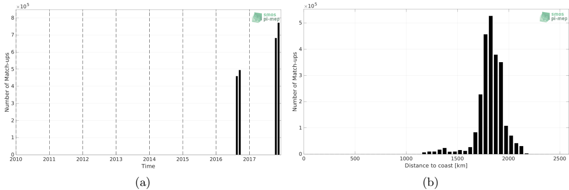
Figure 1: Number of match-ups between Salinity Snake and SMAP SSS L2 v5.0 (JPL) SSS as a function of time (a) and as function of the distance to coast (b) over the SPURS 2 Pi-MEP region and for the full satellite product period.
