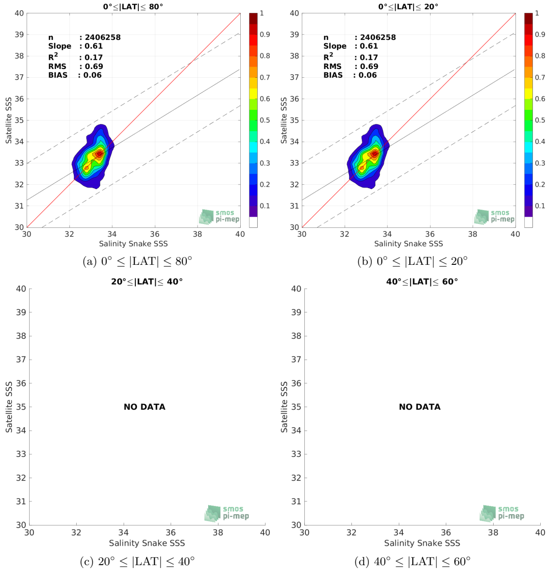
Figure 9: Contour maps of the concentration of SMAP SSS L2 v5.0 (JPL) SSS (y-axis) versus Salinity Snake SSS (x-axis) at match-up pairs for different latitude bands. For each plot, the red line shows x=y . The black thin and dashed lines indicate a linear fit through the data cloud and the \pm 95\% confidence levels, respectively. The number match-up pairs n , the slope and R^2 coefficient of the linear fit, the root mean square (RMS) and the mean bias between satellite and in situ data are indicated for each latitude band in each plots.
