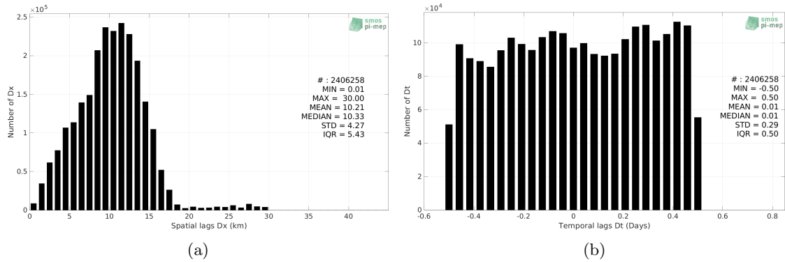
Figure 5: Histograms of the spatial (a) and temporal (b) lags between the location/time of the Salinity Snake measurement and the date of the corresponding SMAP SSS L2 v5.0 (JPL) SSS pixel.
