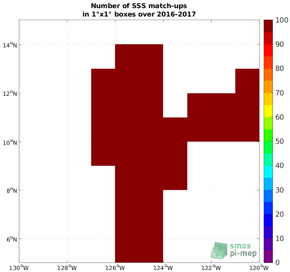
Figure 4: Number of SSS match-ups between Salinity Snake SSS and the SMAP SSS L2 v5.0 (JPL) SSS product for the SPURS 2 Pi-MEP region over 1°x1° boxes and for the full satellite product period.
