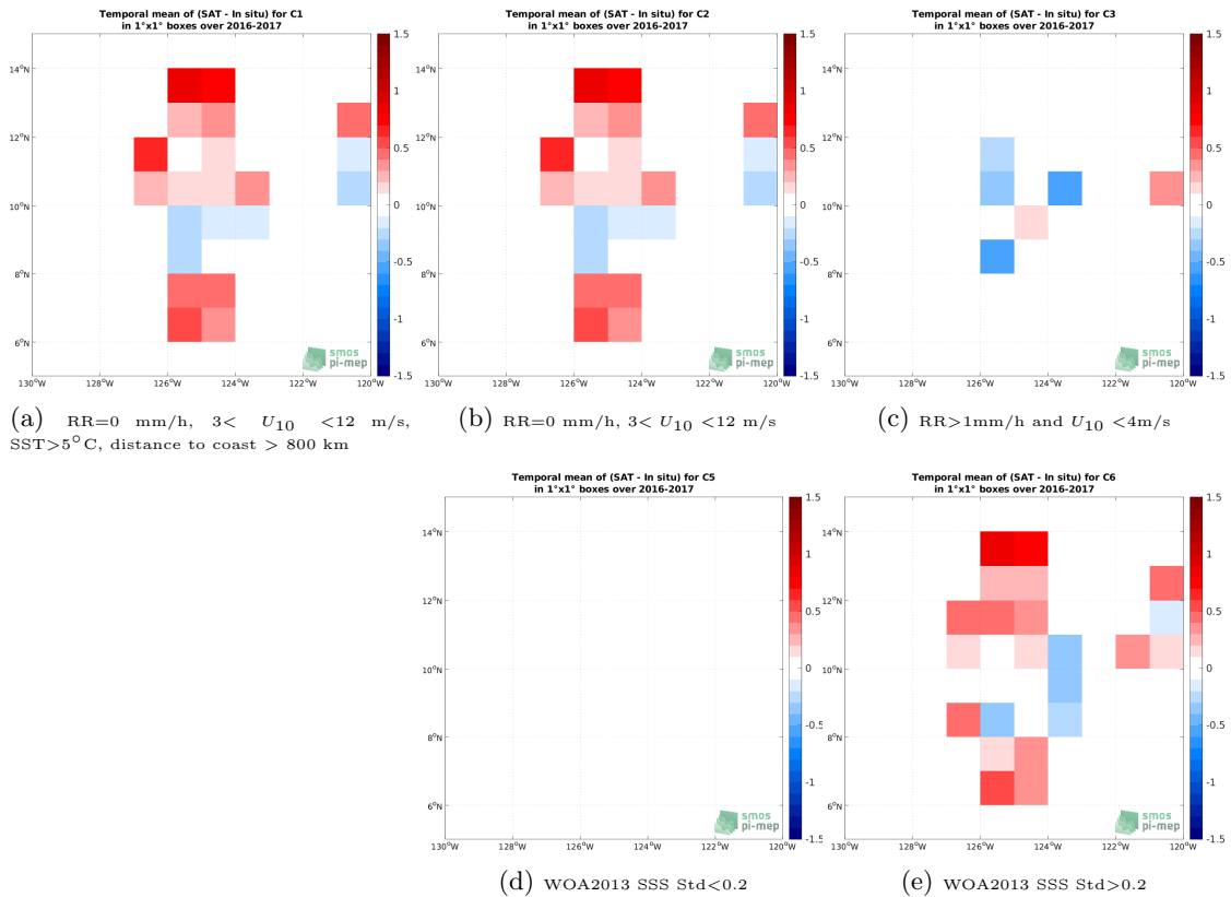
Figure 12: Temporal mean gridded over spatial boxes of size 1^\circ \times 1^\circ of \Delta SSS (SMAP SSS L2 v5.0 (JPL) - Salinity Snake) for 5 different subdatasets corresponding to:RR=0 mm/h, 3 < U_{10} < 12 m/s, SST >5^\circ C, distance to coast > 800 km (a), RR=0 mm/h, 3 < U_{10} < 12 m/s (b), RR >1 mm/h and U_{10} < 4 m/s (c), WOA2013 SSS Std <0.2 (d), WOA2013 SSS Std >0.2 (e).
