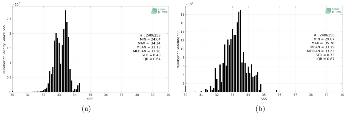
Figure 2: Histograms of SSS from Salinity Snake (a) and SMAP SSS L2 v5.0 (JPL) (b) considering all match-up pairs per bins of 0.1 over the SPURS 2 Pi-MEP region and for the full satellite product period.
