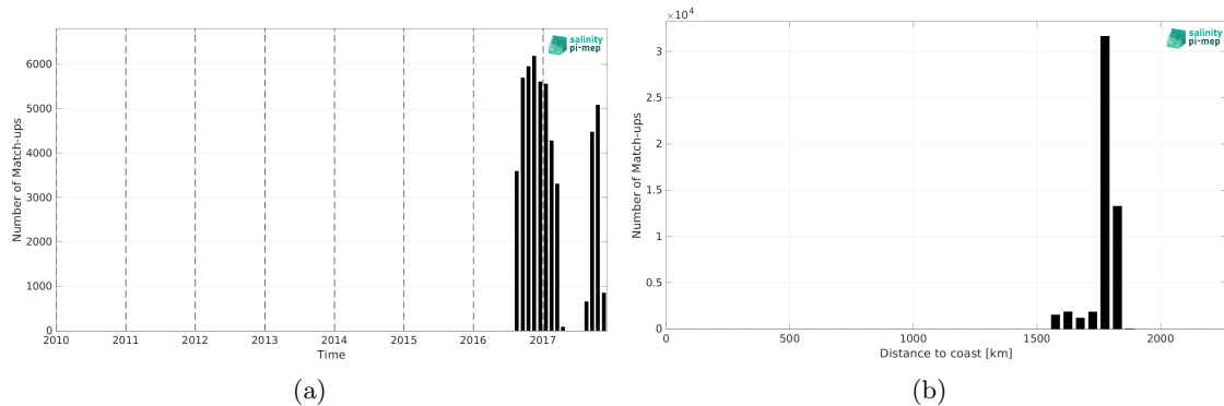
Figure 2: Number of match-ups between Seaglider (SPURS 2) and SMAP SSS L2 v5.0 (JPL) SSS as a function of time (a) and as function of the distance to coast (b) over the SPURS 2 Pi-MEP region and for the full satellite product period.
