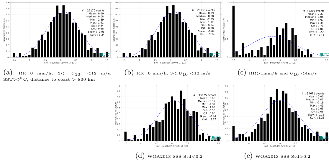
Figure 15: Normalized histogram of \Delta SSS (SMAP SSS L2 v5.0 (JPL) - Seaglider (SPURS 2)) for 5 different subdatasets corresponding to: RR=0 mm/h, 3 < U_{10} < 12 m/s, SST>5°C, distance to coast > 800 km (a), RR=0 mm/h, 3 < U_{10} < 12 m/s (b), RR>1mm/h and U_{10} < 4 m/s (c), WOA2013 SSS Std<0.2 (d), WOA2013 SSS Std>0.2 (e).
