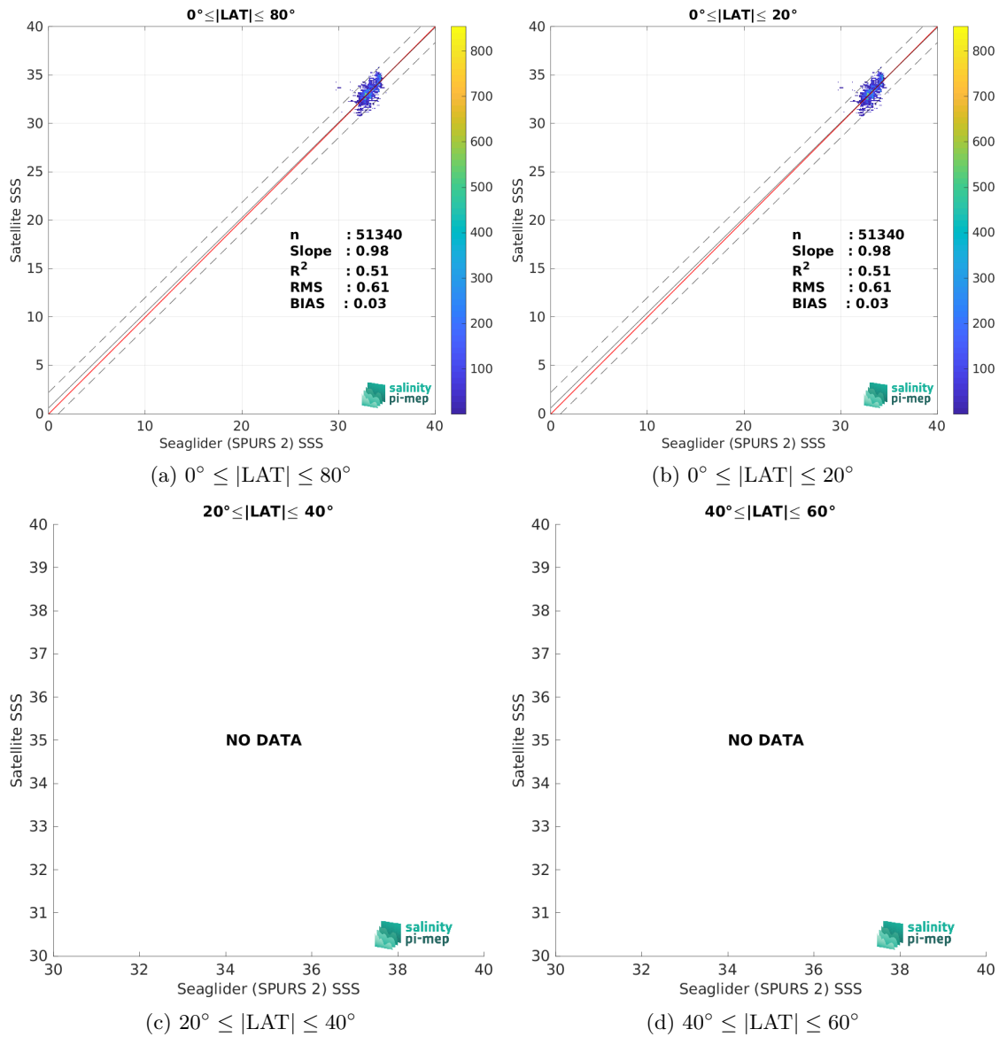
Figure 10: Contour maps of the concentration of SMAP SSS L2 v5.0 (JPL) SSS (y-axis) versus Seaglider (SPURS 2) SSS (x-axis) at match-up pairs for different latitude bands. For each plot, the red line shows x=y . The black thin and dashed lines indicate a linear fit through the data cloud and the \pm 95\% confidence levels, respectively. The number match-up pairs n , the slope and R^2 coefficient of the linear fit, the root mean square (RMS) and the mean bias between satellite and in situ data are indicated for each latitude band in each plots.
