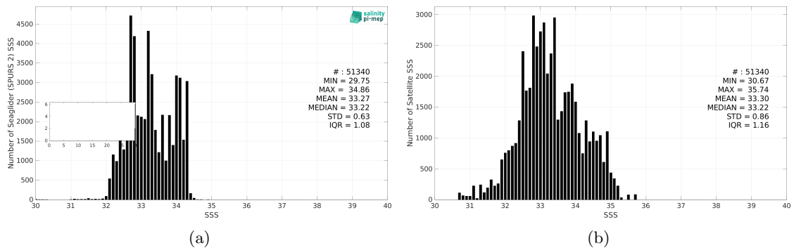
Figure 3: Histograms of SSS from Seaglider (SPURS 2) (a) and SMAP SSS L2 v5.0 (JPL) (b) considering all match-up pairs per bins of 0.1 over the SPURS 2 Pi-MEP region and for the full satellite product period.
