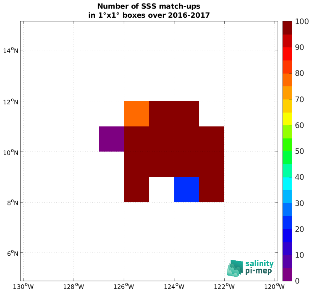
Figure 5: Number of SSS match-ups between Seaglider (SPURS 2) SSS and the SMAP SSS L2 v5.0 (JPL) SSS product for the SPURS 2 Pi-MEP region over 1^\circ \times 1^\circ boxes and for the full satellite product period.
