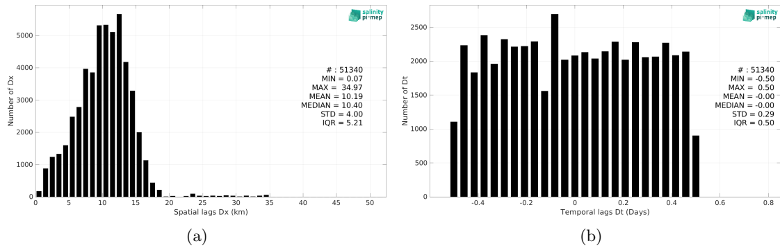
Figure 6: Histograms of the spatial (a) and temporal (b) lags between the location/time of the Seaglider (SPURS 2) measurement and the date of the corresponding SMAP SSS L2 v5.0 (JPL) SSS pixel.
