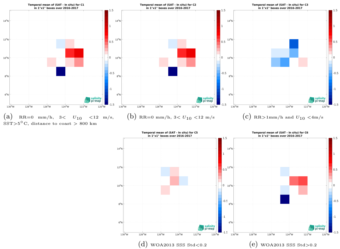
Figure 14: Temporal mean gridded over spatial boxes of size 1^\circ \times 1^\circ of \Delta SSS (SMAP SSS L2 v5.0 (JPL) - Seaglider (SPURS 2)) for 5 different subdatasets corresponding to:RR=0 mm/h, 3 < U_{10} < 12 m/s, SST >5^\circ C, distance to coast > 800 km (a), RR=0 mm/h, 3 < U_{10} < 12 m/s (b), RR >1 mm/h and U_{10} < 4 m/s (c), WOA2013 SSS Std <0.2 (d), WOA2013 SSS Std >0.2 (e).
