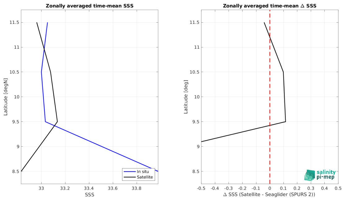
Figure 9: Left panel: Zonal mean SSS from SMAP SSS L2 v5.0 (JPL) satellite product (black) and from Seaglider (SPURS 2) (blue). Right panel: Zonal mean of \Delta SSS (Satellite - Seaglider (SPURS 2)) for all the collected Pi-MEP match-up pairs estimated over the full satellite product period.
