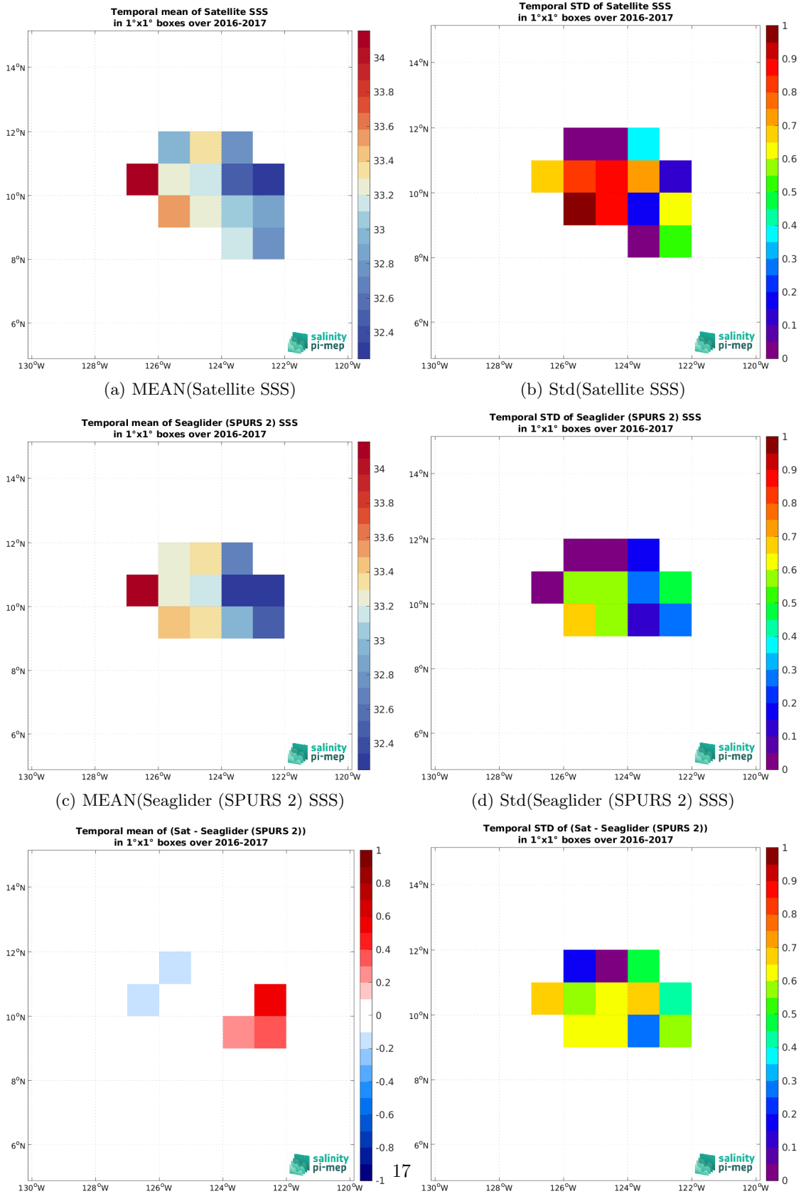
(e) MEAN( \Delta SSS) (Satellite - Seaglider (SPURS 2)) (f) Std( \Delta SSS) (Satellite - Seaglider (SPURS 2)) Figure 7: Temporal mean (left) and Std (right) of SSS from SMAP SSS L2 v5.0 (JPL) (top), Seaglider (SPURS 2) (middle), and of \Delta SSS (Satellite - Seaglider (SPURS 2)). Only match-up pairs are used to generate these maps.
