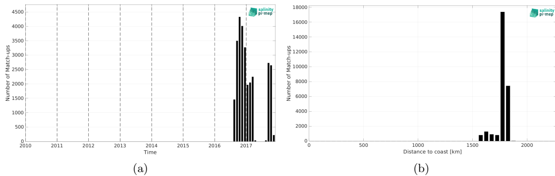
Figure 2: Number of match-ups between Seaglider (SPURS 2) and SMAP SSS L2 v5.0 (JPL) SSS as a function of time (a) and as function of the distance to coast (b) over the SPURS 2 Pi-MEP region and for the full satellite product period.
