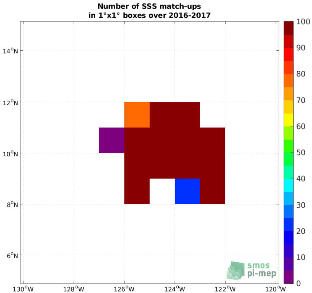
Figure 4: Number of SSS match-ups between Seaglider (SPURS 2) SSS and the SMAP SSS L2 v5.0 (JPL) SSS product for the SPURS 2 Pi-MEP region over 1°x1° boxes and for the full satellite product period.
