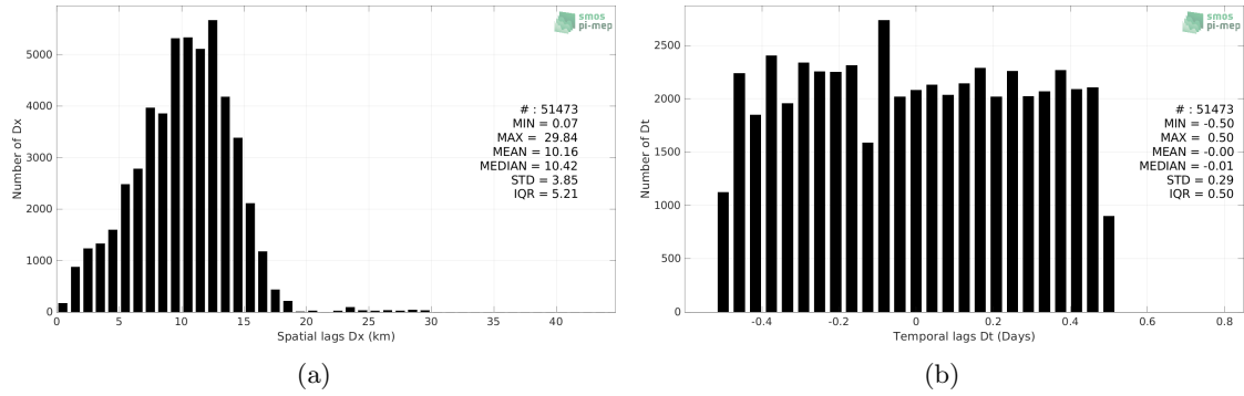
Figure 5: Histograms of the spatial (a) and temporal (b) lags between the location/time of the Seaglider measurement and the date of the corresponding SMAP SSS L2 v5.0 (JPL) SSS pixel.
