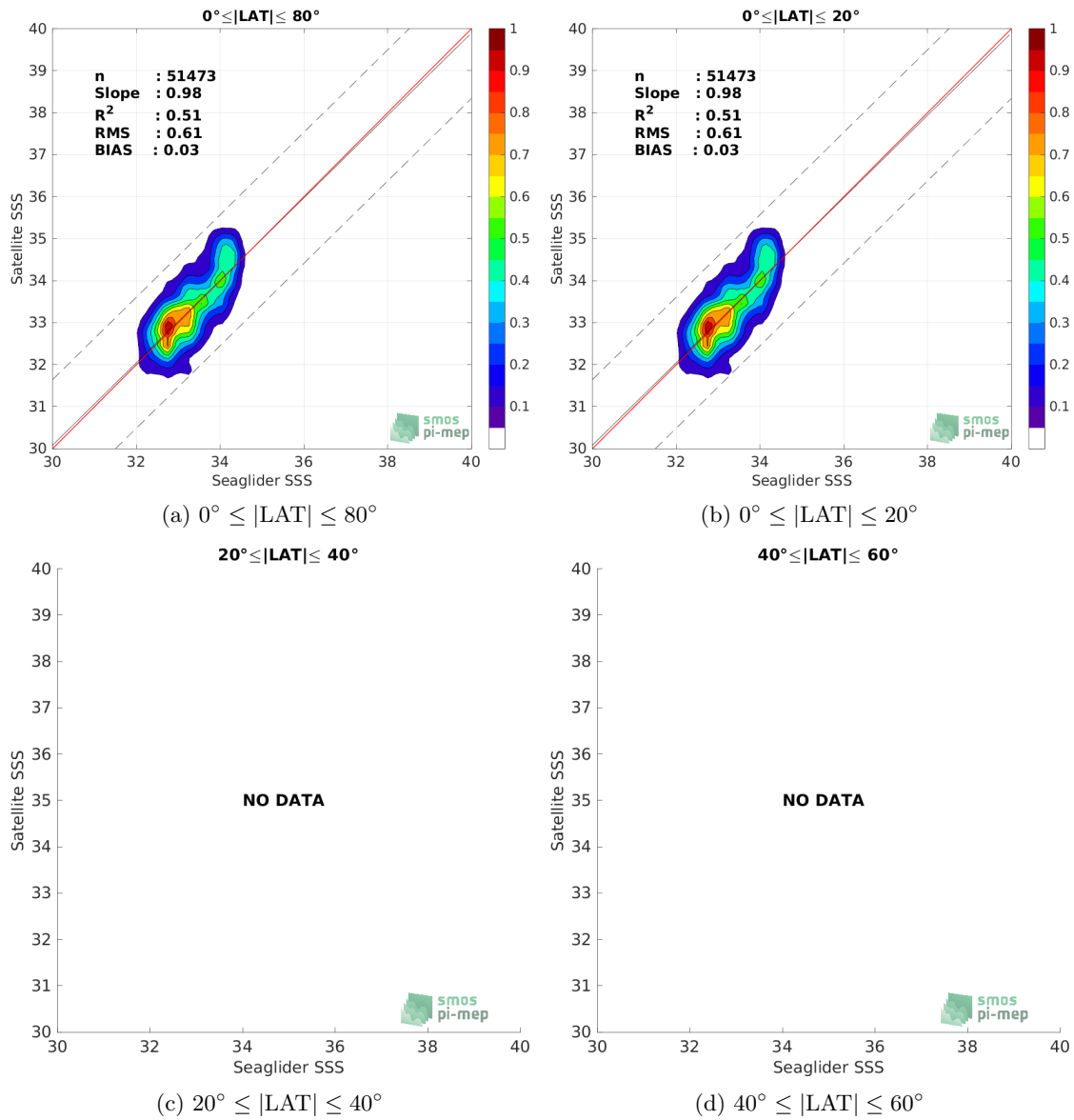
Figure 9: Contour maps of the concentration of SMAP SSS L2 v5.0 (JPL) SSS (y-axis) versus Seaglider SSS (x-axis) at match-up pairs for different latitude bands. For each plot, the red line shows x=y . The black thin and dashed lines indicate a linear fit through the data cloud and the \pm 95\% confidence levels, respectively. The number match-up pairs n , the slope and R^2 coefficient of the linear fit, the root mean square (RMS) and the mean bias between satellite and in situ data are indicated for each latitude band in each plots.
