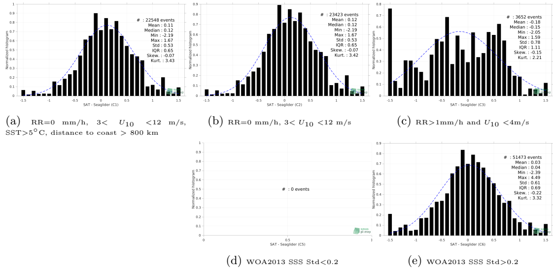
Figure 13: Normalized histogram of \Delta SSS (SMAP SSS L2 v5.0 (JPL) - Seaglider) for 5 different subdatasets corresponding to: RR=0 mm/h, 3 < U_{10} < 12 m/s, SST>5°C, distance to coast > 800 km (a), RR=0 mm/h, 3 < U_{10} < 12 m/s (b), RR>1mm/h and U_{10} < 4 m/s (c), WOA2013 SSS Std<0.2 (d), WOA2013 SSS Std>0.2 (e).
