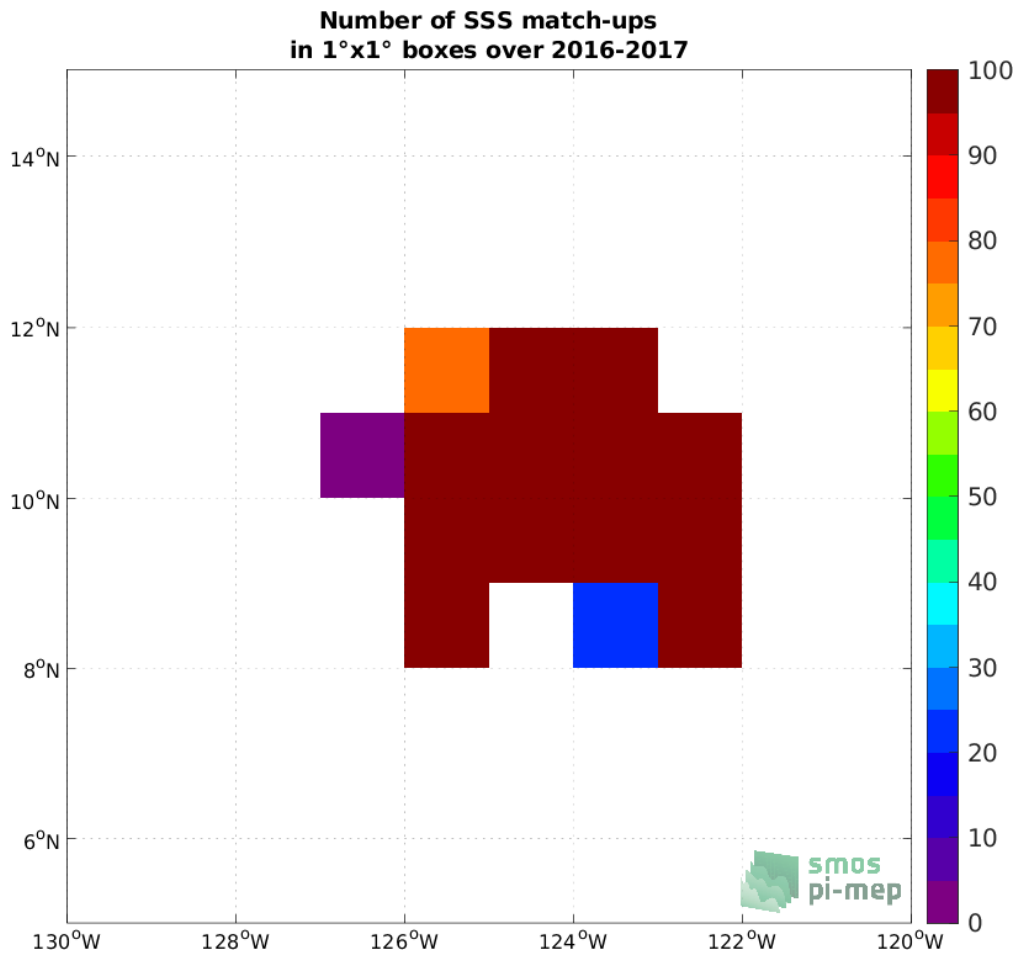
Figure 4: Number of SSS match-ups between Seaglider SSS and the SMAP SSS L2 v5.0 (JPL) SSS product for the SPURS 2 Pi-MEP region over 1°x1° boxes and for the full satellite product period.
