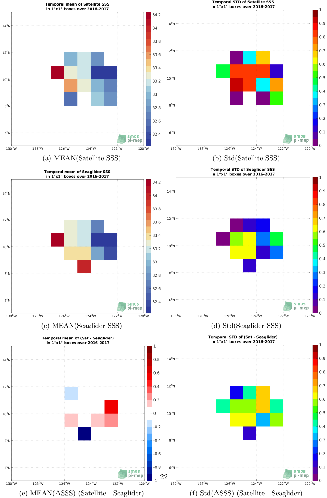
Figure 6: Temporal mean (left) and Std (right) of SSS from SMAP SSS L2 v5.0 (JPL) (top), Seaglider (middle), and of \Delta SSS (Satellite - Seaglider). Only match-up pairs are used to generate these maps.
