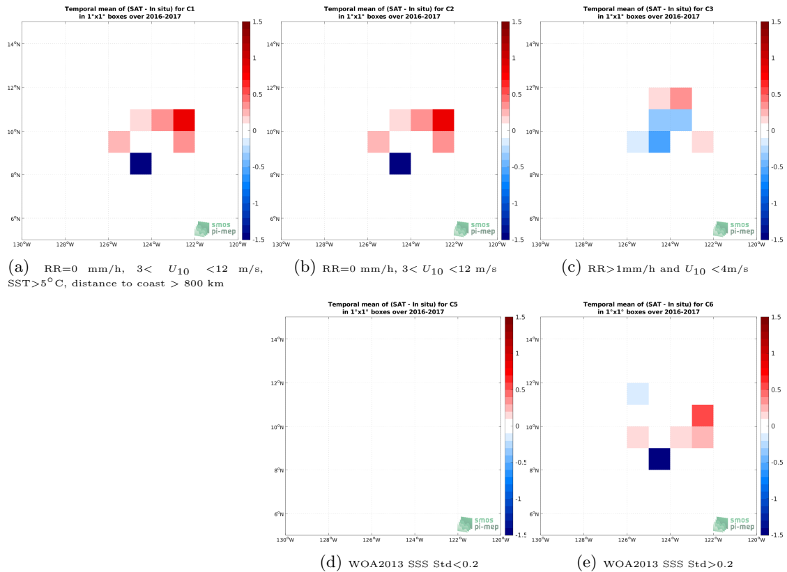
Figure 12: Temporal mean gridded over spatial boxes of size 1^\circ \times 1^\circ of \Delta SSS (SMAP SSS L2 v5.0 (JPL) - Seaglider) for 5 different subdatasets corresponding to: RR=0 mm/h, 3 < U_{10} < 12 m/s, SST > 5^\circ\text{C} , distance to coast > 800 km (a), RR=0 mm/h, 3 < U_{10} < 12 m/s (b), RR > 1 mm/h and U_{10} < 4 m/s (c), WOA2013 SSS Std < 0.2 (d), WOA2013 SSS Std > 0.2 (e).
