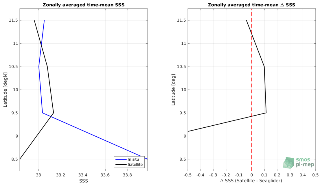
Figure 8: Left panel: Zonal mean SSS from SMAP SSS L2 v5.0 (JPL) satellite product (black) and from Seaglider (blue). Right panel: Zonal mean of \Delta SSS (Satellite - Seaglider) for all the collected Pi-MEP match-up pairs estimated over the full satellite product period.
