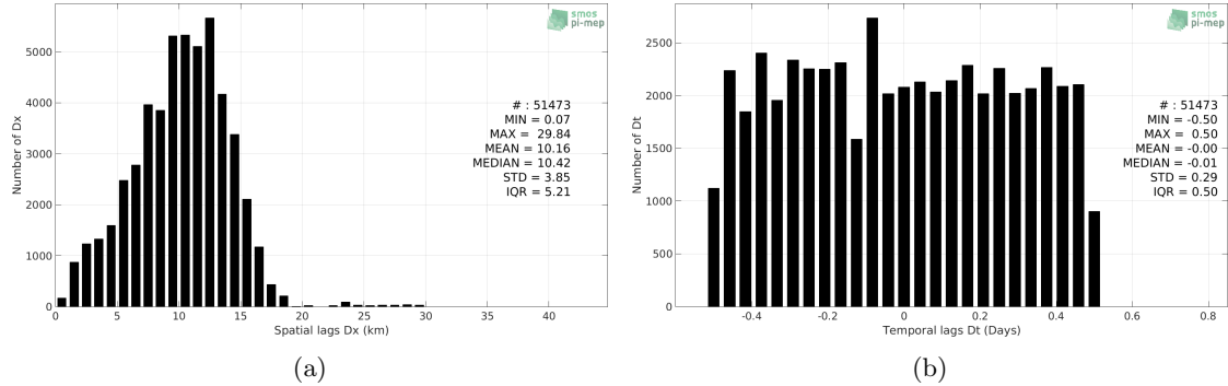
Figure 5: Histograms of the spatial (a) and temporal (b) lags between the time of the Seaglider measurements and the date of the corresponding SMAP SSS L2 v5.0 (JPL) SSS product.
