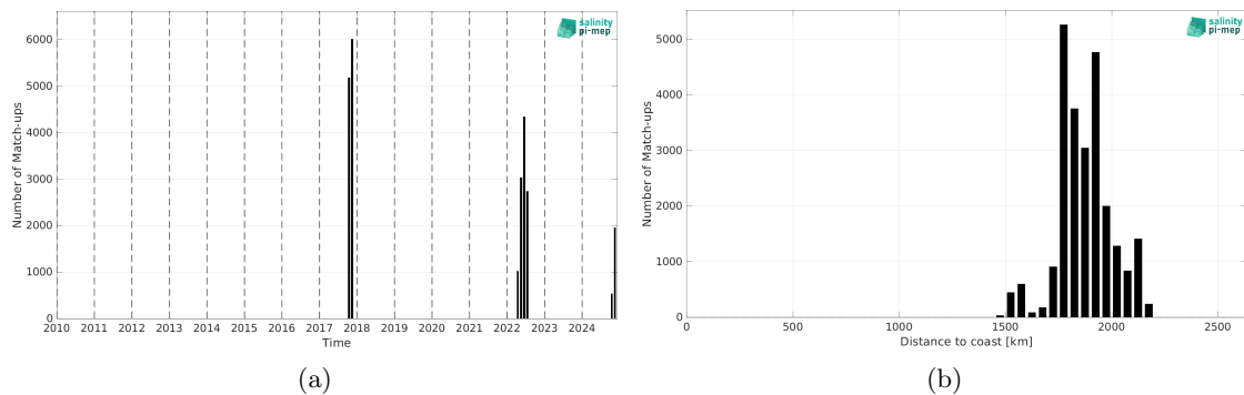
Figure 2: Number of match-ups between Saildrone and SMAP SSS L2 v5.0 (JPL) SSS as a function of time (a) and as function of the distance to coast (b) over the SPURS 2 Pi-MEP region and for the full satellite product period.
