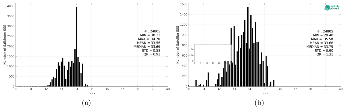
Figure 3: Histograms of SSS from Saildrone (a) and SMAP SSS L2 v5.0 (JPL) (b) considering all match-up pairs per bins of 0.1 over the SPURS 2 Pi-MEP region and for the full satellite product period.
