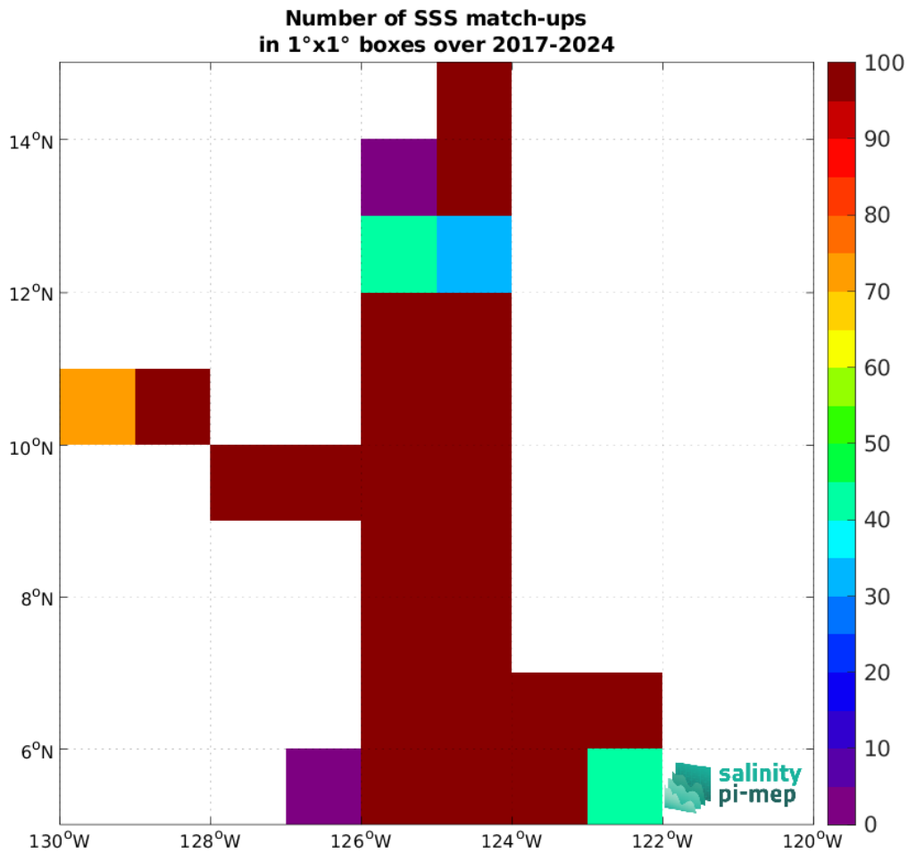
Figure 5: Number of SSS match-ups between Saildrone SSS and the SMAP SSS L2 v5.0 (JPL) SSS product for the SPURS 2 Pi-MEP region over 1°x1° boxes and for the full satellite product period.
