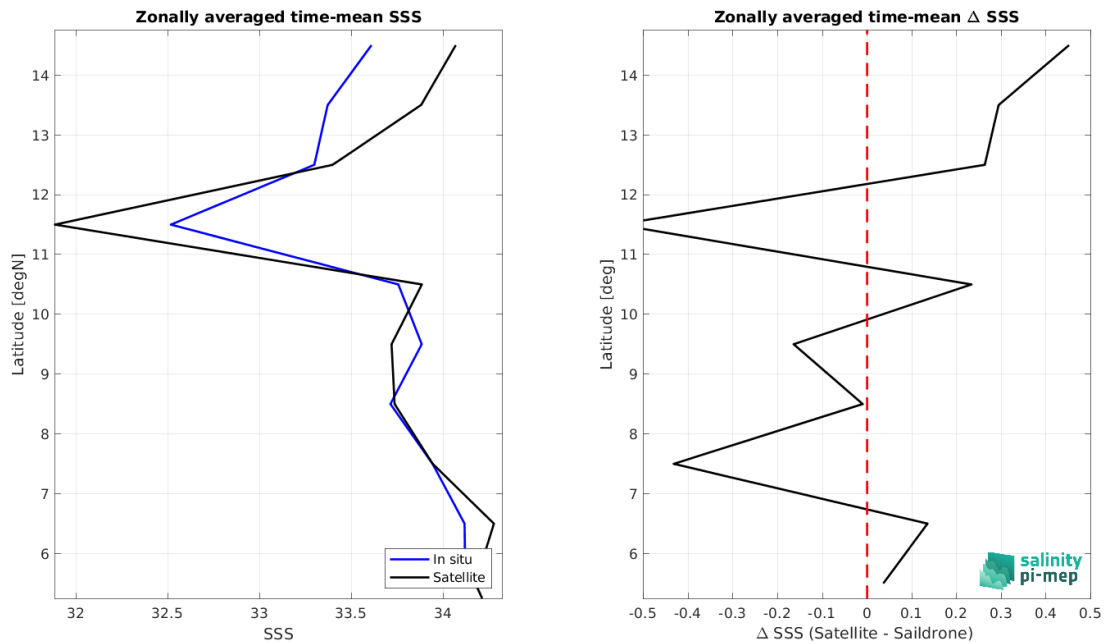
Figure 9: Left panel: Zonal mean SSS from SMAP SSS L2 v5.0 (JPL) satellite product (black) and from Sairdron (blue). Right panel: Zonal mean of \Delta SSS (Satellite - Sairdron) for all the collected Pi-MEP match-up pairs estimated over the full satellite product period.
