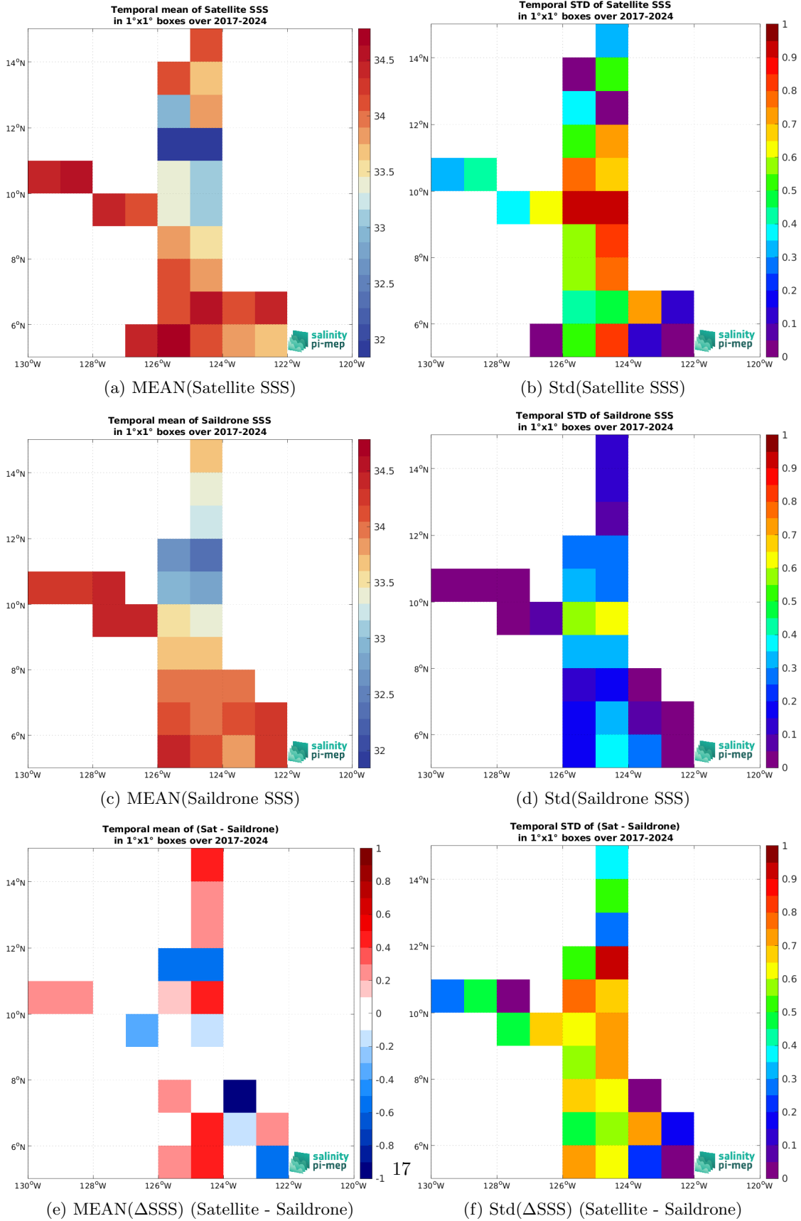
Figure 7: Temporal mean (left) and Std (right) of SSS from SMAP SSS L2 v5.0 (JPL) (top), Saildrone (middle), and of \Delta SSS (Satellite - Saildrone). Only match-up pairs are used to generate these maps.
