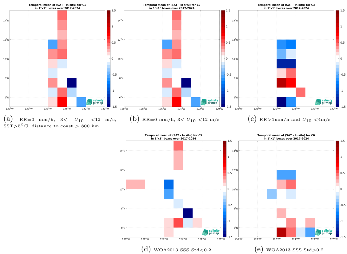
Figure 14: Temporal mean gridded over spatial boxes of size 1^\circ \times 1^\circ of \Delta\text{SSS} (SMAP SSS L2 v5.0 (JPL) - Saildrone) for 5 different subdatasets corresponding to: RR=0 mm/h, 3 < U_{10} < 12 m/s, SST > 5°C, distance to coast > 800 km (a), RR=0 mm/h, 3 < U_{10} < 12 m/s (b), RR > 1mm/h and U_{10} < 4 m/s (c), WOA2013 SSS Std < 0.2 (d), WOA2013 SSS Std > 0.2 (e).
