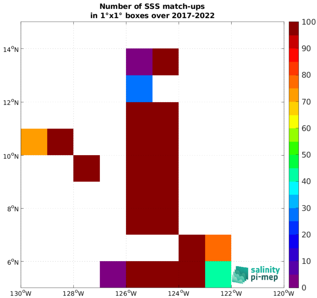
Figure 5: Number of SSS match-ups between Saildrone SSS and the SMAP SSS L2 v5.0 (JPL) SSS product for the SPURS 2 Pi-MEP region over 1°×1° boxes and for the full satellite product period.
