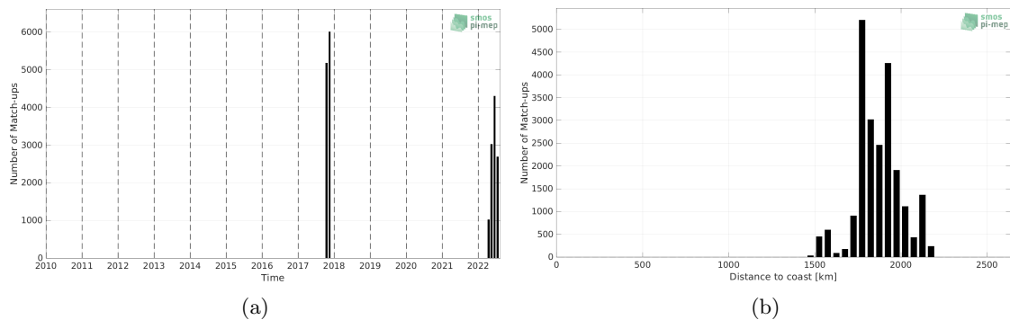
Figure 1: Number of match-ups between Sairdron and SMAP SSS L2 v5.0 (JPL) SSS as a function of time (a) and as function of the distance to coast (b) over the SPURS 2 Pi-MEP region and for the full satellite product period.
