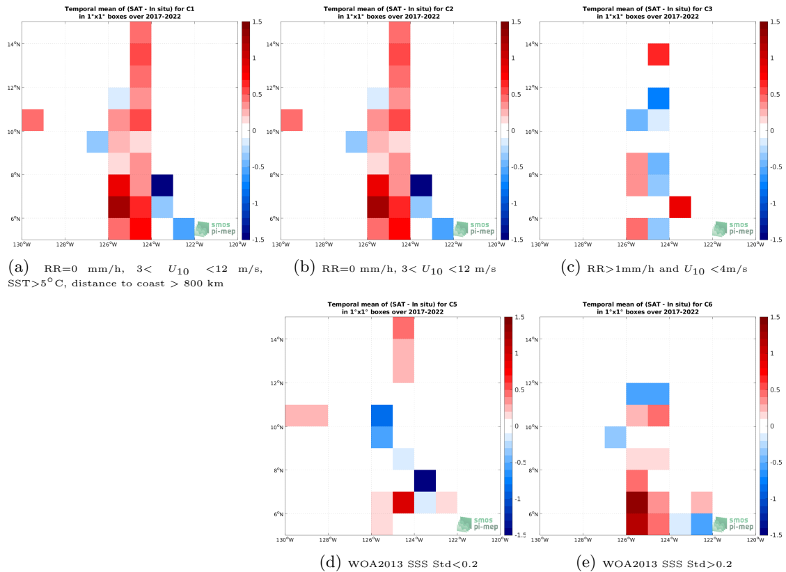
Figure 12: Temporal mean gridded over spatial boxes of size 1^\circ \times 1^\circ of \Delta SSS (SMAP SSS L2 v5.0 (JPL) - Saildrone) for 5 different subdatasets corresponding to:RR=0 mm/h, 3 < U_{10} < 12 m/s, SST >5^\circ C, distance to coast > 800 km (a), RR=0 mm/h, 3 < U_{10} < 12 m/s (b), RR >1 mm/h and U_{10} < 4 m/s (c), WOA2013 SSS Std <0.2 (d), WOA2013 SSS Std >0.2 (e).
