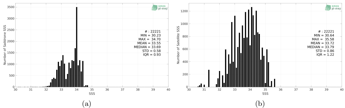
Figure 2: Histograms of SSS from Sairdron (a) and SMAP SSS L2 v5.0 (JPL) (b) considering all match-up pairs per bins of 0.1 over the SPURS 2 Pi-MEP region and for the full satellite product period.
