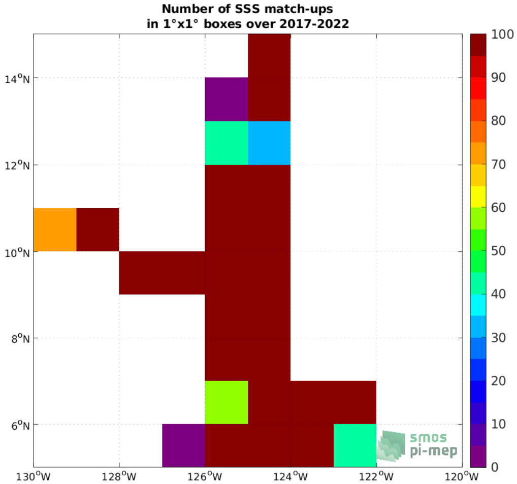
Figure 4: Number of SSS match-ups between Saildrone SSS and the SMAP SSS L2 v5.0 (JPL) SSS product for the SPURS 2 Pi-MEP region over 1°x1° boxes and for the full satellite product period.
