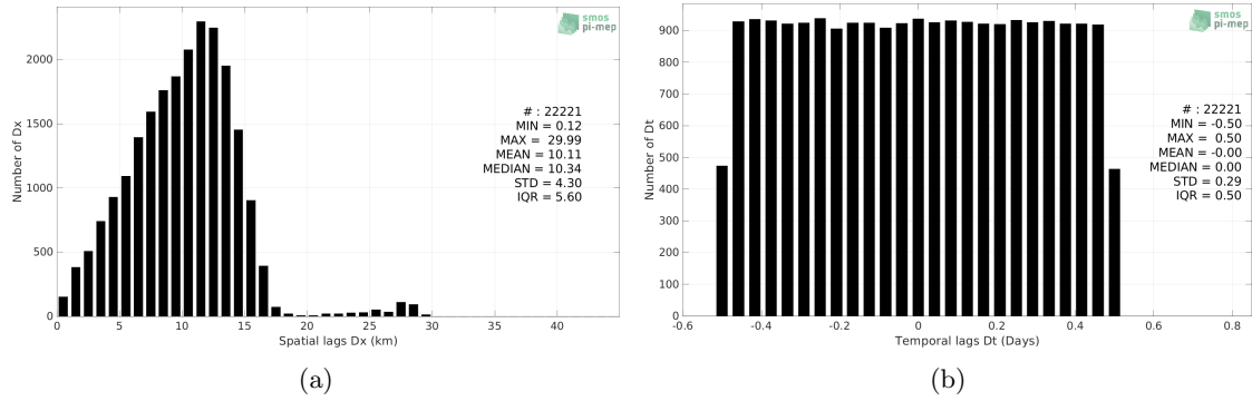
Figure 5: Histograms of the spatial (a) and temporal (b) lags between the location/time of the Sailldrone measurement and the date of the corresponding SMAP SSS L2 v5.0 (JPL) SSS pixel.
