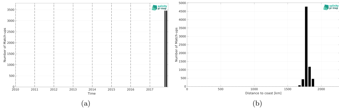
Figure 2: Number of match-ups between Saildrone (SPURS 2) and SMAP SSS L2 v5.0 (JPL) SSS as a function of time (a) and as function of the distance to coast (b) over the SPURS 2 Pi-MEP region and for the full satellite product period.
