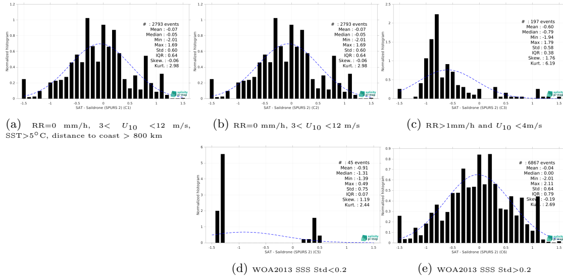
Figure 15: Normalized histogram of \Delta SSS (SMAP SSS L2 v5.0 (JPL) - Saildrone (SPURS 2)) for 5 different subdatasets corresponding to: RR=0 mm/h, 3 < U_{10} < 12 m/s, SST>5°C, distance to coast > 800 km (a), RR=0 mm/h, 3 < U_{10} < 12 m/s (b), RR>1mm/h and U_{10} < 4 m/s (c), WOA2013 SSS Std<0.2 (d), WOA2013 SSS Std>0.2 (e).
