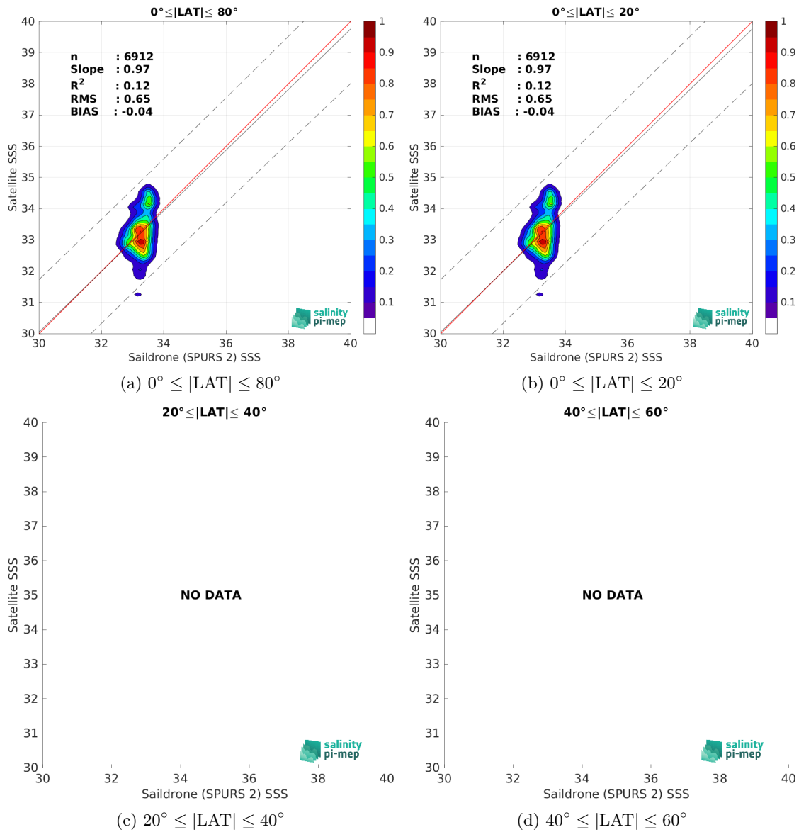
Figure 10: Contour maps of the concentration of SMAP SSS L2 v5.0 (JPL) SSS (y-axis) versus Saildrone (SPURS 2) SSS (x-axis) at match-up pairs for different latitude bands. For each plot, the red line shows x=y . The black thin and dashed lines indicate a linear fit through the data cloud and the \pm 95\% confidence levels, respectively. The number match-up pairs n , the slope and R^2 coefficient of the linear fit, the root mean square (RMS) and the mean bias between satellite and in situ data are indicated for each latitude band in each plots.
