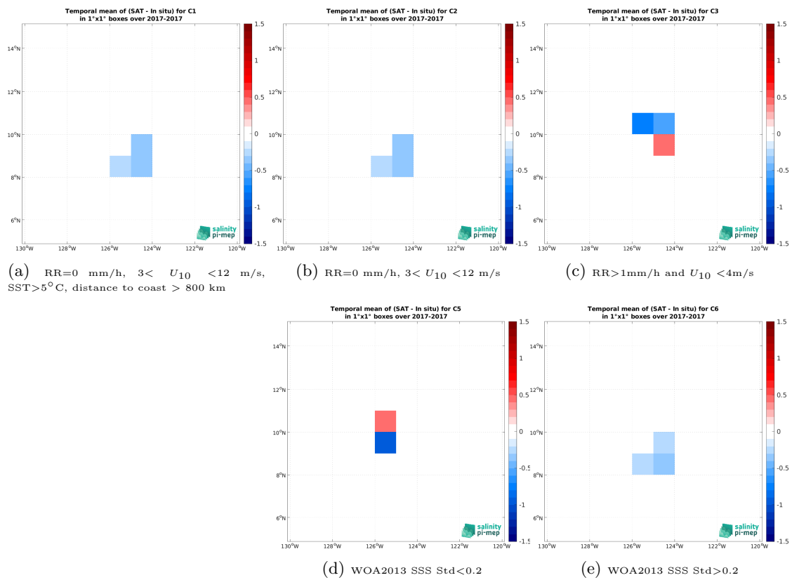
Figure 14: Temporal mean gridded over spatial boxes of size 1^\circ \times 1^\circ of \Delta SSS (SMAP SSS L2 v5.0 (JPL) - Saildrone (SPURS 2)) for 5 different subdatasets corresponding to:RR=0 mm/h, 3 < U_{10} < 12 m/s, SST>5°C, distance to coast > 800 km (a), RR=0 mm/h, 3 < U_{10} < 12 m/s (b), RR>1mm/h and U_{10} < 4 m/s (c), WOA2013 SSS Std<0.2 (d), WOA2013 SSS Std>0.2 (e).
