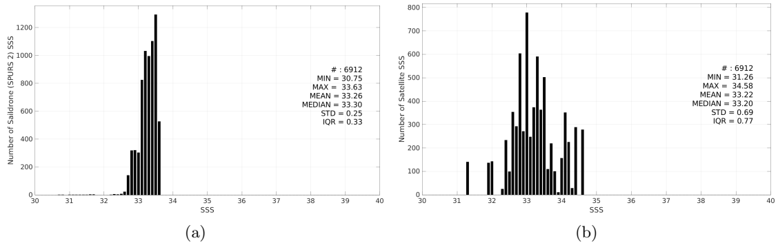
Figure 3: Histograms of SSS from Saildrone (SPURS 2) (a) and SMAP SSS L2 v5.0 (JPL) (b) considering all match-up pairs per bins of 0.1 over the SPURS 2 Pi-MEP region and for the full satellite product period.
