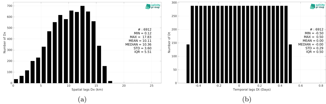
Figure 6: Histograms of the spatial (a) and temporal (b) lags between the location/time of the Saildrone (SPURS 2) measurement and the date of the corresponding SMAP SSS L2 v5.0 (JPL) SSS pixel.
