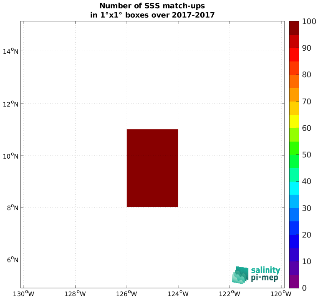
Figure 5: Number of SSS match-ups between Saildrone (SPURS 2) SSS and the SMAP SSS L2 v5.0 (JPL) SSS product for the SPURS 2 Pi-MEP region over 1^\circ \times 1^\circ boxes and for the full satellite product period.
