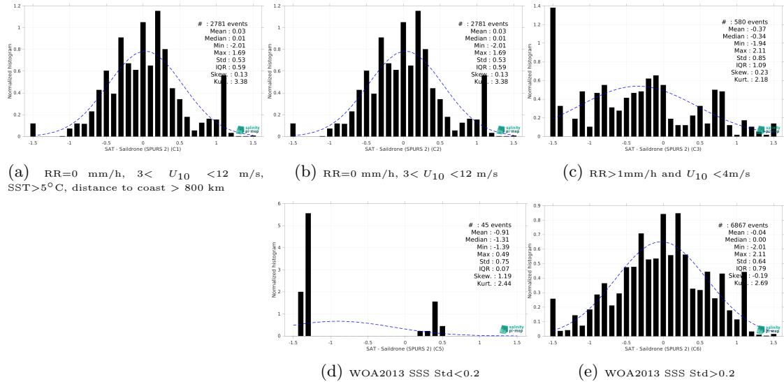
Figure 13: Normalized histogram of \Delta SSS (SMAP SSS L2 v5.0 (JPL) - Saildrome (SPURS 2)) for 5 different subdatasets corresponding to: RR=0 mm/h, 3 < U_{10} < 12 m/s, SST > 5°C, distance to coast > 800 km (a), RR=0 mm/h, 3 < U_{10} < 12 m/s (b), RR > 1mm/h and U_{10} < 4 m/s (c), WOA2013 SSS Std < 0.2 (d), WOA2013 SSS Std > 0.2 (e).
