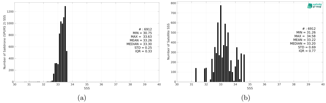
Figure 2: Histograms of SSS from Saildrone (SPURS 2) (a) and SMAP SSS L2 v5.0 (JPL) (b) considering all match-up pairs per bins of 0.1 over the SPURS 2 Pi-MEP region and for the full satellite product period.
