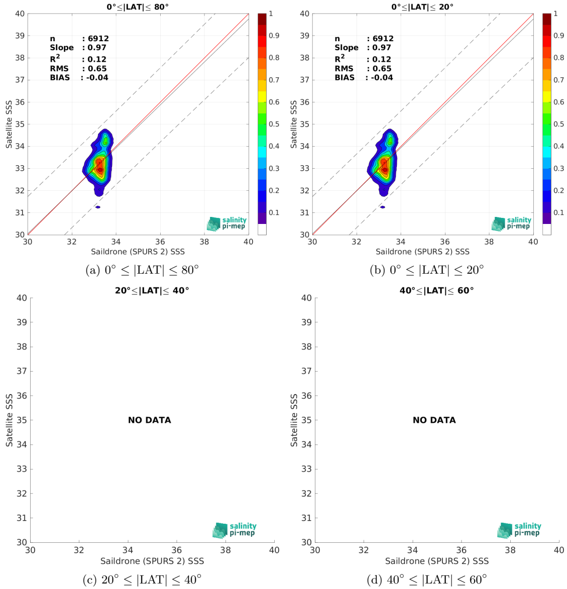
Figure 9: Contour maps of the concentration of SMAP SSS L2 v5.0 (JPL) SSS (y-axis) versus Saildrone (SPURS 2) SSS (x-axis) at match-up pairs for different latitude bands. For each plot, the red line shows x=y . The black thin and dashed lines indicate a linear fit through the data cloud and the \pm 95\% confidence levels, respectively. The number match-up pairs n , the slope and R^2 coefficient of the linear fit, the root mean square (RMS) and the mean bias between satellite and in situ data are indicated for each latitude band in each plots.
