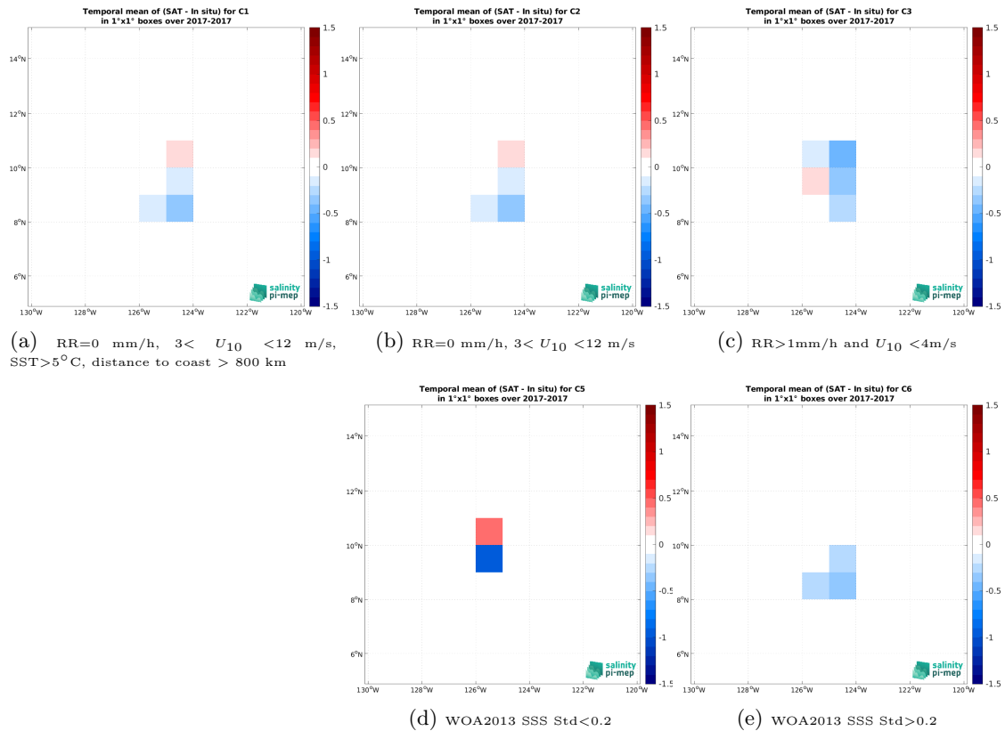
Figure 12: Temporal mean gridded over spatial boxes of size 1^\circ \times 1^\circ of \Delta SSS (SMAP SSS L2 v5.0 (JPL) - Saildrone (SPURS 2)) for 5 different subdatasets corresponding to:RR=0 mm/h, 3 < U_{10} < 12 m/s, SST >5^\circ\text{C} , distance to coast > 800 km (a), RR=0 mm/h, 3 < U_{10} < 12 m/s (b), RR >1 mm/h and U_{10} < 4 m/s (c), WOA2013 SSS Std <0.2 (d), WOA2013 SSS Std >0.2 (e).
