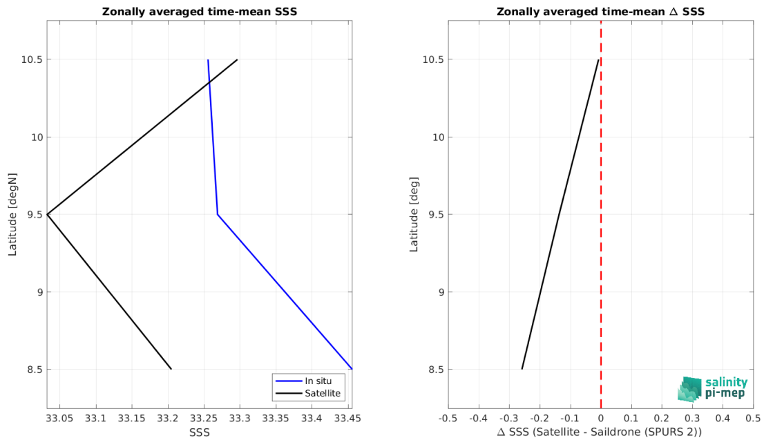
Figure 8: Left panel: Zonal mean SSS from SMAP SSS L2 v5.0 (JPL) satellite product (black) and from Sairdron (SPURS 2) (blue). Right panel: Zonal mean of \Delta SSS (Satellite - Sairdron (SPURS 2)) for all the collected Pi-MEP match-up pairs estimated over the full satellite product period.
