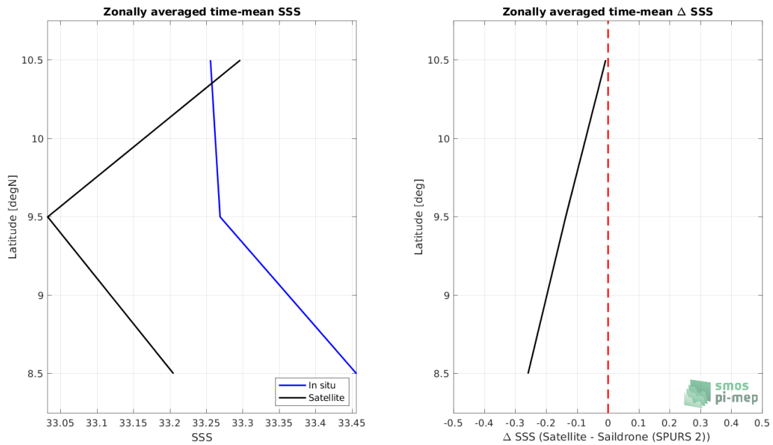
Figure 8: Left panel: Zonal mean SSS from SMAP SSS L2 v5.0 (JPL) satellite product (black) and from Sairdrone (SPURS 2) (blue). Right panel: Zonal mean of \Delta SSS (Satellite - Sairdrone (SPURS 2)) for all the collected Pi-MEP match-up pairs estimated over the full satellite product period.
