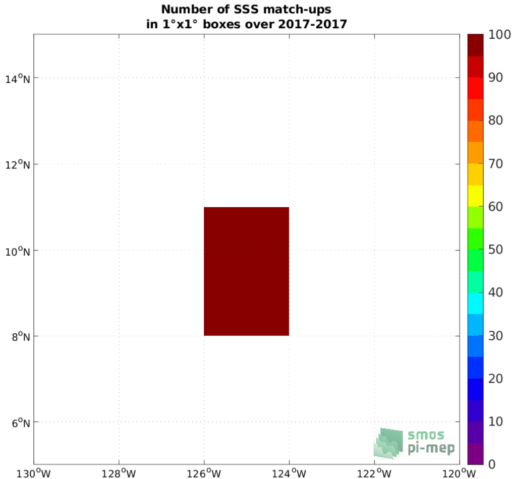
Figure 3: Number of SSS match-ups between Saildrone SSS and the SMAP SSS L2 v5.0 (JPL) SSS product for the SPURS 2 Pi-MEP region over 1^\circ \times 1^\circ boxes and for the full satellite product period.
