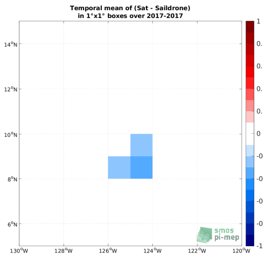
(e) MEAN( \Delta SSS) (Satellite - Saildrone)
