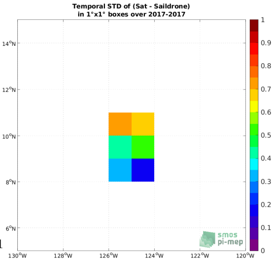
(f) Std( \Delta SSS) (Satellite - Saildrone)
