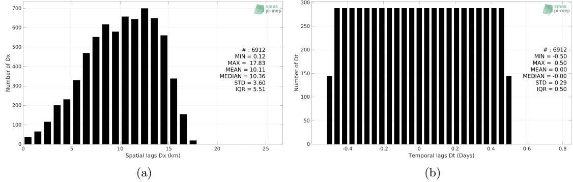
Figure 4: Histograms of the spatial (a) and temporal (b) lags between the location/time of the Sailldrone measurement and the date of the corresponding SMAP SSS L2 v5.0 (JPL) SSS pixel.
