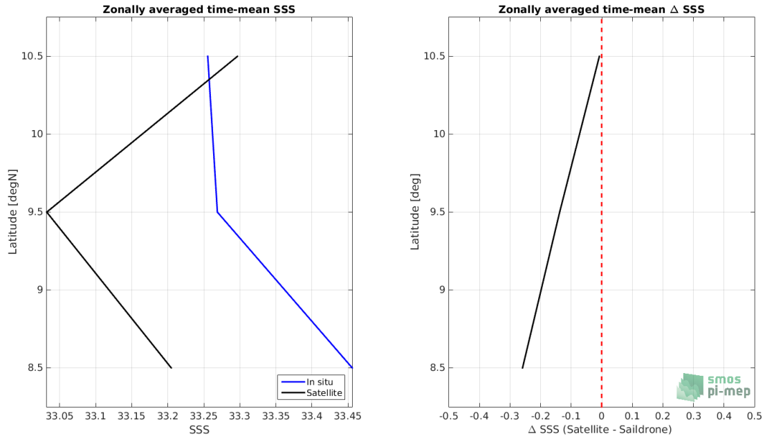
Figure 7: Left panel: Zonal mean SSS from SMAP SSS L2 v5.0 (JPL) satellite product (black) and from Saildrone (blue). Right panel: Zonal mean of \Delta SSS (Satellite - Saildrone) for all the collected Pi-MEP match-up pairs estimated over the full satellite product period.
