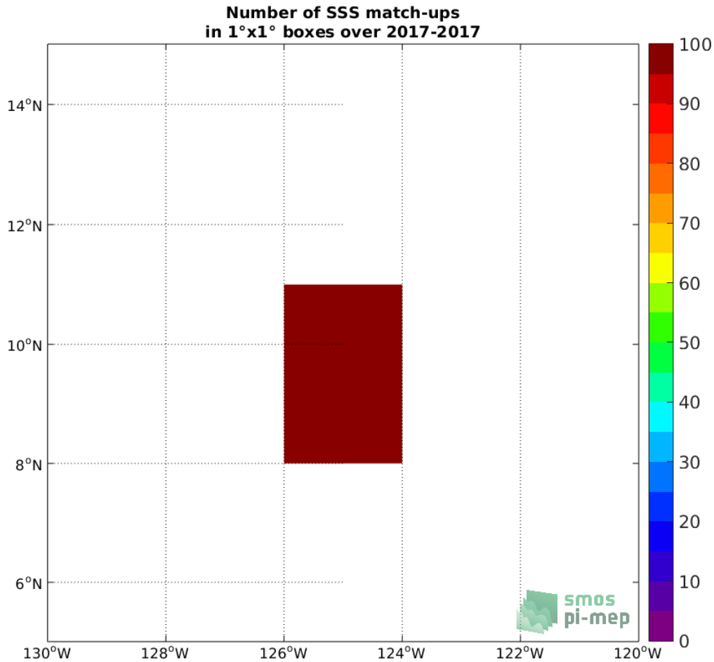
Figure 3: Number of SSS match-ups between Saildrone SSS and the SMAP SSS L2 v5.0 (JPL) SSS product for the SPURS 2 Pi-MEP region over 1^\circ \times 1^\circ boxes and for the full satellite product period.
