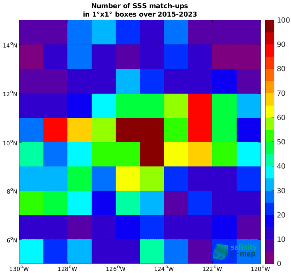
Figure 4: Number of SSS match-ups between Argo SSS and the SMAP SSS L2 v5.0 (JPL) SSS product for the SPURS 2 Pi-MEP region over 1°x1° boxes and for the full satellite product period.
