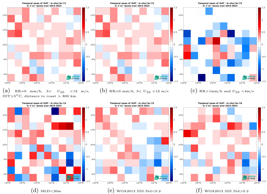
Figure 12: Temporal mean gridded over spatial boxes of size 1^\circ \times 1^\circ of \Delta SSS (SMAP SSS L2 v5.0 (JPL) - Argo) for 6 different subdatasets corresponding to:RR=0 mm/h, 3 < U_{10} < 12 m/s, SST >5^\circ C, distance to coast > 800 km (a), RR=0 mm/h, 3 < U_{10} < 12 m/s (b), RR >1 mm/h and U_{10} < 4 m/s (c),MLD <20 m (d),WOA2013 SSS Std <0.2 (e),WOA2013 SSS Std >0.2 (f).
