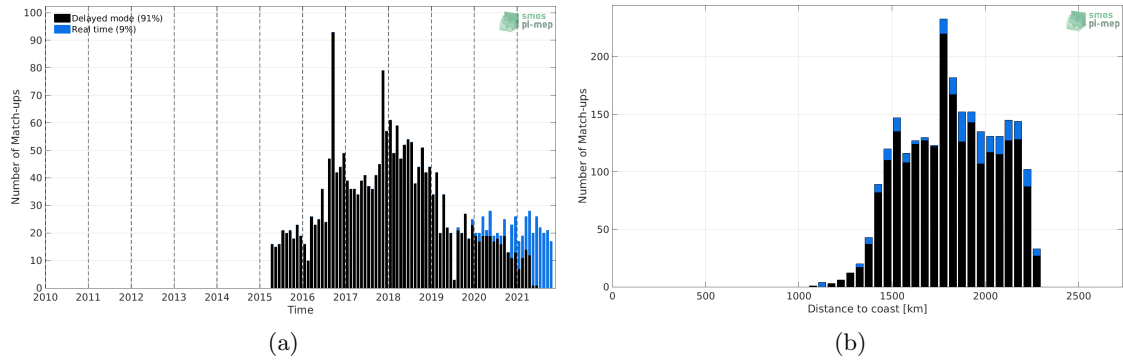
Figure 1: Number of match-ups between Argo and SMAP SSS L2 v5.0 (JPL) SSS as a function of time (a) and as function of the distance to coast (b) over the SPURS 2 Pi-MEP region and for the full satellite product period.
