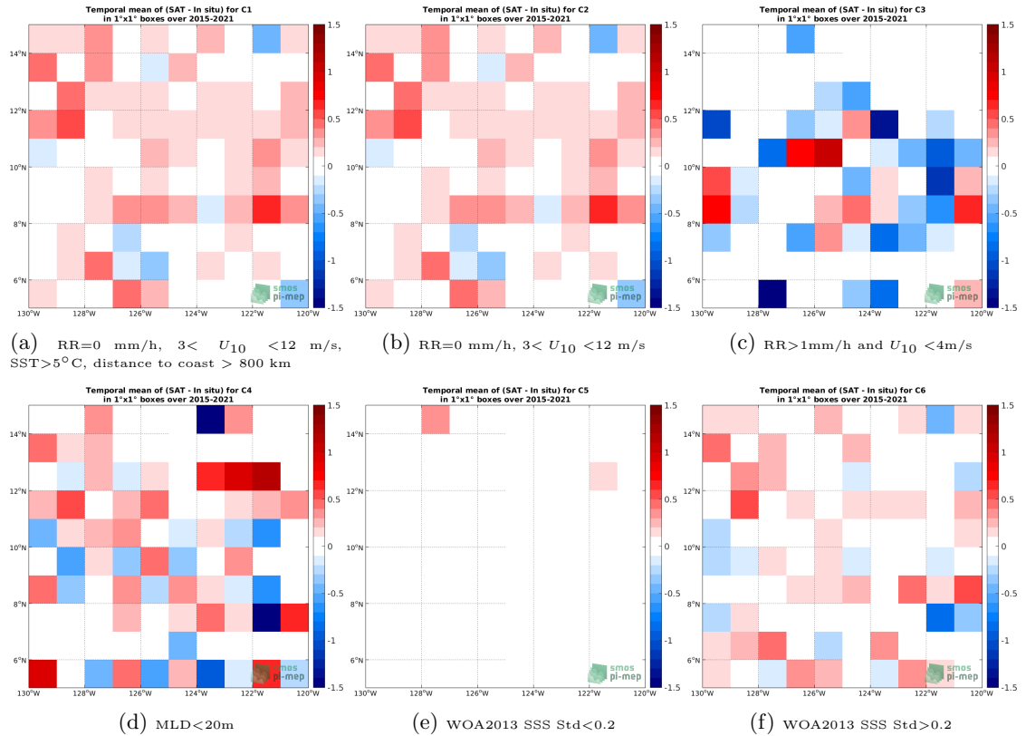
Figure 12: Temporal mean gridded over spatial boxes of size 1^\circ \times 1^\circ of \Delta SSS (SMAP SSS L2 v5.0 (JPL) - Argo) for 6 different subdatasets corresponding to:RR=0 mm/h, 3 < U_{10} < 12 m/s, SST >5^\circ C, distance to coast > 800 km (a), RR=0 mm/h, 3 < U_{10} < 12 m/s (b), RR >1 mm/h and U_{10} < 4 m/s (c),MLD <20 m (d),WOA2013 SSS Std <0.2 (e),WOA2013 SSS Std >0.2 (f).
