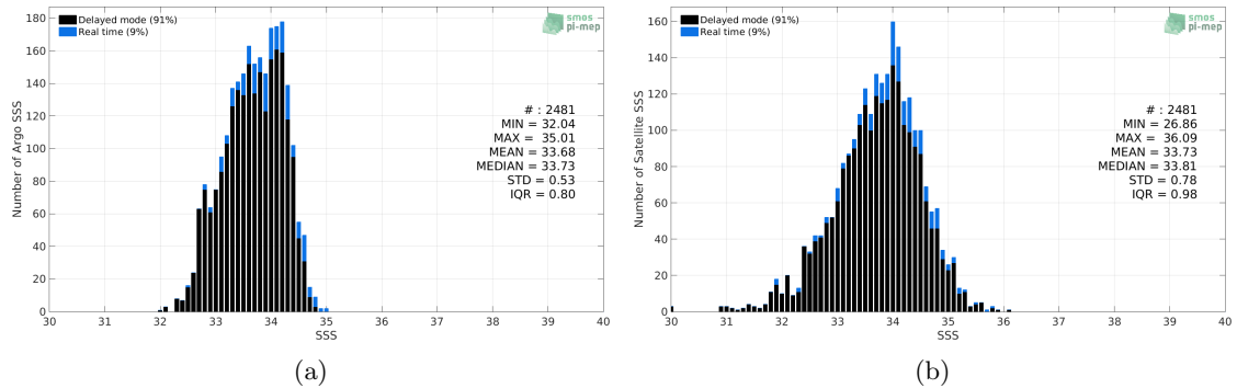
Figure 2: Histograms of SSS from Argo (a) and SMAP SSS L2 v5.0 (JPL) (b) considering all match-up pairs per bins of 0.1 over the SPURS 2 Pi-MEP region and for the full satellite product period.
