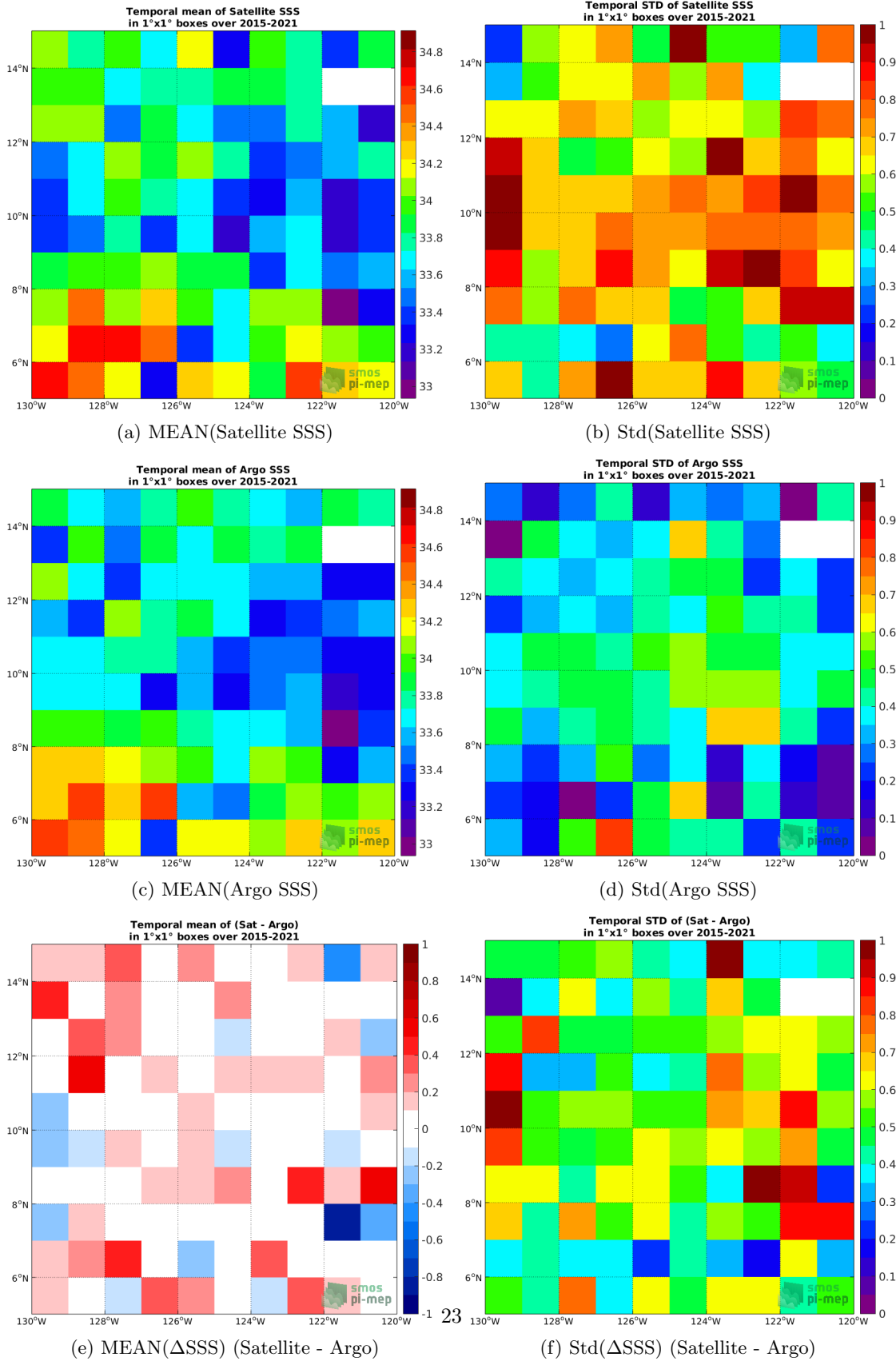
Figure 6: Temporal mean (left) and Std (right) of SSS from SMAP SSS L2 v5.0 (JPL) (top), Argo (middle), and of \Delta SSS (Satellite - Argo). Only match-up pairs are used to generate these maps.
