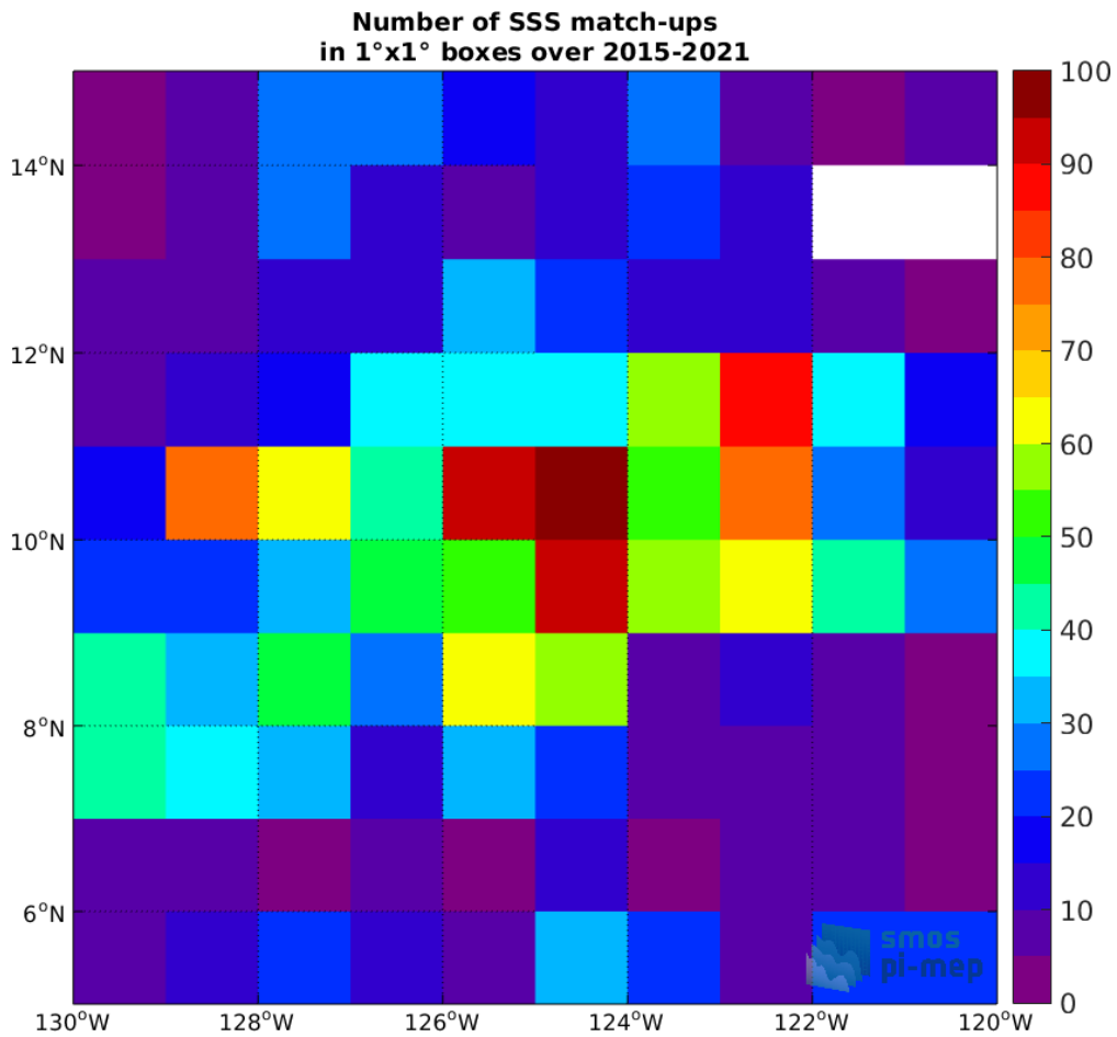
Figure 4: Number of SSS match-ups between Argo SSS and the SMAP SSS L2 v5.0 (JPL) SSS product for the SPURS 2 Pi-MEP region over 1°×1° boxes and for the full satellite product period.
