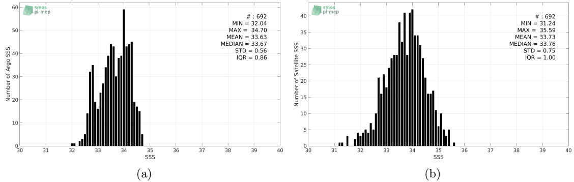
Figure 2: Histograms of SSS from Argo (a) and SMAP-L2-JPL-V4 (b) considering all match-up pairs per bins of 0.1 over the SPURS 2 Pi-MEP region and for the full satellite product period.
