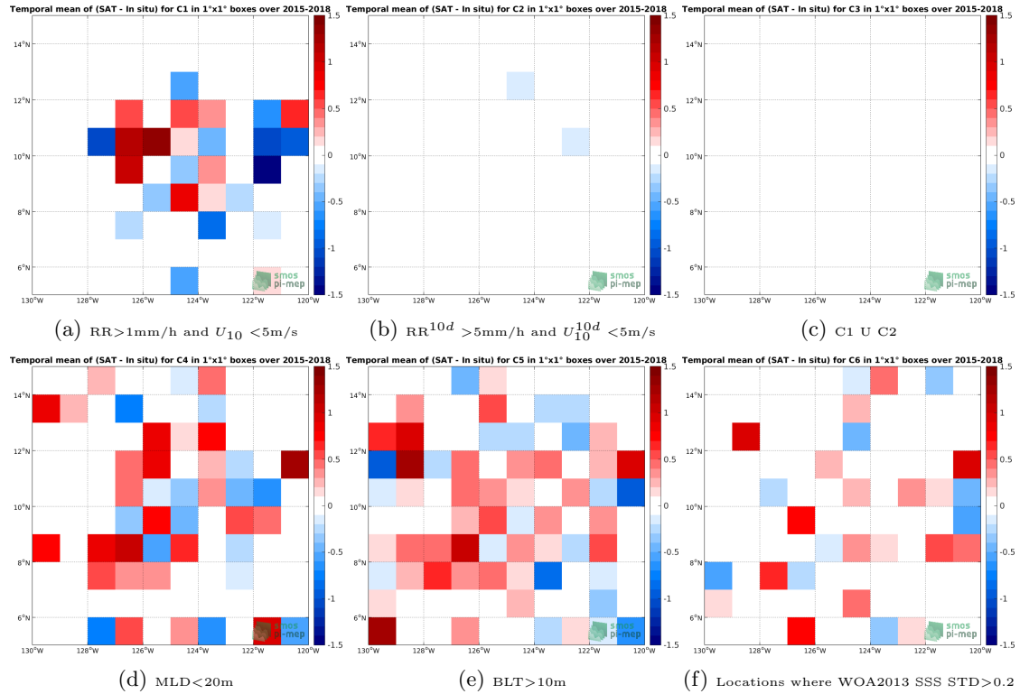
Figure 12: Temporal mean gridded over spatial boxes of size 1^\circ \times 1^\circ of \Delta\text{SSS} (SMAP-L2-JPL-V4 - Argo) for 6 different subdatasets corresponding to: \text{RR} > 1\text{mm/h} and U_{10} < 5\text{m/s} (a), \text{RR}^{10d} > 5\text{mm/h} and U_{10}^{10d} < 5\text{m/s} (b), C1 U C2 (c), \text{MLD} < 20\text{m} (d), \text{BLT} > 10\text{m} (e), Locations where WOA2013 SSS STD > 0.2 (f).
