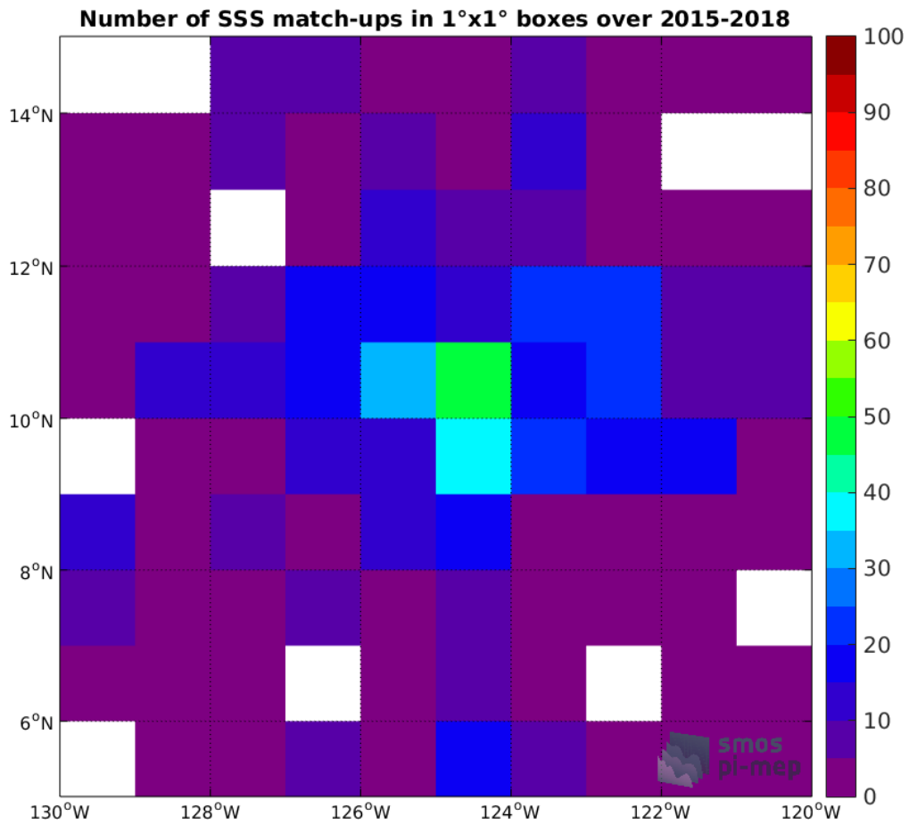
Figure 4: Number of SSS match-ups between Argo SSS and the SMAP-L2-JPL-V4 SSS product for the SPURS 2 Pi-MEP region over 1°x1° boxes and for the full satellite product period.
