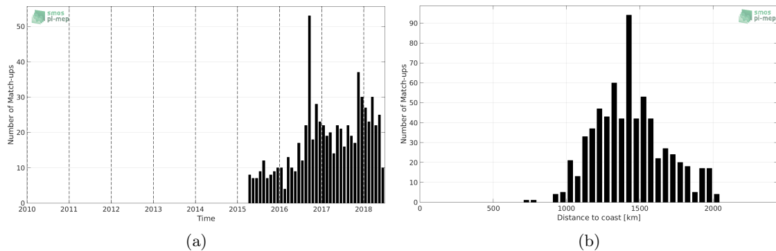
Figure 1: Number of match-ups between Argo and SMAP-L2-JPL-V4 SSS as a function of time (a) and as function of the distance to coast (b) over the SPURS 2 Pi-MEP region and for the full satellite product period.
