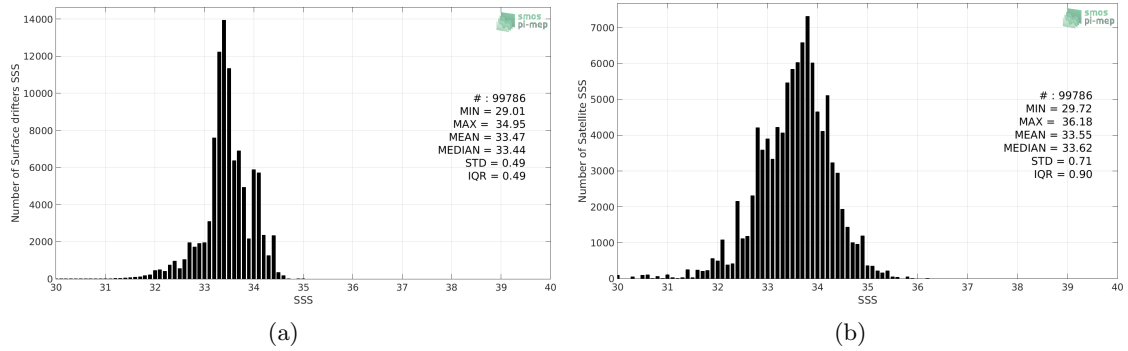
Figure 2: Histograms of SSS from Surface drifters (a) and SMAP-L2-JPL-V4.3 (b) considering all match-up pairs per bins of 0.1 over the SPURS 2 Pi-MEP region and for the full satellite product period.
