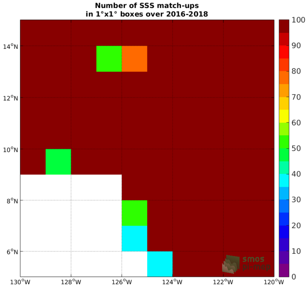
Figure 3: Number of SSS match-ups between Surface drifters SSS and the SMAP-L2-JPL-V4.3 SSS product for the SPURS 2 Pi-MEP region over 1°x1° boxes and for the full satellite product period.
