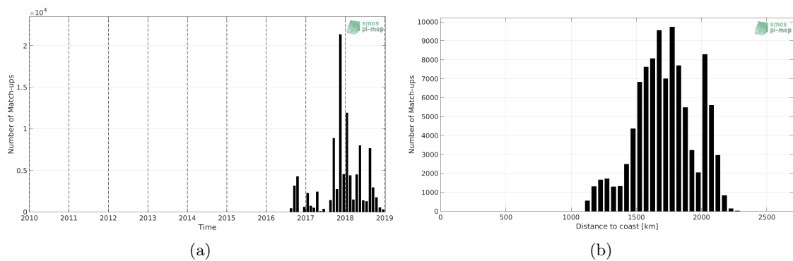
Figure 1: Number of match-ups between Surface drifters and SMAP-L2-JPL-V4.3 SSS as a function of time (a) and as function of the distance to coast (b) over the SPURS 2 Pi-MEP region and for the full satellite product period.
