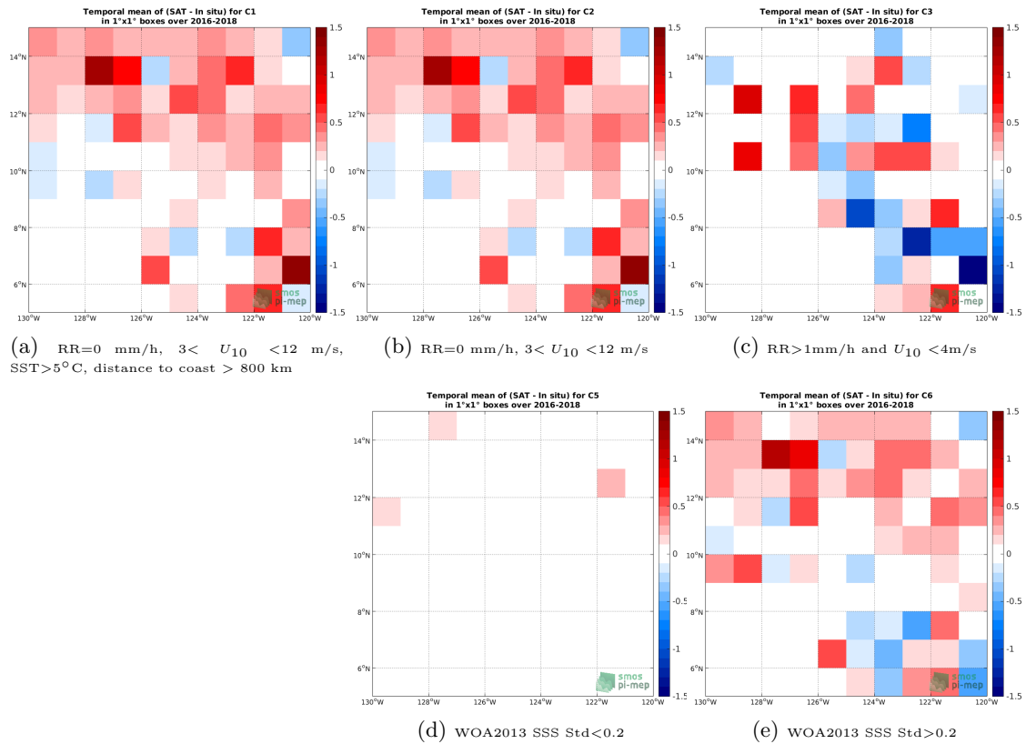
Figure 11: Temporal mean gridded over spatial boxes of size 1^\circ \times 1^\circ of \Delta SSS (SMAP-L2-JPL-V4.3 - Surface drifters) for 5 different subdatasets corresponding to:RR=0 mm/h, 3 < U_{10} < 12 m/s, SST >5^\circ\text{C} , distance to coast > 800 km (a), RR=0 mm/h, 3 < U_{10} < 12 m/s (b), RR >1 mm/h and U_{10} < 4 m/s (c), WOA2013 SSS Std <0.2 (d), WOA2013 SSS Std >0.2 (e).
