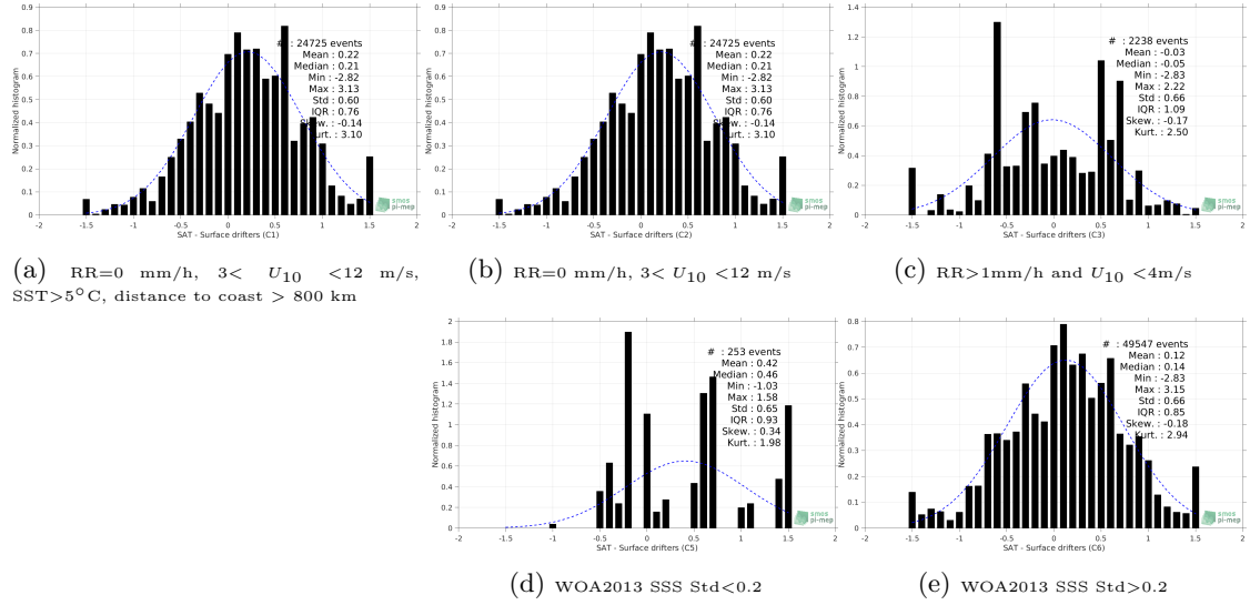
Figure 12: Normalized histogram of \Delta SSS (SMAP-L2-JPL-V4.3 - Surface drifters) for 5 different subdatasets corresponding to: RR=0 mm/h, 3 < U_{10} < 12 m/s, SST>5°C, distance to coast > 800 km (a), RR=0 mm/h, 3 < U_{10} < 12 m/s (b), RR>1mm/h and U_{10} < 4 m/s (c), WOA2013 SSS Std<0.2 (d), WOA2013 SSS Std>0.2 (e).
