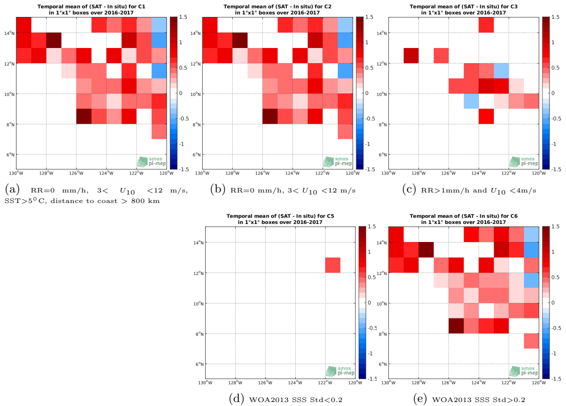
Figure 11: Temporal mean gridded over spatial boxes of size 1^\circ \times 1^\circ of \Delta SSS (SMAP-L2-JPL-V4.2 - Surface drifters) for 5 different subdatasets corresponding to:RR=0 mm/h, 3 < U_{10} < 12 m/s, SST >5^\circ C, distance to coast > 800 km (a), RR=0 mm/h, 3 < U_{10} < 12 m/s (b), RR >1 mm/h and U_{10} < 4 m/s (c), WOA2013 SSS Std <0.2 (d), WOA2013 SSS Std >0.2 (e).
