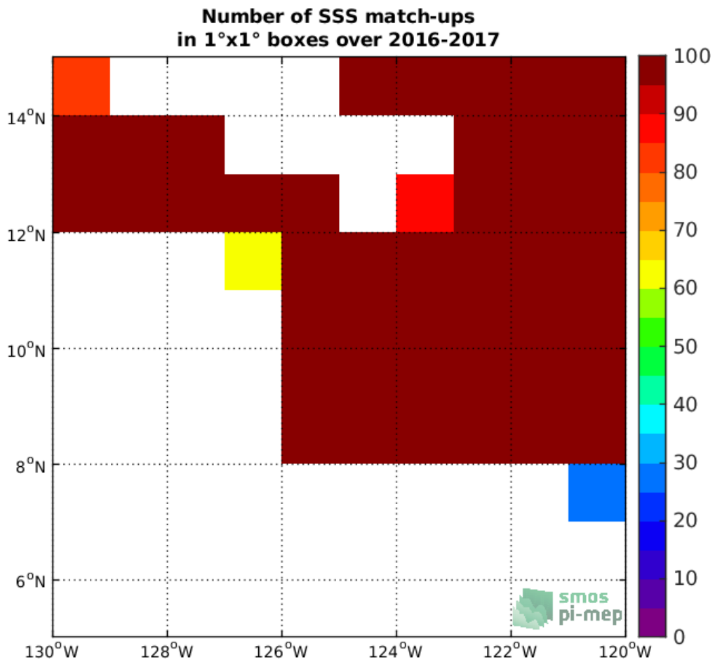
Figure 3: Number of SSS match-ups between Surface drifters SSS and the SMAP-L2-JPL-V4.2 SSS product for the SPURS 2 Pi-MEP region over 1°x1° boxes and for the full satellite product period.
