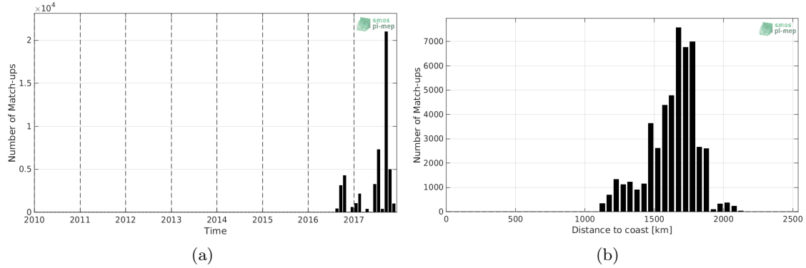
Figure 1: Number of match-ups between Surface drifters and SMAP-L2-JPL-V4.2 SSS as a function of time (a) and as function of the distance to coast (b) over the SPURS 2 Pi-MEP region and for the full satellite product period.
