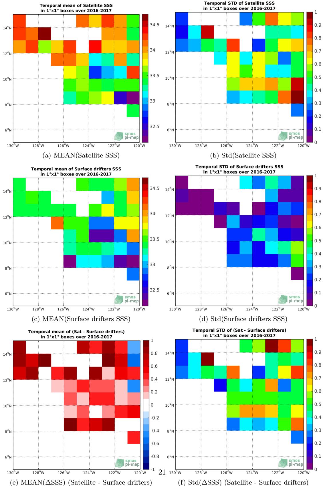
Figure 5: Temporal mean (left) and Std (right) of SSS from SMAP-L2-JPL-V4.2 (top), Surface drifters (middle), and of \Delta SSS (Satellite - Surface drifters). Only match-up pairs are used to generate these maps.
