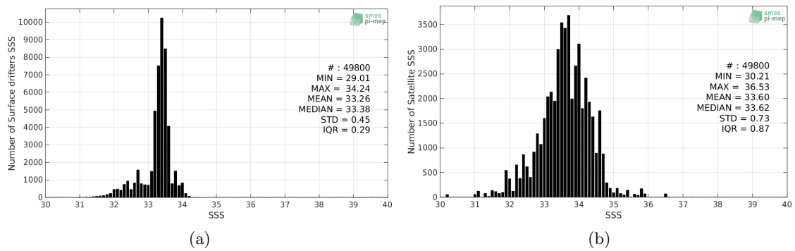
Figure 2: Histograms of SSS from Surface drifters (a) and SMAP-L2-JPL-V4.2 (b) considering all match-up pairs per bins of 0.1 over the SPURS 2 Pi-MEP region and for the full satellite product period.
