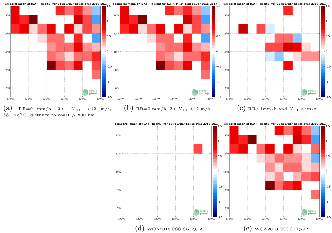
Figure 11: Temporal mean gridded over spatial boxes of size 1^\circ \times 1^\circ of \Delta SSS (SMAP-L2-JPL-V4.2 - Surface drifters) for 5 different subdatasets corresponding to: RR=0 mm/h, 3 < U_{10} < 12 m/s, SST > 5^\circ C , distance to coast > 800 km (a), RR=0 mm/h, 3 < U_{10} < 12 m/s (b), RR > 1 mm/h and U_{10} < 4 m/s (c), WOA2013 SSS Std <0.2 (d), WOA2013 SSS Std >0.2 (e).
