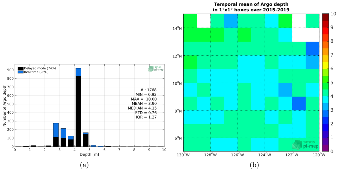
Figure 3: Histograms of the depth of the upper level SSS measurements from Argos in the Match-up DataBase for the SPURS 2 Pi-MEP region (a) and temporal mean spatial distribution of pressure of the in situ SSS data over 1^\circ \times 1^\circ boxes and for the full satellite product period (b).
