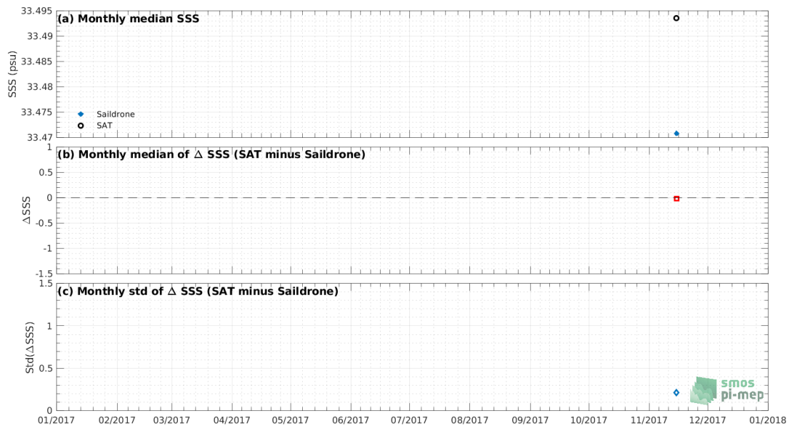
Figure 7: Time series of the monthly median SSS (top), median of \Delta SSS (Satellite - Sairdrone) and Std of \Delta SSS (Satellite - Sairdrone) over the SPURS 2 Pi-MEP region considering all match-ups collected by the Pi-MEP.
