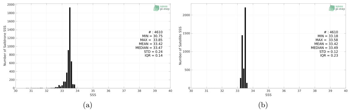
Figure 2: Histograms of SSS from Sairdron (a) and SMAP SSS L3 v5.0 - Monthly (JPL) (b) considering all match-up pairs per bins of 0.1 over the SPURS 2 Pi-MEP region and for the full satellite product period.
