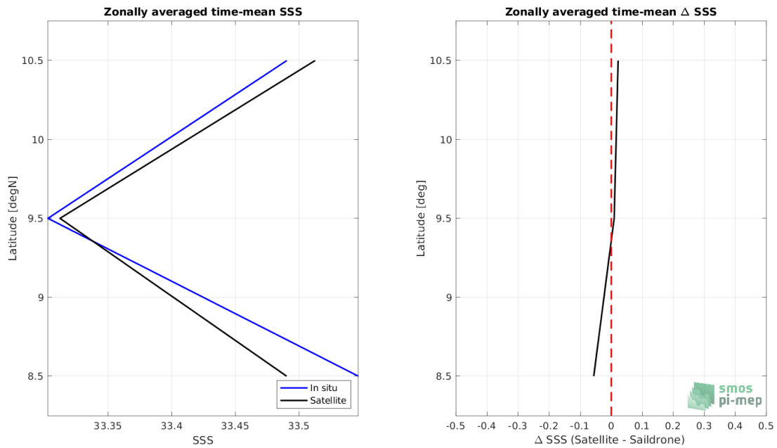
Figure 8: Left panel: Zonal mean SSS from SMAP SSS L3 v5.0 - Monthly (JPL) satellite product (black) and from Sairdron (blue). Right panel: Zonal mean of \Delta SSS (Satellite - Sairdron) for all the collected Pi-MEP match-up pairs estimated over the full satellite product period.
