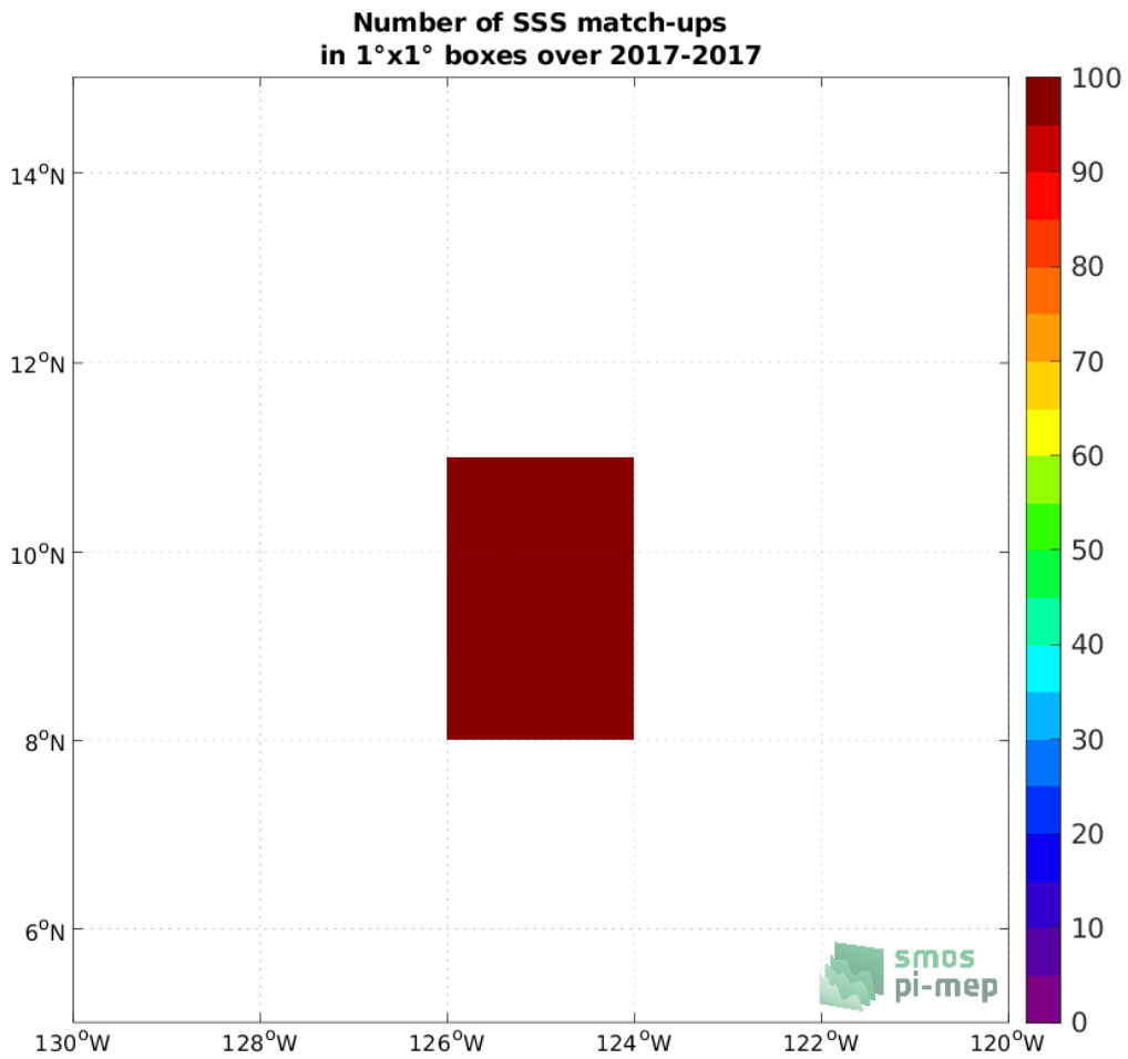
Figure 4: Number of SSS match-ups between Saildrone SSS and the SMAP SSS L3 v5.0 - Monthly (JPL) SSS product for the SPURS 2 Pi-MEP region over 1°x1° boxes and for the full satellite product period.
