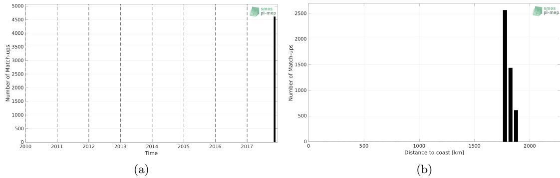
Figure 1: Number of match-ups between Sairdron and SMAP SSS L3 v5.0 - Monthly (JPL) SSS as a function of time (a) and as function of the distance to coast (b) over the SPURS 2 Pi-MEP region and for the full satellite product period.
