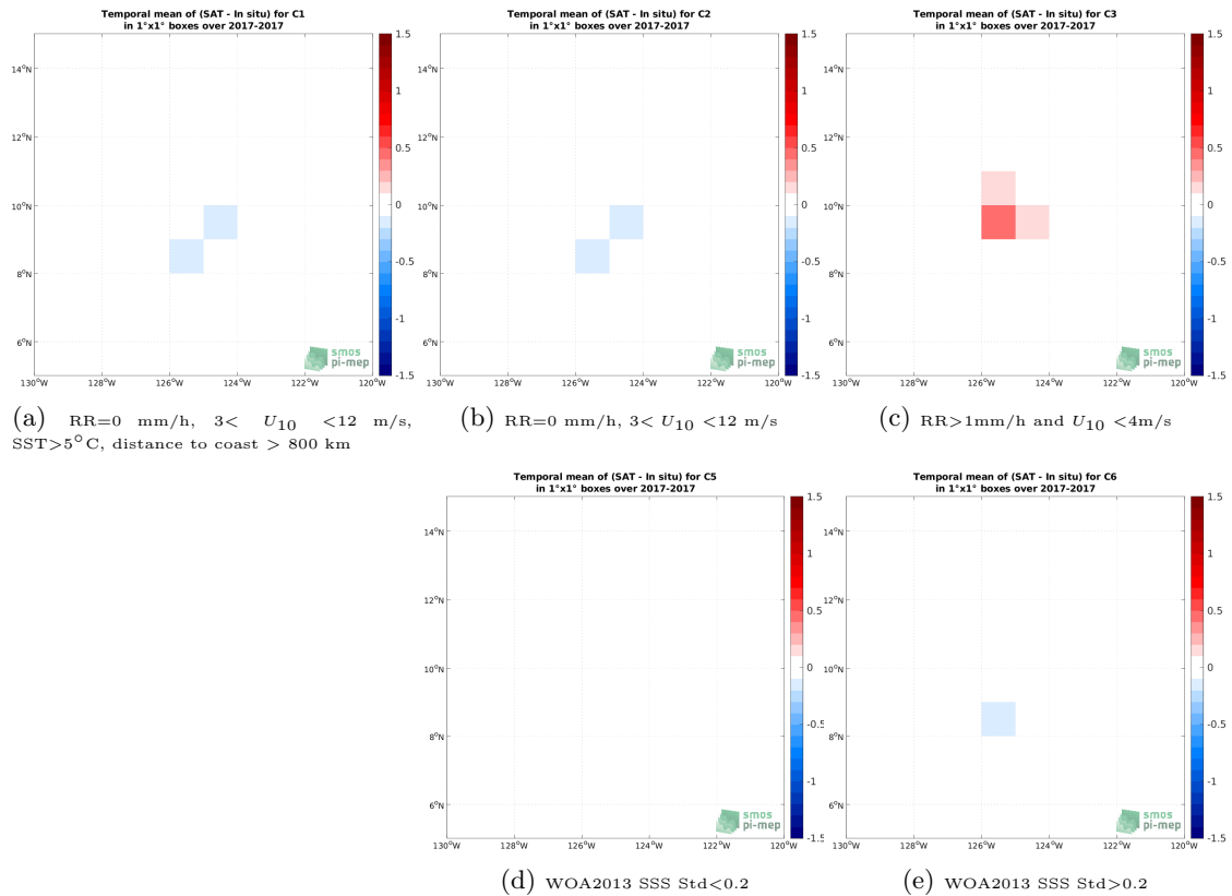
Figure 12: Temporal mean gridded over spatial boxes of size 1^\circ \times 1^\circ of \Delta SSS (SMAP SSS L3 v5.0 - Monthly (JPL) - Saildrone) for 5 different subdatasets corresponding to:RR=0 mm/h, 3 < U_{10} < 12 m/s, SST >5^\circ C, distance to coast > 800 km (a), RR=0 mm/h, 3 < U_{10} < 12 m/s (b), RR >1 mm/h and U_{10} < 4 m/s (c), WOA2013 SSS Std <0.2 (d), WOA2013 SSS Std >0.2 (e).
