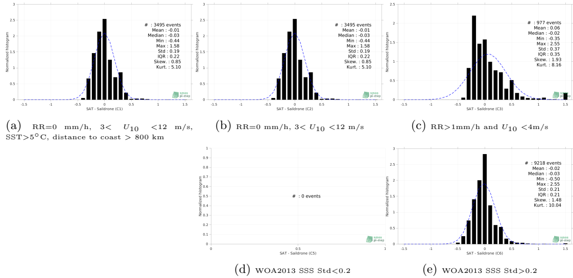
Figure 12: Normalized histogram of \Delta SSS (SMAP SSS L3 v5.0 - Monthly (JPL) - Saildrone) for 5 different subdatasets corresponding to: RR=0 mm/h, 3 < U_{10} < 12 m/s, SST > 5°C, distance to coast > 800 km (a), RR=0 mm/h, 3 < U_{10} < 12 m/s (b), RR > 1mm/h and U_{10} < 4 m/s (c), WOA2013 SSS Std < 0.2 (d), WOA2013 SSS Std > 0.2 (e).
