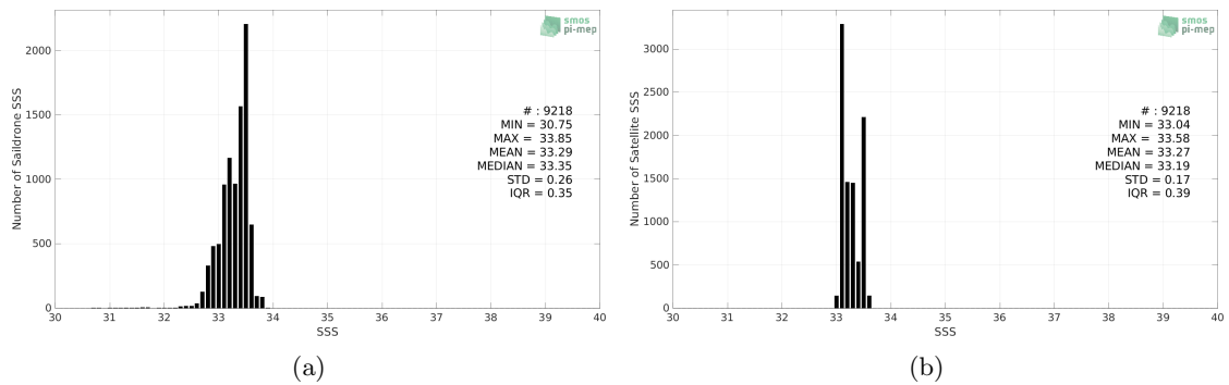
Figure 2: Histograms of SSS from Sairdrone (a) and SMAP SSS L3 v5.0 - Monthly (JPL) (b) considering all match-up pairs per bins of 0.1 over the SPURS 2 Pi-MEP region and for the full satellite product period.
