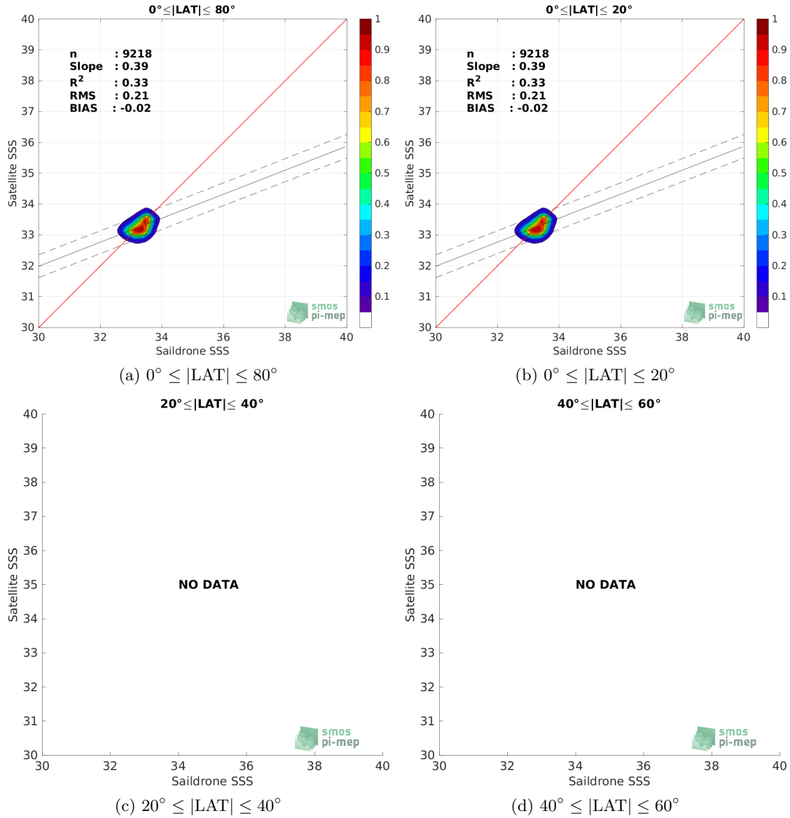
Figure 8: Contour maps of the concentration of SMAP SSS L3 v5.0 - Monthly (JPL) SSS (y-axis) versus Saildrone SSS (x-axis) at match-up pairs for different latitude bands. For each plot, the red line shows x=y . The black thin and dashed lines indicate a linear fit through the data cloud and the \pm 95\% confidence levels, respectively. The number match-up pairs n , the slope and R^2 coefficient of the linear fit, the root mean square (RMS) and the mean bias between satellite and in situ data are indicated for each latitude band in each plots.
