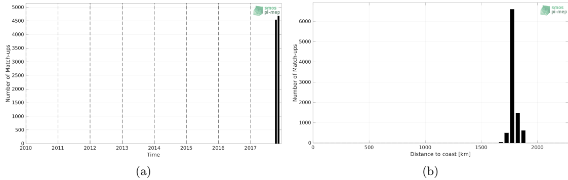
Figure 1: Number of match-ups between Sairdrone and SMAP SSS L3 v5.0 - Monthly (JPL) SSS as a function of time (a) and as function of the distance to coast (b) over the SPURS 2 Pi-MEP region and for the full satellite product period.
