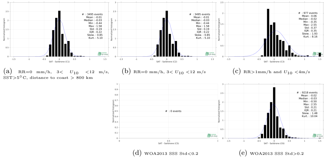
Figure 12: Normalized histogram of \Delta\text{SSS} (SMAP SSS L3 v5.0 - Monthly (JPL) - Saildrone) for 5 different subdatasets corresponding to: RR=0 mm/h, 3 < U_{10} < 12 m/s, SST > 5^\circ\text{C} , distance to coast > 800 km (a), RR=0 mm/h, 3 < U_{10} < 12 m/s (b), RR > 1\text{mm/h} and U_{10} < 4\text{m/s} (c), WOA2013 SSS Std < 0.2 (d), WOA2013 SSS Std > 0.2 (e).
