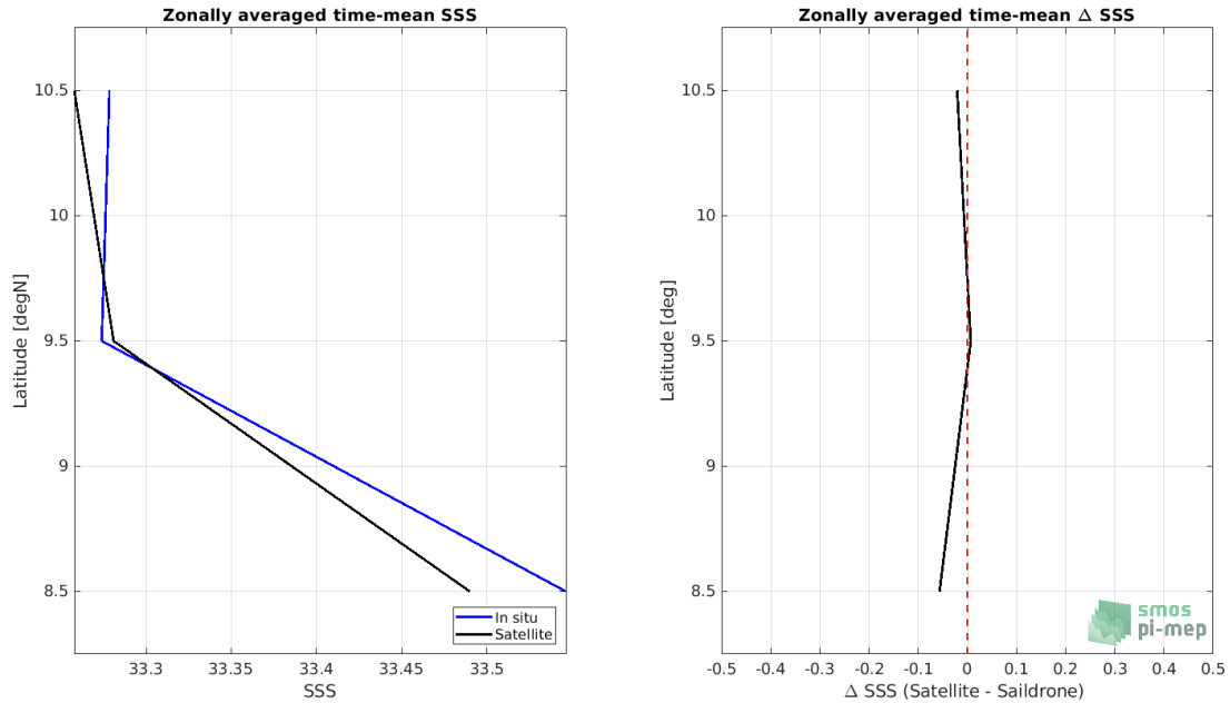
Figure 7: Left panel: Zonal mean SSS from SMAP SSS L3 v5.0 - Monthly (JPL) satellite product (black) and from Sairdrone (blue). Right panel: Zonal mean of \Delta SSS (Satellite - Sairdrone) for all the collected Pi-MEP match-up pairs estimated over the full satellite product period.
