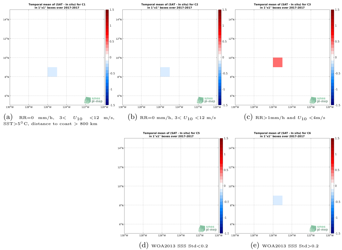
Figure 11: Temporal mean gridded over spatial boxes of size 1^\circ \times 1^\circ of \Delta SSS (SMAP SSS L3 v5.0 - Monthly (JPL) - Saildrone) for 5 different subdatasets corresponding to: RR=0 mm/h, 3 < U_{10} < 12 m/s, SST > 5^\circ\text{C} , distance to coast > 800 km (a), RR=0 mm/h, 3 < U_{10} < 12 m/s (b), RR > 1\text{mm/h} and U_{10} < 4\text{m/s} (c), WOA2013 SSS Std < 0.2 (d), WOA2013 SSS Std > 0.2 (e).
