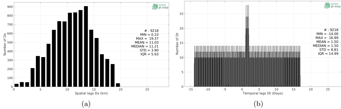
Figure 4: Histograms of the spatial (a) and temporal (b) lags between the location/time of the Saildrone measurement and the date of the corresponding SMAP SSS L3 v5.0 - Monthly (JPL) SSS pixel.
