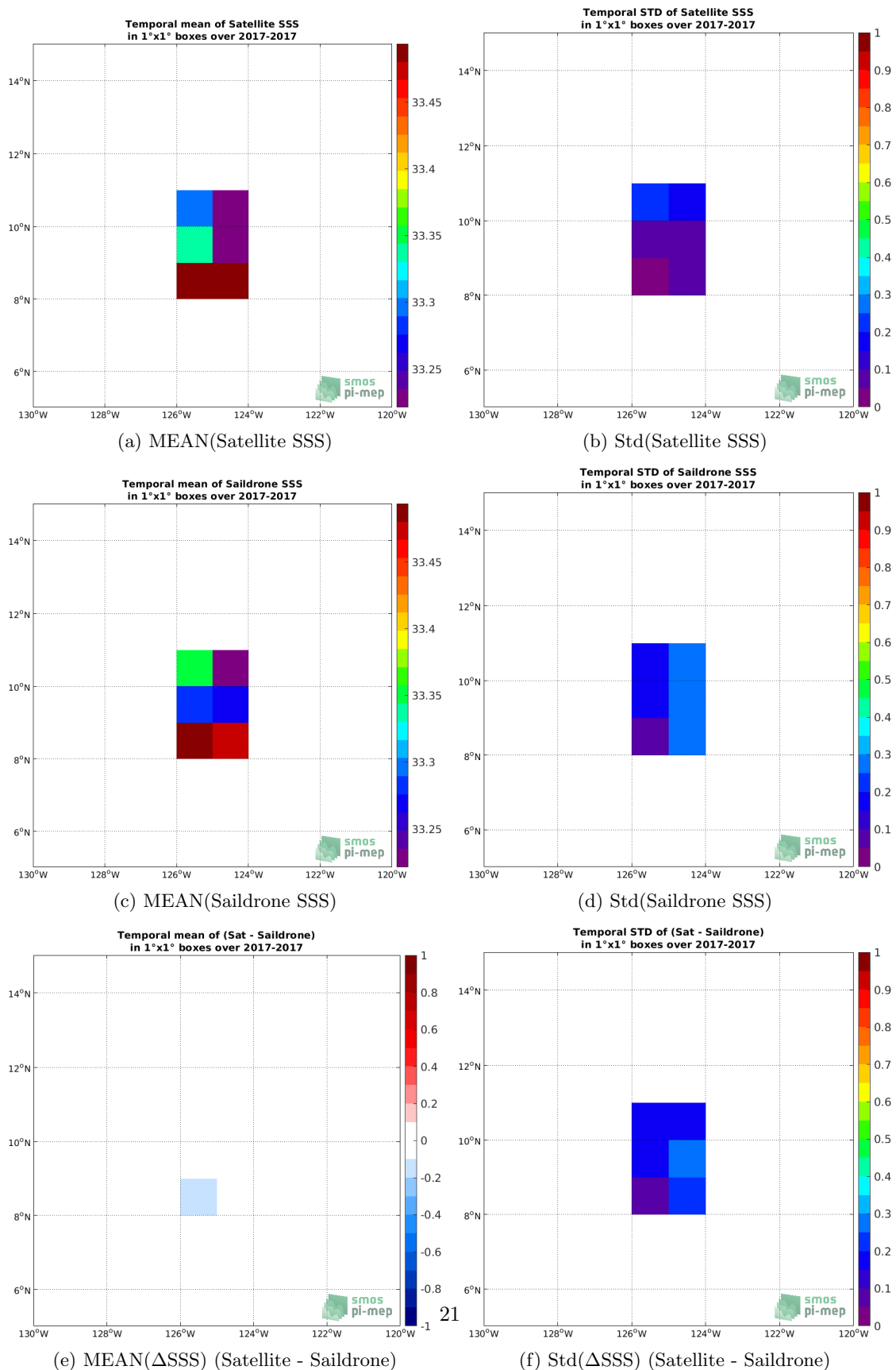
Figure 5: Temporal mean (left) and Std (right) of SSS from SMAP SSS L3 v5.0 - Monthly (JPL) (top), Saildrone (middle), and of \Delta SSS (Satellite - Saildrone). Only match-up pairs are used to generate these maps.
