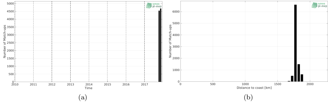
Figure 1: Number of match-ups between Saildrone and SMAP SSS L3 v5.0 - Monthly (JPL) SSS as a function of time (a) and as function of the distance to coast (b) over the SPURS 2 Pi-MEP region and for the full satellite product period.
