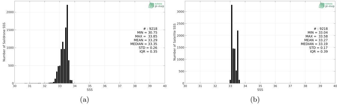
Figure 2: Histograms of SSS from Saildrone (a) and SMAP SSS L3 v5.0 - Monthly (JPL) (b) considering all match-up pairs per bins of 0.1 over the SPURS 2 Pi-MEP region and for the full satellite product period.
