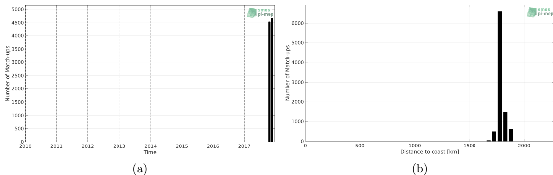
Figure 1: Number of match-ups between Saldrone and SMAP SSS L3 v5.0 - Monthly (JPL) SSS as a function of time (a) and as function of the distance to coast (b) over the SPURS 2 Pi-MEP region and for the full satellite product period.
