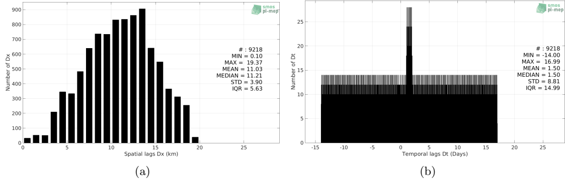
Figure 5: Histograms of the spatial (a) and temporal (b) lags between the time of the Saildrone measurements and the date of the corresponding SMAP SSS L3 v5.0 - Monthly (JPL) SSS product.
