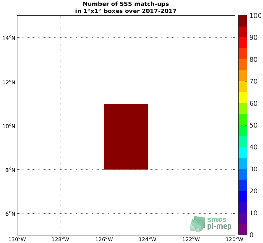
Figure 4: Number of SSS match-ups between Saildrone SSS and the SMAP SSS L3 v5.0 - Monthly (JPL) SSS product for the SPURS 2 Pi-MEP region over 1°x1° boxes and for the full satellite product period.
