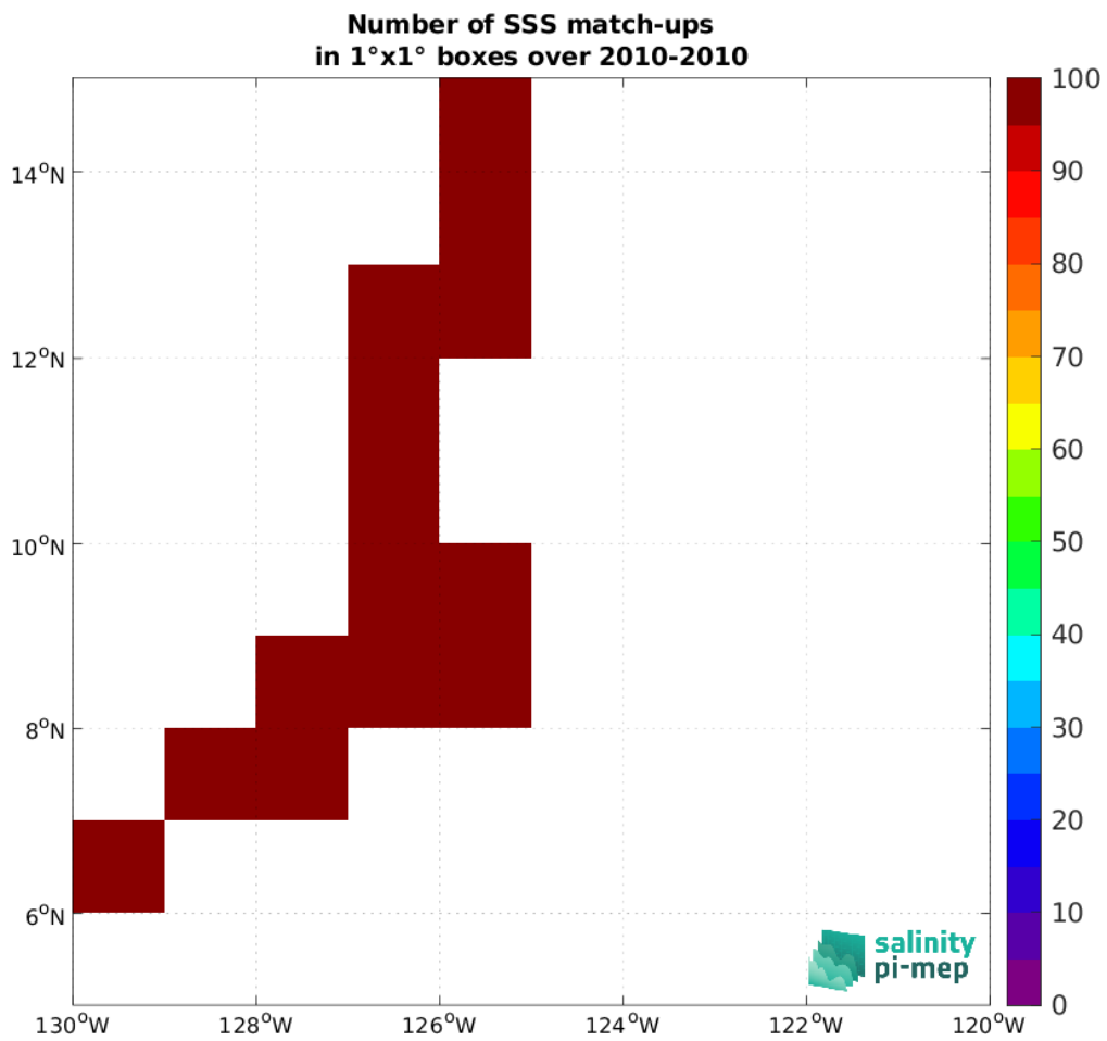
Figure 5: Number of SSS match-ups between TSG (GOSUD-Sailing-ship) SSS and the ISAS SSS product for the SPURS 2 Pi-MEP region over 1°x1° boxes and for the full satellite product period.
