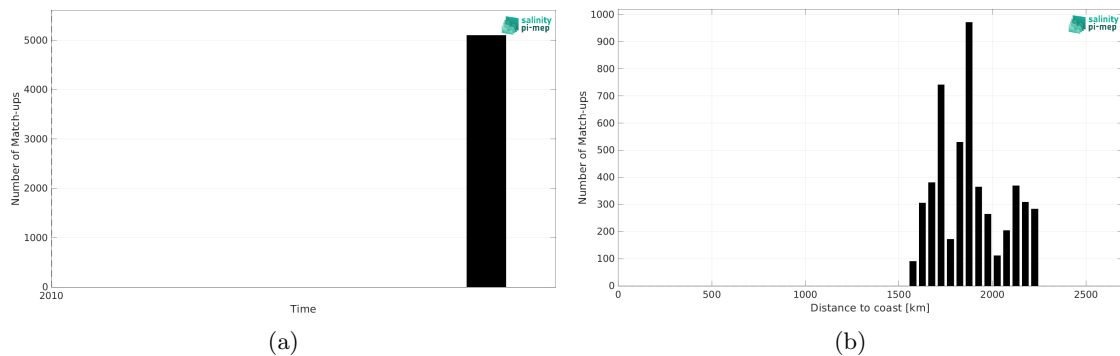
Figure 2: Number of match-ups between TSG (GOSUD-Sailing-ship) and ISAS SSS as a function of time (a) and as function of the distance to coast (b) over the SPURS 2 Pi-MEP region and for the full satellite product period.
