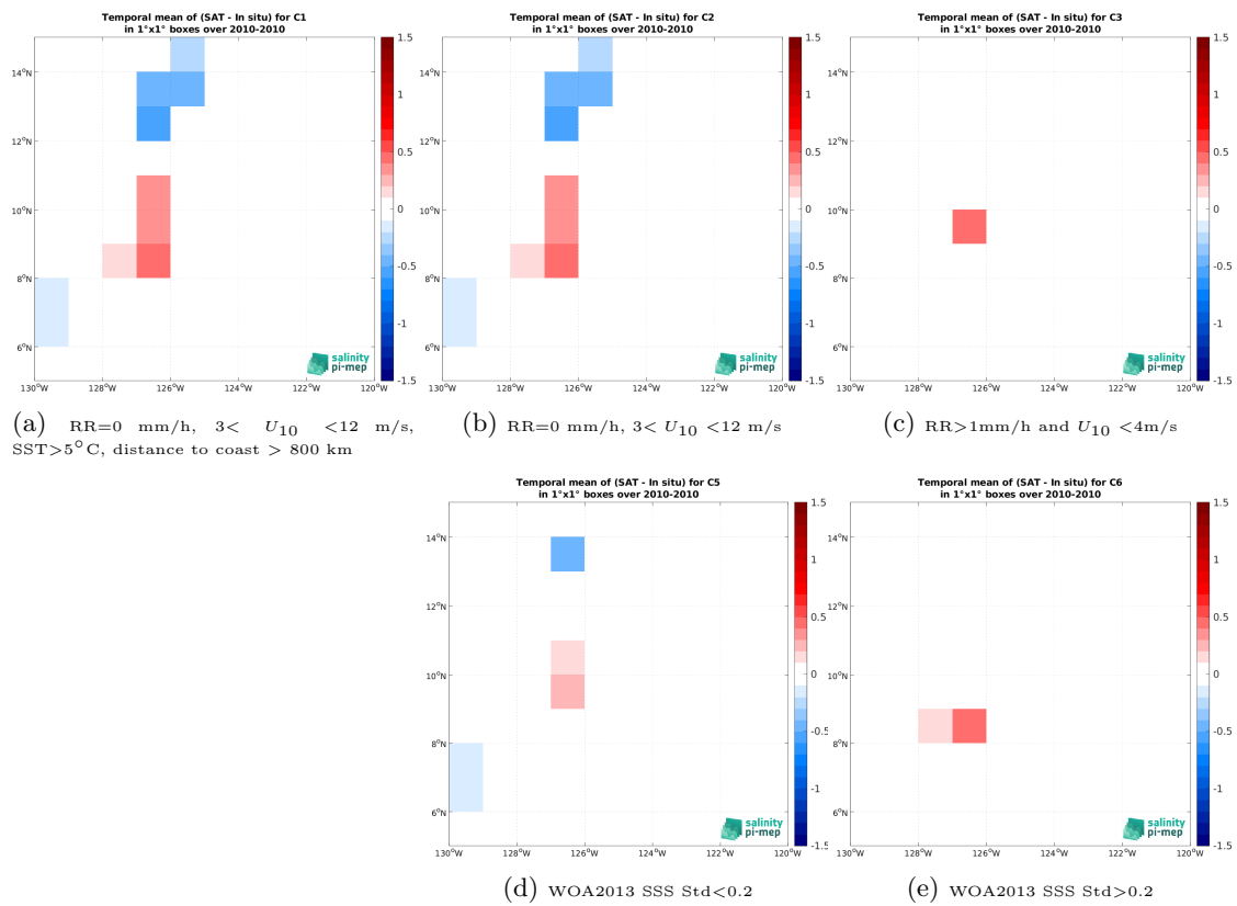
Figure 14: Temporal mean gridded over spatial boxes of size 1^\circ \times 1^\circ of \Delta SSS (ISAS - TSG (GOSUD-Sailing-ship)) for 5 different subdatasets corresponding to:RR=0 mm/h, 3 < U_{10} < 12 m/s, SST>5°C, distance to coast > 800 km (a), RR=0 mm/h, 3 < U_{10} < 12 m/s (b), RR>1mm/h and U_{10} < 4 m/s (c), WOA2013 SSS Std<0.2 (d), WOA2013 SSS Std>0.2 (e).
