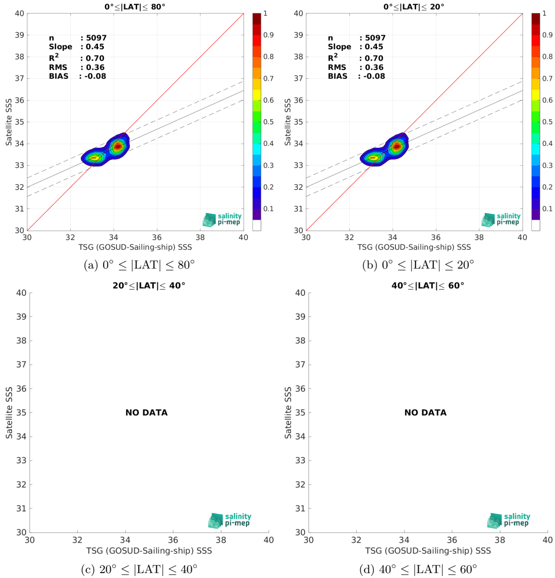
Figure 10: Contour maps of the concentration of ISAS SSS (y-axis) versus TSG (GOSUD-Sailing-ship) SSS (x-axis) at match-up pairs for different latitude bands. For each plot, the red line shows x=y . The black thin and dashed lines indicate a linear fit through the data cloud and the \pm 95\% confidence levels, respectively. The number match-up pairs n , the slope and R^2 coefficient of the linear fit, the root mean square (RMS) and the mean bias between satellite and in situ data are indicated for each latitude band in each plots.
