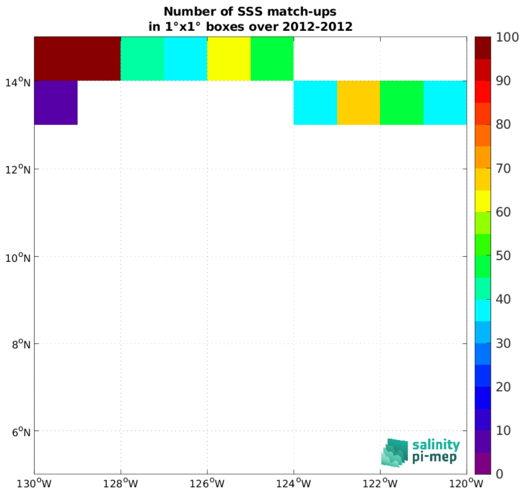
Figure 5: Number of SSS match-ups between TSG (GOSUD-Research-vessel) SSS and the ISAS SSS product for the SPURS 2 Pi-MEP region over 1°x1° boxes and for the full satellite product period.
