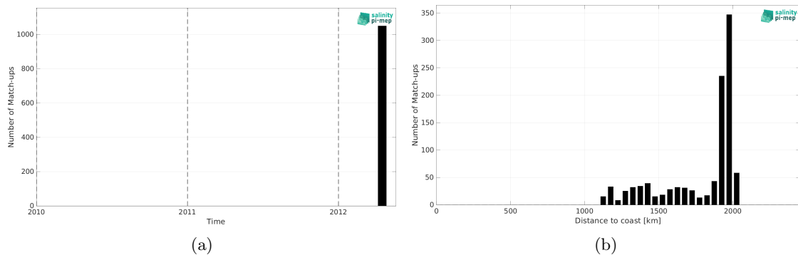
Figure 2: Number of match-ups between TSG (GOSUD-Research-vessel) and ISAS SSS as a function of time (a) and as function of the distance to coast (b) over the SPURS 2 Pi-MEP region and for the full satellite product period.
