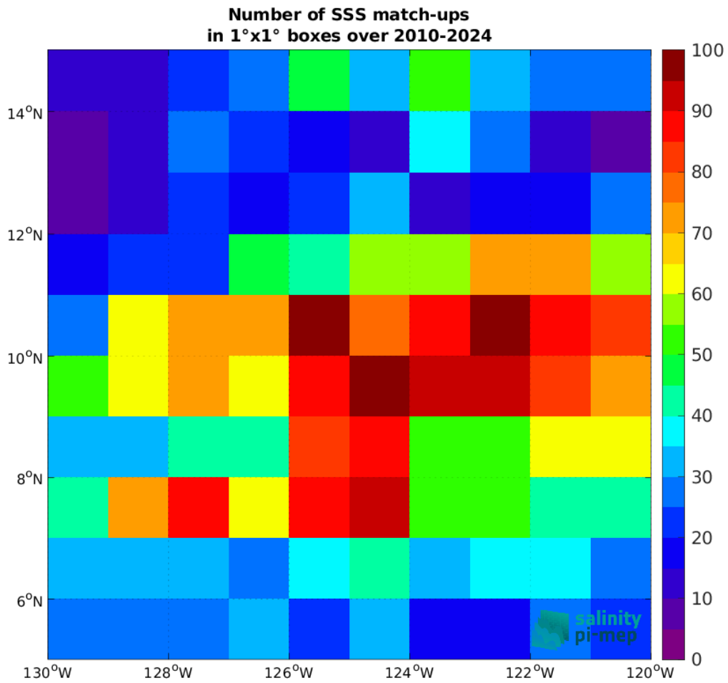
Figure 5: Number of SSS match-ups between Argo SSS and the ISAS SSS product for the SPURS 2 Pi-MEP region over 1°x1° boxes and for the full satellite product period.
