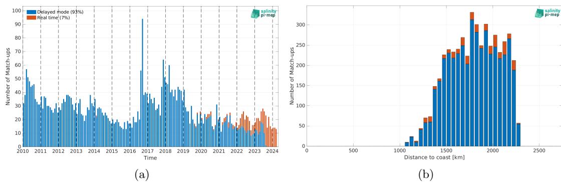
Figure 2: Number of match-ups between Argo and ISAS SSS as a function of time (a) and as function of the distance to coast (b) over the SPURS 2 Pi-MEP region and for the full satellite product period.
