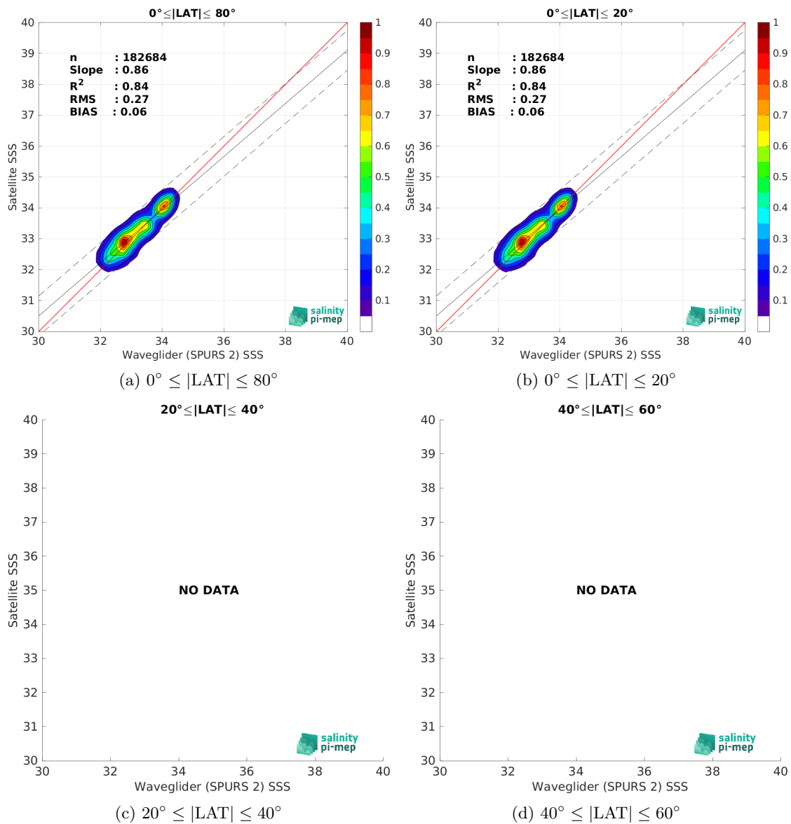
Figure 10: Contour maps of the concentration of CCI SSS L4 Merged-OI v5.5 - 7-day running (ESA) SSS (y-axis) versus Waveglider (SPURS 2) SSS (x-axis) at match-up pairs for different latitude bands. For each plot, the red line shows x=y . The black thin and dashed lines indicate a linear fit through the data cloud and the \pm 95\% confidence levels, respectively. The number match-up pairs n , the slope and R^2 coefficient of the linear fit, the root mean square (RMS) and the mean bias between satellite and in situ data are indicated for each latitude band in each plots.
