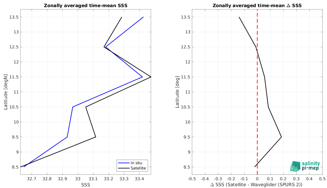
Figure 9: Left panel: Zonal mean SSS from CCI SSS L4 Merged-OI v5.5 - 7-day running (ESA) satellite product (black) and from Waveglider (SPURS 2) (blue). Right panel: Zonal mean of \Delta SSS (Satellite - Waveglider (SPURS 2)) for all the collected Pi-MEP match-up pairs estimated over the full satellite product period.
