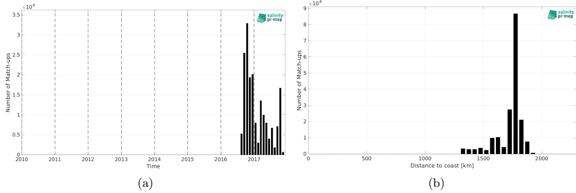
Figure 2: Number of match-ups between Waveglider (SPURS 2) and CCI SSS L4 Merged-OI v5.5 - 7-day running (ESA) SSS as a function of time (a) and as function of the distance to coast (b) over the SPURS 2 Pi-MEP region and for the full satellite product period.
