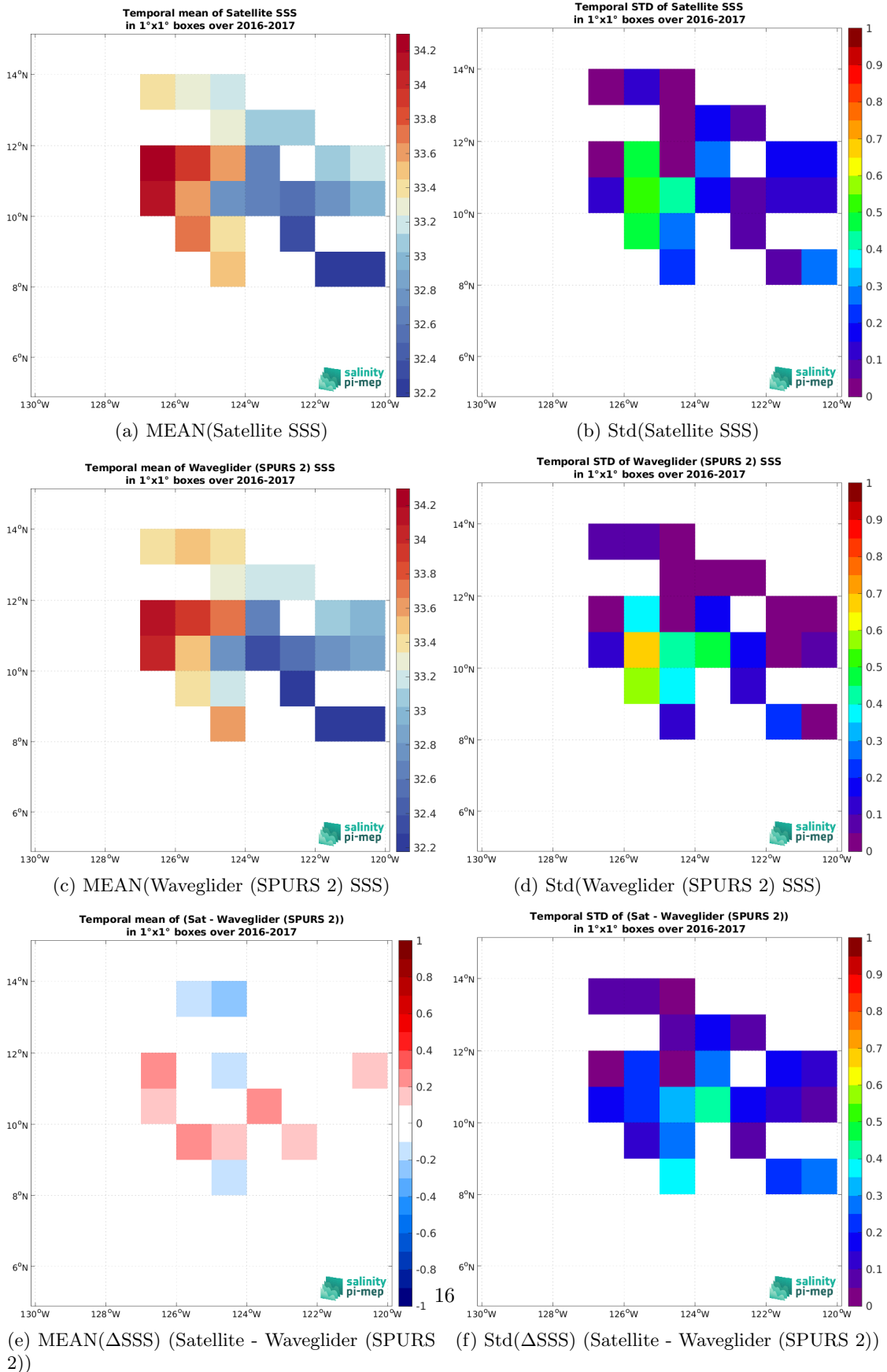
Figure 7: Temporal mean (left) and Std (right) of SSS from CCI SSS L4 Merged-OI v5.5 - 7-day running (ESA) (top), Waveglider (SPURS 2) (middle), and of \Delta SSS (Satellite - Waveglider (SPURS 2)). Only match-up pairs are used to generate these maps.
