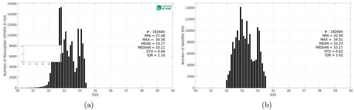
Figure 3: Histograms of SSS from Waveglider (SPURS 2) (a) and CCI SSS L4 Merged-OI v5.5 - 7-day running (ESA) (b) considering all match-up pairs per bins of 0.1 over the SPURS 2 Pi-MEP region and for the full satellite product period.
