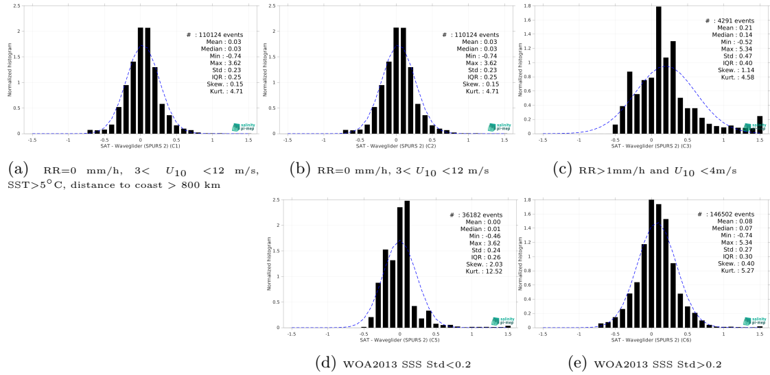
Figure 15: Normalized histogram of \Delta\text{SSS} (CCI SSS L4 Merged-OI v5.5 - 7-day running (ESA) - Waveglider (SPURS 2)) for 5 different subdatasets corresponding to: RR=0 mm/h, 3 < U_{10} < 12 m/s, SST >5^{\circ}\text{C} , distance to coast > 800 km (a), RR=0 mm/h, 3 < U_{10} < 12 m/s (b), RR >1 mm/h and U_{10} < 4 m/s (c), WOA2013 SSS Std <0.2 (d), WOA2013 SSS Std >0.2 (e).
