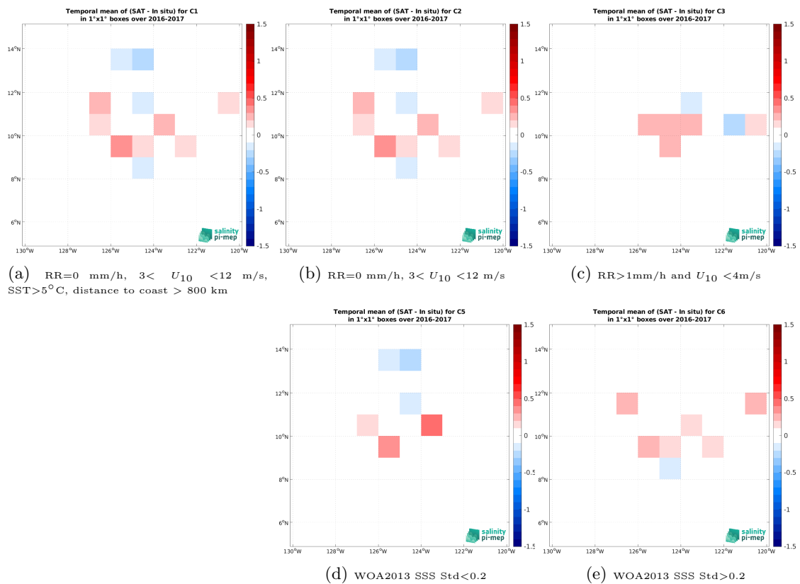
Figure 14: Temporal mean gridded over spatial boxes of size 1^\circ \times 1^\circ of \Delta\text{SSS} (CCI SSS L4 Merged-OI v5.5 - 7-day running (ESA) - Waveglider (SPURS 2)) for 5 different subdatasets corresponding to:RR=0 mm/h, 3 < U_{10} < 12 m/s, SST >5^\circ\text{C} , distance to coast > 800 km (a), RR=0 mm/h, 3 < U_{10} < 12 m/s (b), RR >1 mm/h and U_{10} < 4 m/s (c), WOA2013 SSS Std <0.2 (d), WOA2013 SSS Std >0.2 (e).
