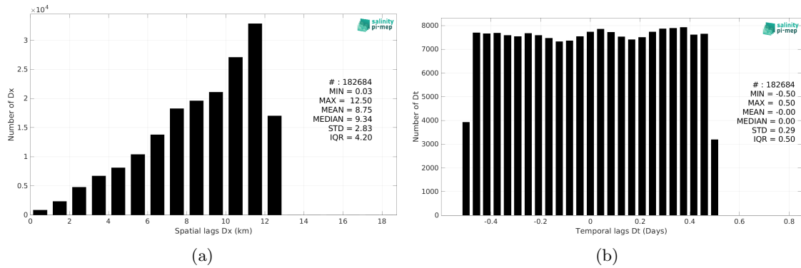
Figure 6: Histograms of the spatial (a) and temporal (b) lags between the location/time of the Waveglider (SPURS 2) measurement and the date of the corresponding CCI SSS L4 Merged-OI v5.5 - 7-day running (ESA) SSS pixel.
