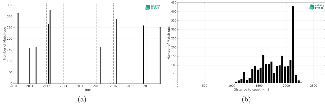
Figure 2: Number of match-ups between TSG (SAMOS) and CCI SSS L4 Merged-OI v5.5 - 7-day running (ESA) SSS as a function of time (a) and as function of the distance to coast (b) over the SPURS 2 Pi-MEP region and for the full satellite product period.
