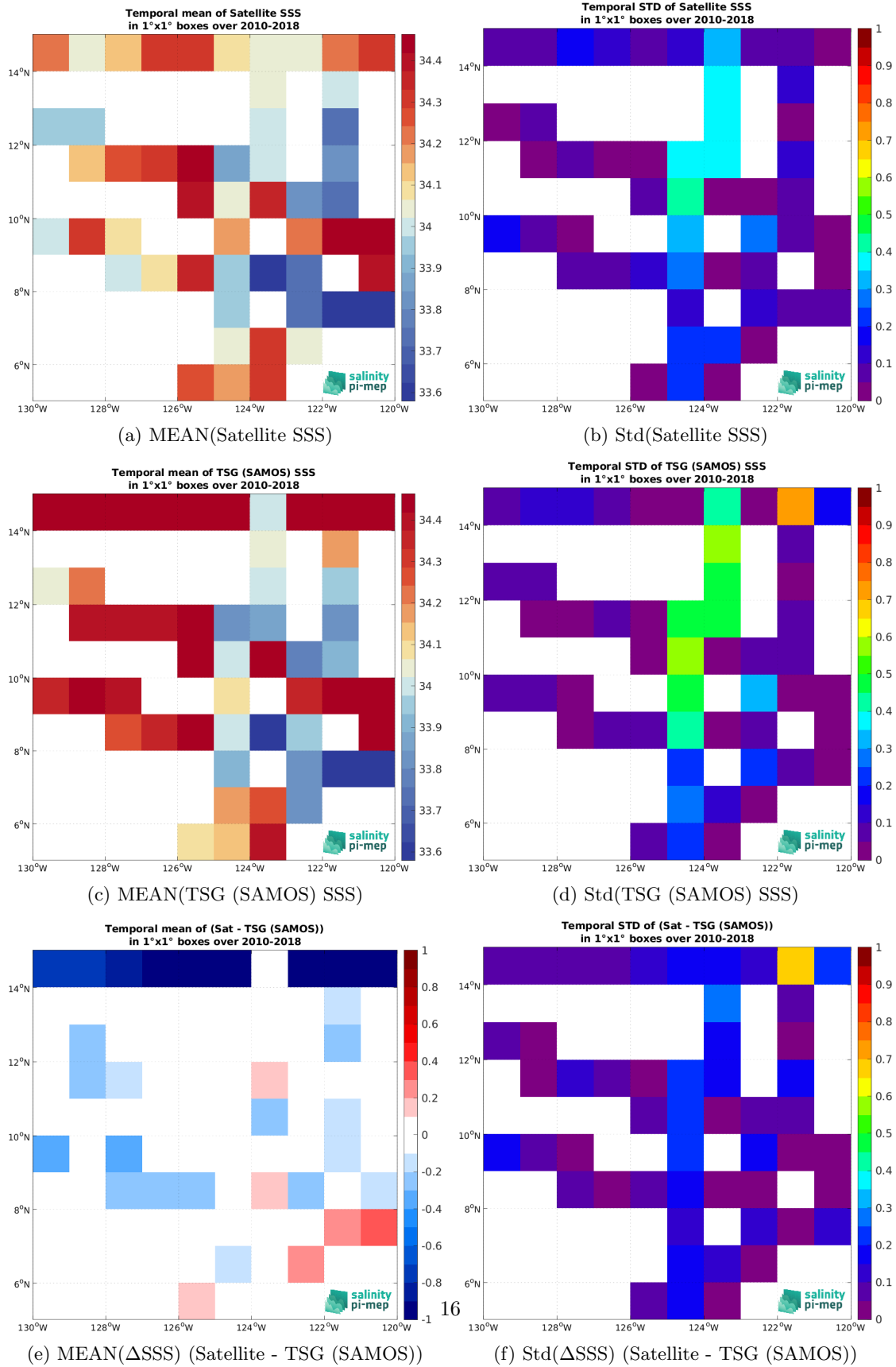
Figure 7: Temporal mean (left) and Std (right) of SSS from CCI SSS L4 Merged-OI v5.5 - 7-day running (ESA) (top), TSG (SAMOS) (middle), and of \Delta SSS (Satellite - TSG (SAMOS)). Only match-up pairs are used to generate these maps.
