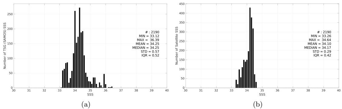
Figure 3: Histograms of SSS from TSG (SAMOS) (a) and CCI SSS L4 Merged-OI v5.5 - 7-day running (ESA) (b) considering all match-up pairs per bins of 0.1 over the SPURS 2 Pi-MEP region and for the full satellite product period.
