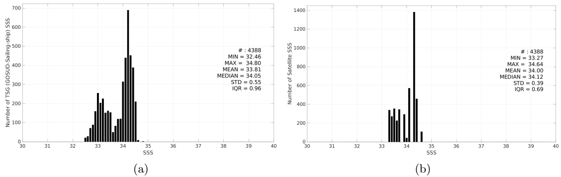
Figure 3: Histograms of SSS from TSG (GOSUD-Sailing-ship) (a) and CCI SSS L4 Merged-OI v5.5 - 7-day running (ESA) (b) considering all match-up pairs per bins of 0.1 over the SPURS 2 Pi-MEP region and for the full satellite product period.
