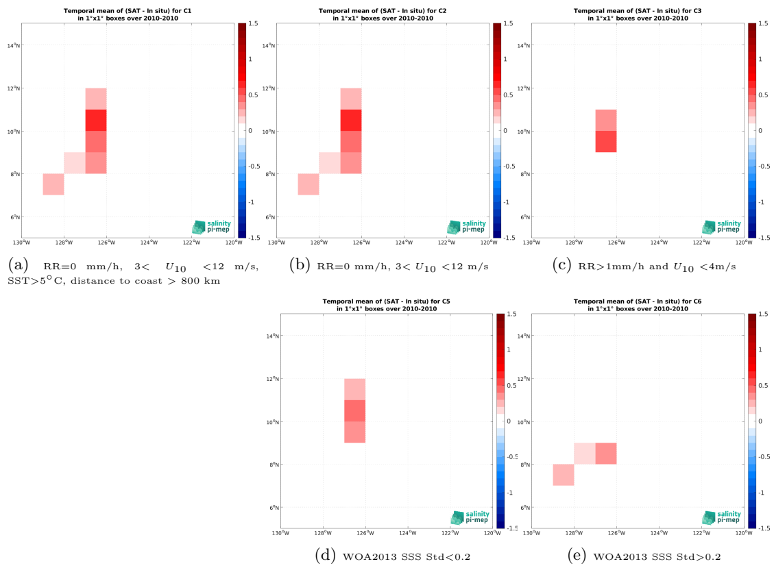
Figure 14: Temporal mean gridded over spatial boxes of size 1^\circ \times 1^\circ of \Delta SSS (CCI SSS L4 Merged-OI v5.5 - 7-day running (ESA) - TSG (GOSUD-Sailing-ship)) for 5 different subdatasets corresponding to:RR=0 mm/h, 3 < U_{10} < 12 m/s, SST >5^\circ C, distance to coast > 800 km (a), RR=0 mm/h, 3 < U_{10} < 12 m/s (b), RR >1 mm/h and U_{10} < 4 m/s (c), WOA2013 SSS Std <0.2 (d), WOA2013 SSS Std >0.2 (e).
