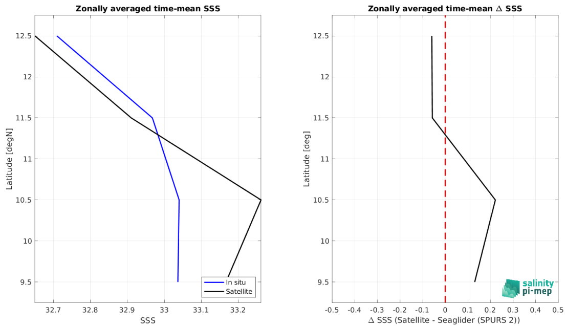
Figure 9: Left panel: Zonal mean SSS from CCI SSS L4 Merged-OI v5.5 - 7-day running (ESA) satellite product (black) and from Seaglider (SPURS 2) (blue). Right panel: Zonal mean of \Delta SSS (Satellite - Seaglider (SPURS 2)) for all the collected Pi-MEP match-up pairs estimated over the full satellite product period.
