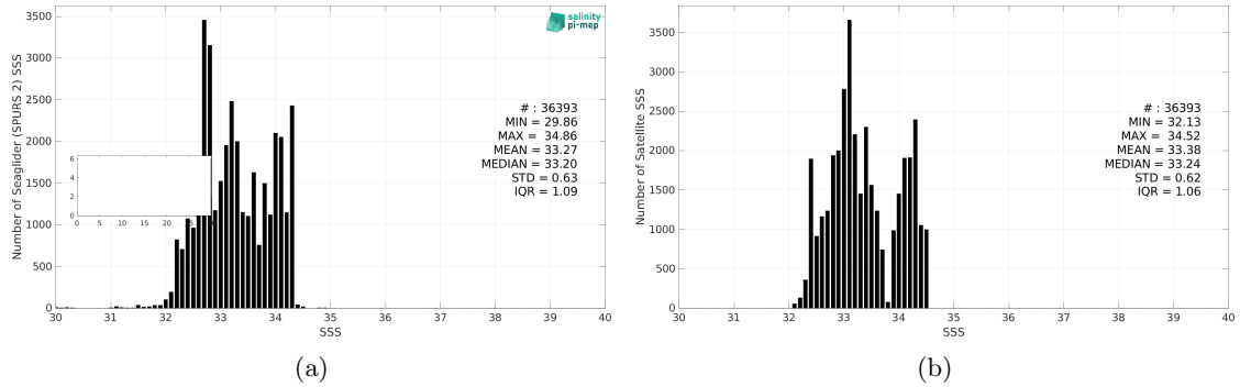
Figure 3: Histograms of SSS from Seaglider (SPURS 2) (a) and CCI SSS L4 Merged-OI v5.5 - 7-day running (ESA) (b) considering all match-up pairs per bins of 0.1 over the SPURS 2 Pi-MEP region and for the full satellite product period.
