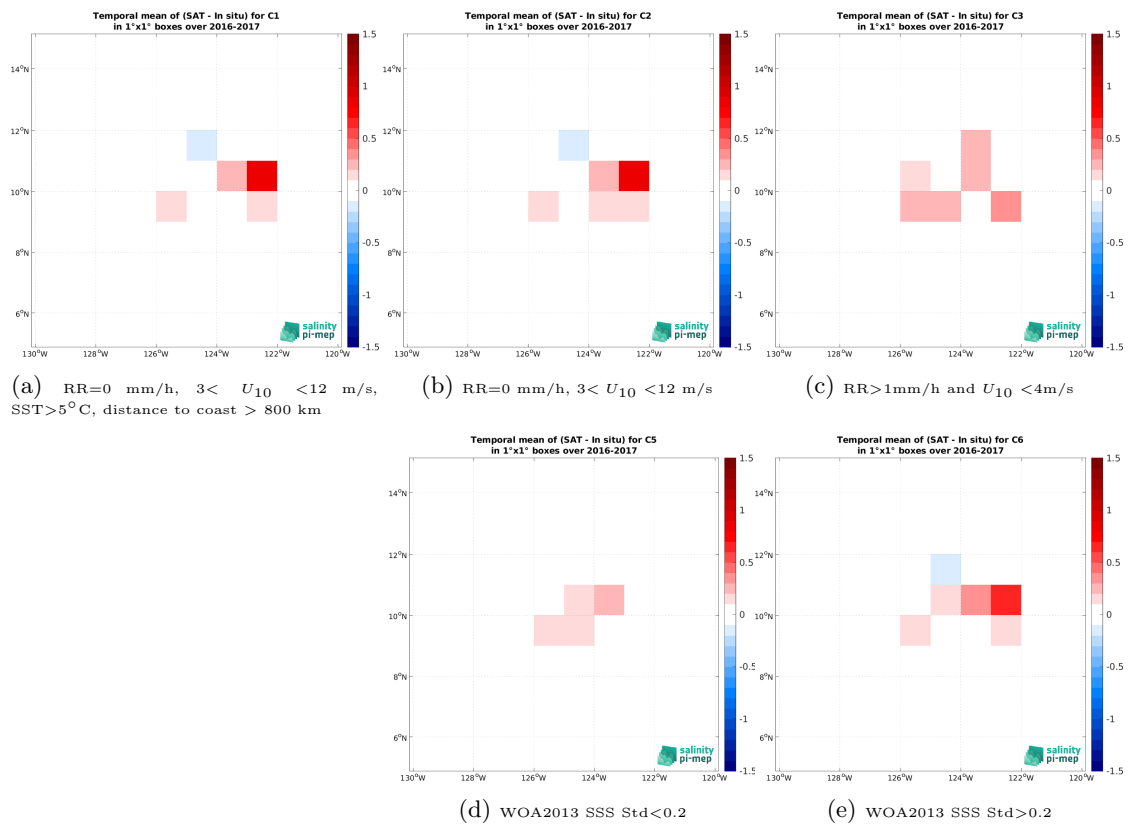
Figure 14: Temporal mean gridded over spatial boxes of size 1^\circ \times 1^\circ of \Delta SSS (CCI SSS L4 Merged-OI v5.5 - 7-day running (ESA) - Seaglider (SPURS 2)) for 5 different subdatasets corresponding to:RR=0 mm/h, 3 < U_{10} < 12 m/s, SST >5^\circ C, distance to coast > 800 km (a), RR=0 mm/h, 3 < U_{10} < 12 m/s (b), RR >1 mm/h and U_{10} < 4 m/s (c), WOA2013 SSS Std <0.2 (d), WOA2013 SSS Std >0.2 (e).
