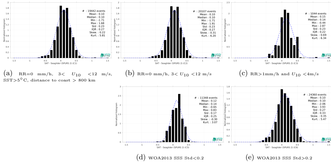
Figure 15: Normalized histogram of \Delta\text{SSS} (CCI SSS L4 Merged-OI v5.5 - 7-day running (ESA) - Seaglider (SPURS 2)) for 5 different subdatasets corresponding to: RR=0 mm/h, 3 < U_{10} < 12 m/s, SST>5°C, distance to coast > 800 km (a), RR=0 mm/h, 3 < U_{10} < 12 m/s (b), RR>1mm/h and U_{10} < 4 m/s (c), WOA2013 SSS Std<0.2 (d), WOA2013 SSS Std>0.2 (e).
