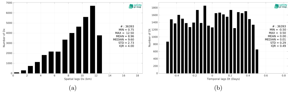
Figure 6: Histograms of the spatial (a) and temporal (b) lags between the location/time of the Seaglider (SPURS 2) measurement and the date of the corresponding CCI SSS L4 Merged-OI v5.5 - 7-day running (ESA) SSS pixel.
