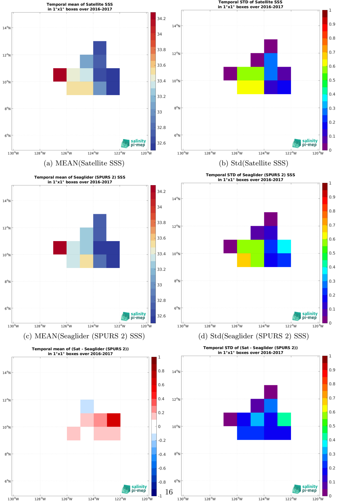
Figure 7: Temporal mean (left) and Std (right) of SSS from CCI SSS L4 Merged-OI v5.5 - 7-day running (ESA) (top), Seaglider (SPURS 2) (middle), and of \Delta SSS (Satellite - Seaglider (SPURS 2)). Only match-up pairs are used to generate these maps.
