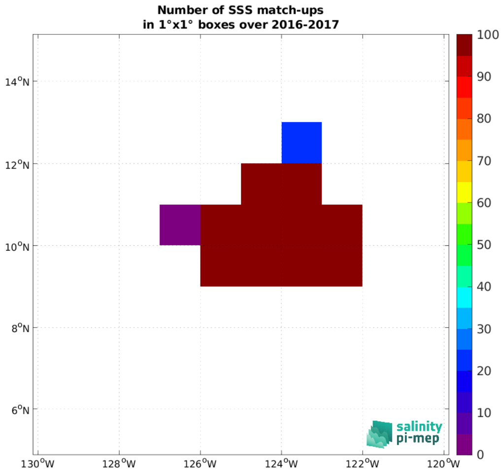
Figure 5: Number of SSS match-ups between Seaglider (SPURS 2) SSS and the CCI SSS L4 Merged-OI v5.5 - 7-day running (ESA) SSS product for the SPURS 2 Pi-MEP region over 1°x1° boxes and for the full satellite product period.
