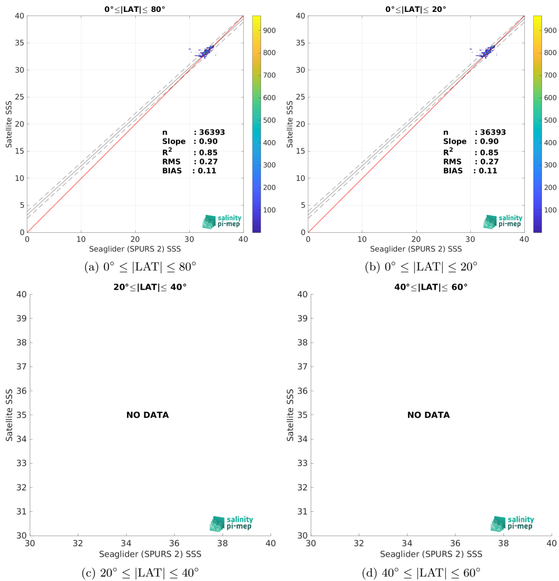
Figure 10: Contour maps of the concentration of CCI SSS L4 Merged-OI v5.5 - 7-day running (ESA) SSS (y-axis) versus Seaglider (SPURS 2) SSS (x-axis) at match-up pairs for different latitude bands. For each plot, the red line shows x=y . The black thin and dashed lines indicate a linear fit through the data cloud and the \pm 95\% confidence levels, respectively. The number match-up pairs n , the slope and R^2 coefficient of the linear fit, the root mean square (RMS) and the mean bias between satellite and in situ data are indicated for each latitude band in each plots.
