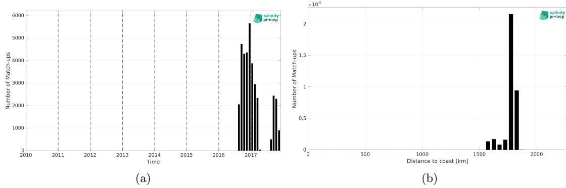
Figure 2: Number of match-ups between Seaglider (SPURS 2) and CCI SSS L4 Merged-OI v5.5 - 7-day running (ESA) SSS as a function of time (a) and as function of the distance to coast (b) over the SPURS 2 Pi-MEP region and for the full satellite product period.
