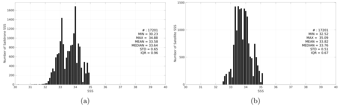
Figure 3: Histograms of SSS from Saildrone (a) and CCI SSS L4 Merged-OI v5.5 - 7-day running (ESA) (b) considering all match-up pairs per bins of 0.1 over the SPURS 2 Pi-MEP region and for the full satellite product period.
