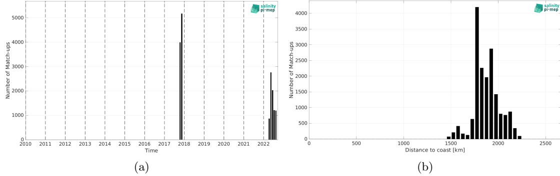
Figure 2: Number of match-ups between Saildrone and CCI SSS L4 Merged-OI v5.5 - 7-day running (ESA) SSS as a function of time (a) and as function of the distance to coast (b) over the SPURS 2 Pi-MEP region and for the full satellite product period.
