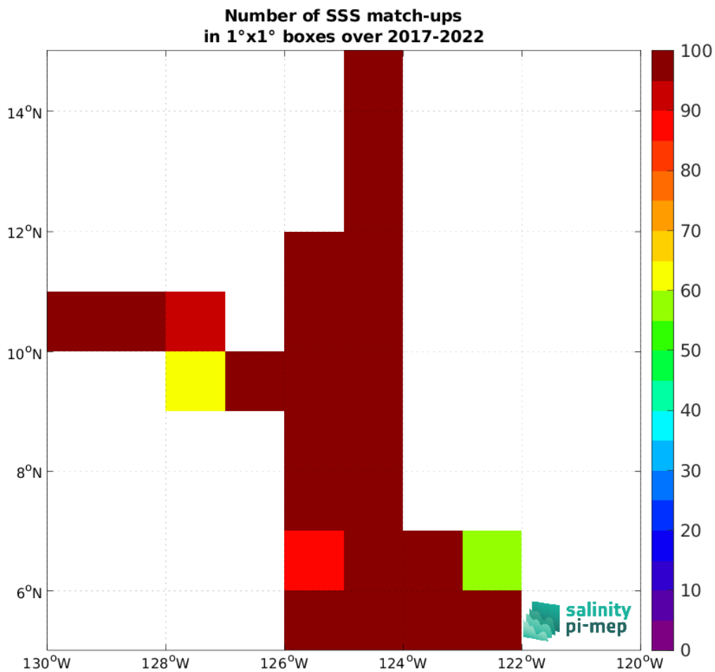
Figure 5: Number of SSS match-ups between Saildrone SSS and the CCI SSS L4 Merged-OI v5.5 - 7-day running (ESA) SSS product for the SPURS 2 Pi-MEP region over 1°x1° boxes and for the full satellite product period.
