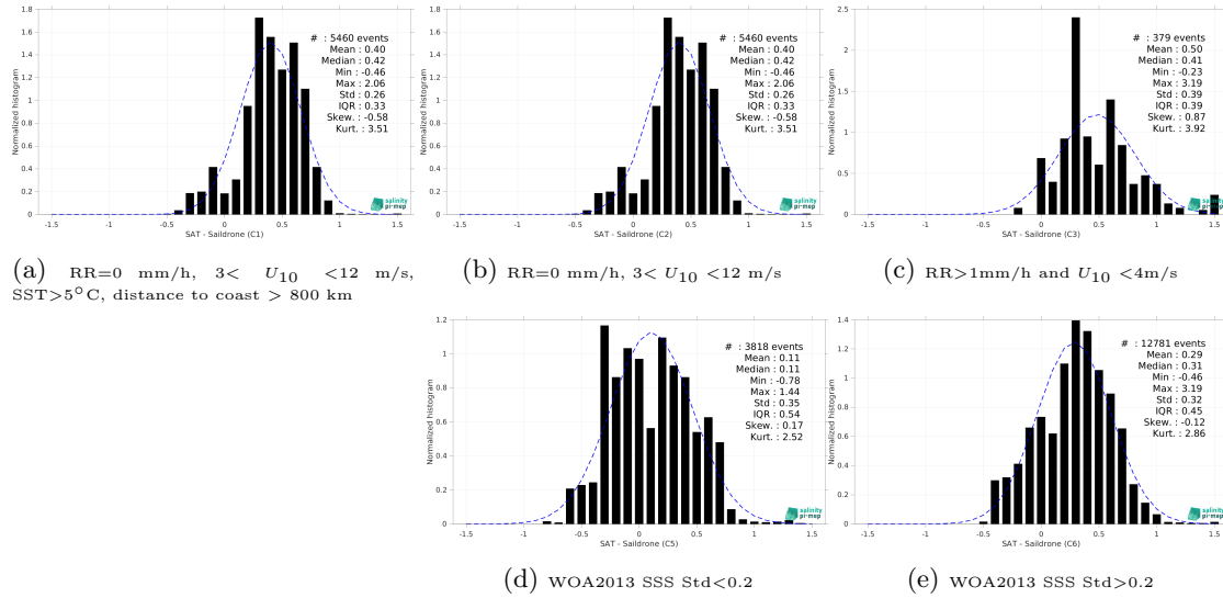
Figure 15: Normalized histogram of \Delta\text{SSS} (CCI SSS L4 Merged-OI v5.5 - 7-day running (ESA) - Saildrone) for 5 different subdatasets corresponding to: RR=0 mm/h, 3 < U_{10} < 12 m/s, SST>5°C, distance to coast > 800 km (a), RR=0 mm/h, 3 < U_{10} < 12 m/s (b), RR>1mm/h and U_{10} < 4 m/s (c), WOA2013 SSS Std<0.2 (d), WOA2013 SSS Std>0.2 (e).
