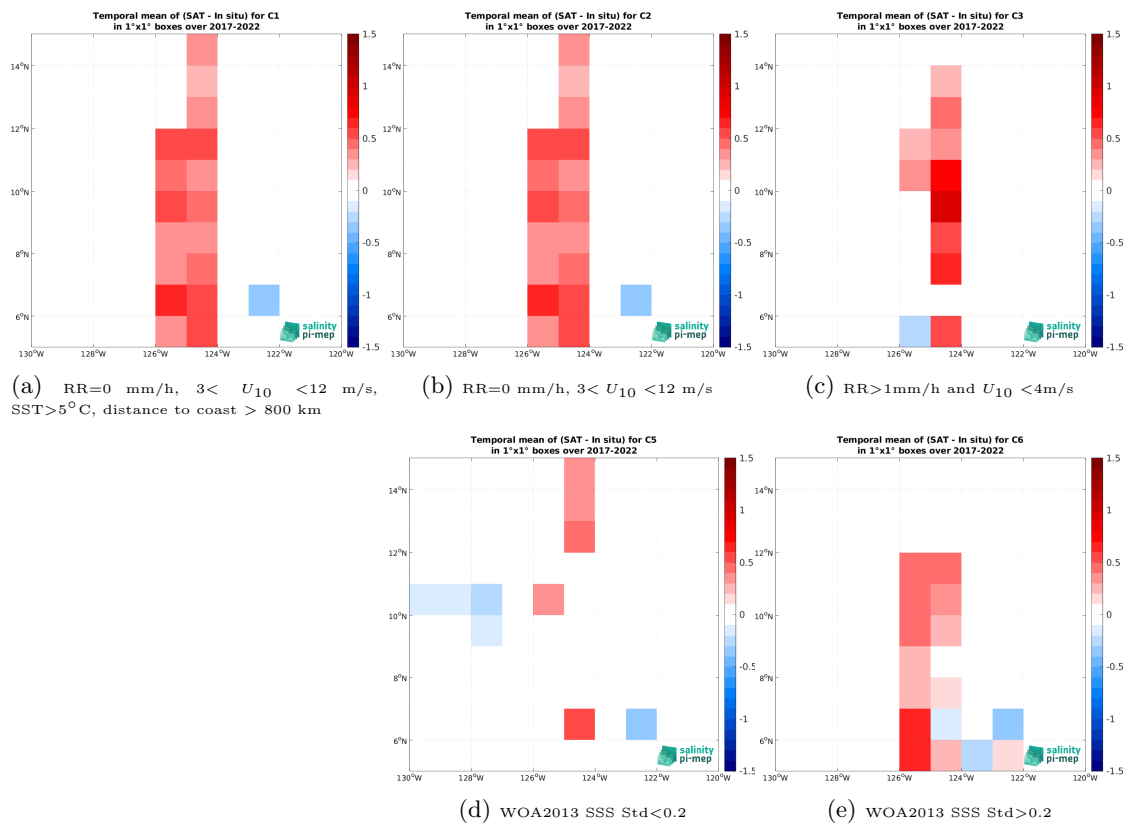
Figure 14: Temporal mean gridded over spatial boxes of size 1^\circ \times 1^\circ of \Delta\text{SSS} (CCI SSS L4 Merged-OI v5.5 - 7-day running (ESA) - Sairdrone) for 5 different subdatasets corresponding to:RR=0 mm/h, 3 < U_{10} < 12 m/s, SST>5°C, distance to coast > 800 km (a), RR=0 mm/h, 3 < U_{10} < 12 m/s (b), RR>1mm/h and U_{10} < 4 m/s (c), WOA2013 SSS Std<0.2 (d), WOA2013 SSS Std>0.2 (e).
