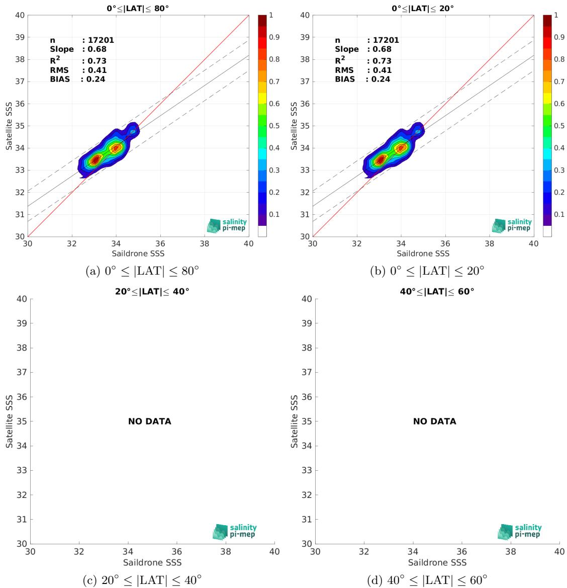
Figure 10: Contour maps of the concentration of CCI SSS L4 Merged-OI v5.5 - 7-day running (ESA) SSS (y-axis) versus Saildrone SSS (x-axis) at match-up pairs for different latitude bands. For each plot, the red line shows x=y . The black thin and dashed lines indicate a linear fit through the data cloud and the \pm 95\% confidence levels, respectively. The number match-up pairs n , the slope and R^2 coefficient of the linear fit, the root mean square (RMS) and the mean bias between satellite and in situ data are indicated for each latitude band in each plots.
