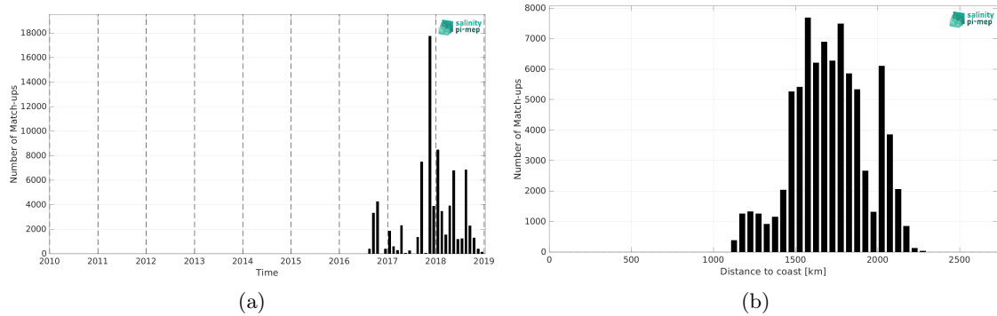
Figure 2: Number of match-ups between Surface drifters and CCI SSS L4 Merged-OI v5.5 - 7-day running (ESA) SSS as a function of time (a) and as function of the distance to coast (b) over the SPURS 2 Pi-MEP region and for the full satellite product period.
