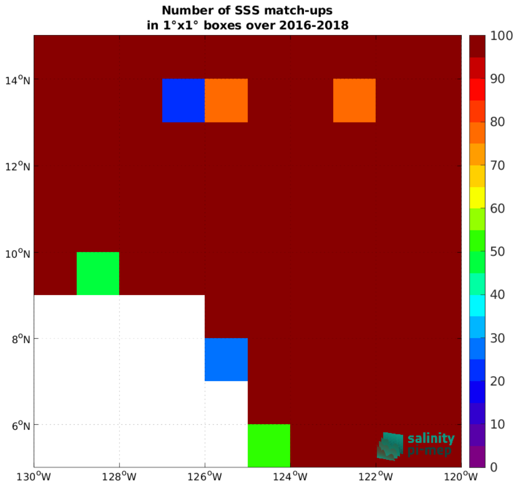
Figure 4: Number of SSS match-ups between Surface drifters SSS and the CCI SSS L4 Merged-OI v5.5 - 7-day running (ESA) SSS product for the SPURS 2 Pi-MEP region over 1°x1° boxes and for the full satellite product period.
