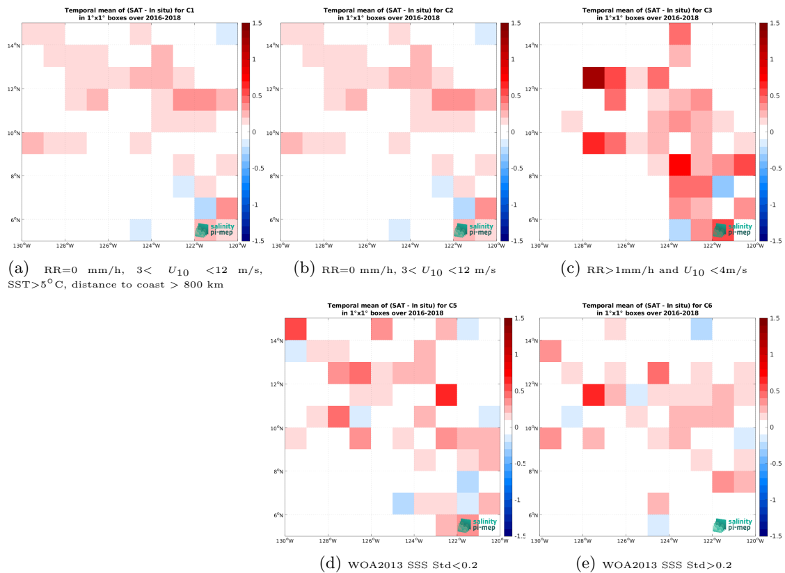
Figure 13: Temporal mean gridded over spatial boxes of size 1^\circ \times 1^\circ of \Delta SSS (CCI SSS L4 Merged-OI v5.5 - 7-day running (ESA) - Surface drifters) for 5 different subdatasets corresponding to:RR=0 mm/h, 3 < U_{10} < 12 m/s, SST >5^\circ C, distance to coast > 800 km (a), RR=0 mm/h, 3 < U_{10} < 12 m/s (b), RR >1 mm/h and U_{10} < 4 m/s (c), WOA2013 SSS Std <0.2 (d), WOA2013 SSS Std >0.2 (e).
