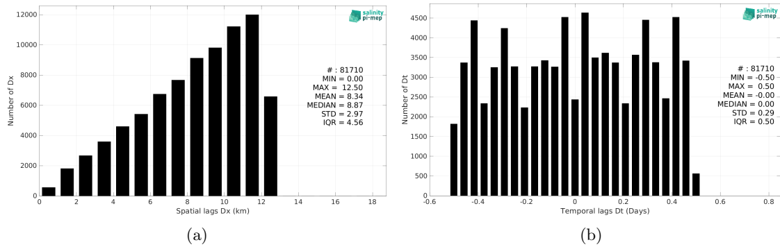
Figure 5: Histograms of the spatial (a) and temporal (b) lags between the location/time of the Surface drifters measurement and the date of the corresponding CCI SSS L4 Merged-OI v5.5 - 7-day running (ESA) SSS pixel.
