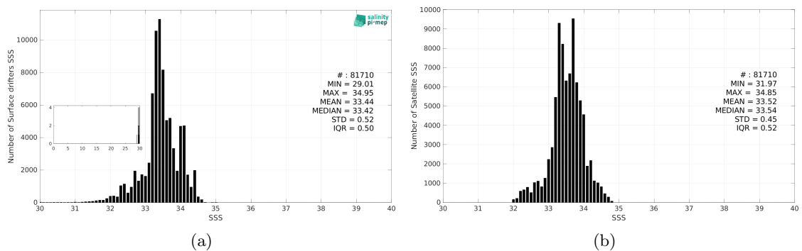
Figure 3: Histograms of SSS from Surface drifters (a) and CCI SSS L4 Merged-OI v5.5 - 7-day running (ESA) (b) considering all match-up pairs per bins of 0.1 over the SPURS 2 Pi-MEP region and for the full satellite product period.
