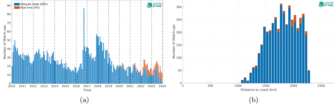
Figure 2: Number of match-ups between Argo and CCI SSS L4 Merged-OI v5.5 - 7-day running (ESA) SSS as a function of time (a) and as function of the distance to coast (b) over the SPURS 2 Pi-MEP region and for the full satellite product period.
