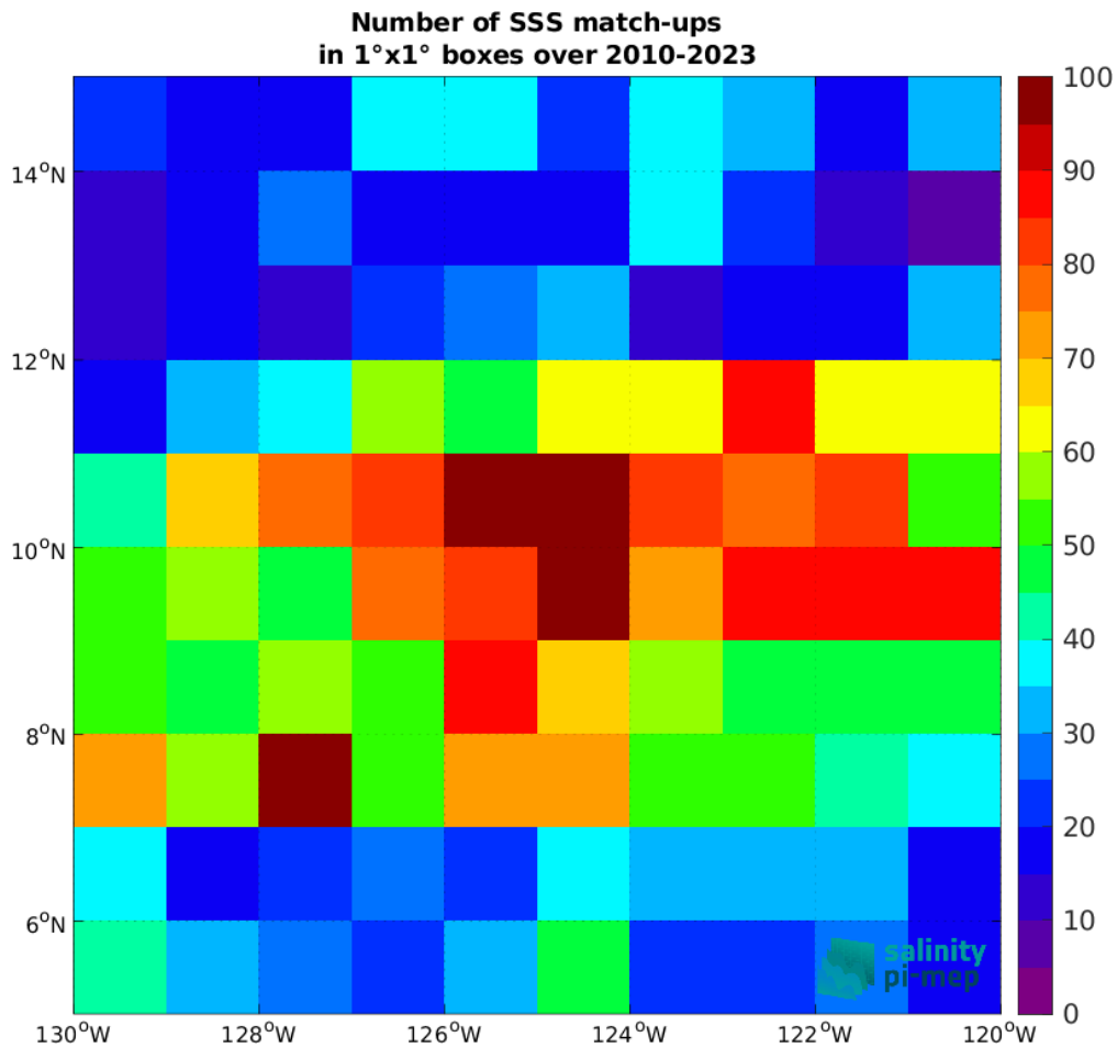
Figure 5: Number of SSS match-ups between Argo SSS and the CCI SSS L4 Merged-OI v5.5 - 7-day running (ESA) SSS product for the SPURS 2 Pi-MEP region over 1°x1° boxes and for the full satellite product period.
