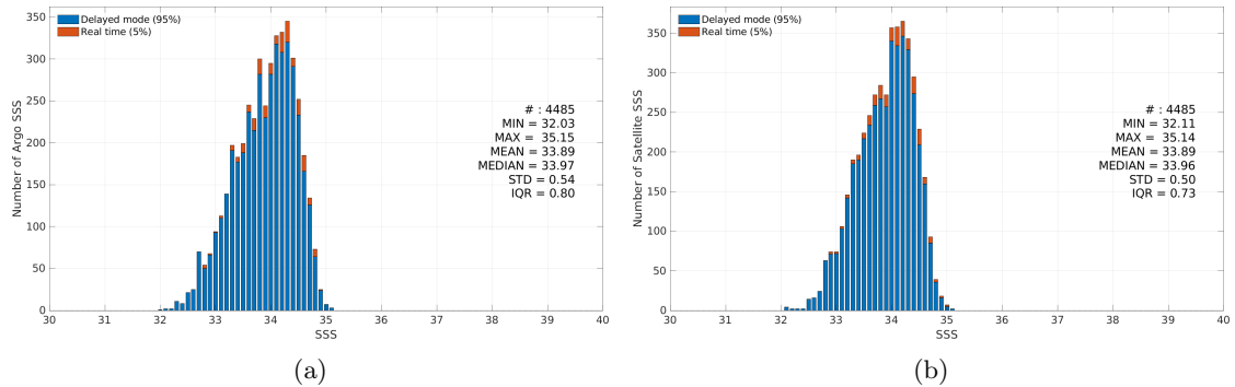
Figure 3: Histograms of SSS from Argo (a) and CCI SSS L4 Merged-OI v5.5 - 7-day running (ESA) (b) considering all match-up pairs per bins of 0.1 over the SPURS 2 Pi-MEP region and for the full satellite product period.
