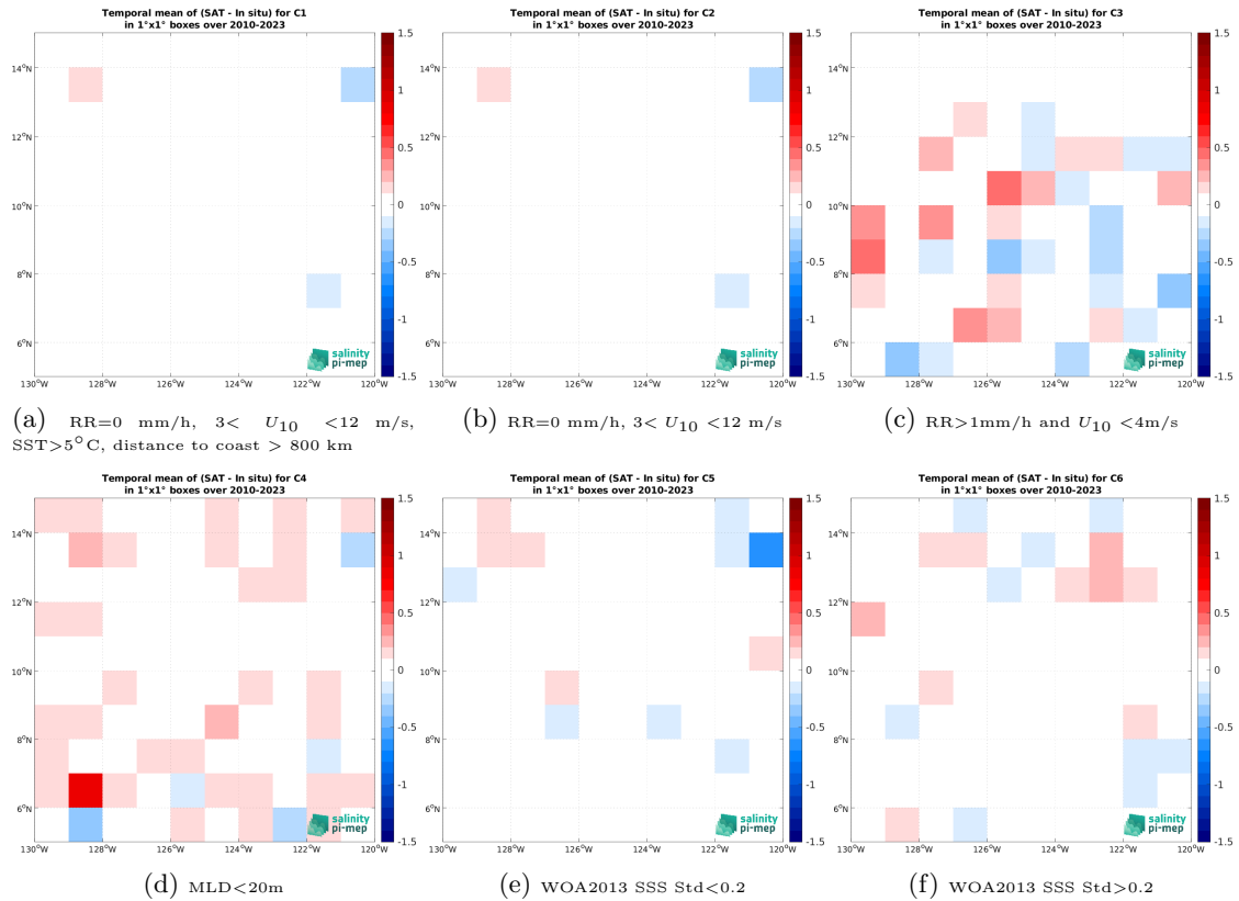
Figure 14: Temporal mean gridded over spatial boxes of size 1^\circ \times 1^\circ of \Delta SSS (CCI SSS L4 Merged-OI v5.5 - 7-day running (ESA) - Argo) for 6 different subdatasets corresponding to:RR=0 mm/h, 3 < U_{10} < 12 m/s, SST >5^\circ C, distance to coast > 800 km (a), RR=0 mm/h, 3 < U_{10} < 12 m/s (b), RR >1 mm/h and U_{10} < 4 m/s (c),MLD <20 m (d),WOA2013 SSS Std <0.2 (e),WOA2013 SSS Std >0.2 (f).
