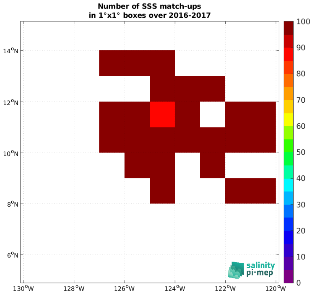
Figure 5: Number of SSS match-ups between Waveglider (SPURS 2) SSS and the CCI SSS L4 Merged-OI v5.5 - 30-day running (ESA) SSS product for the SPURS 2 Pi-MEP region over 1^\circ \times 1^\circ boxes and for the full satellite product period.
