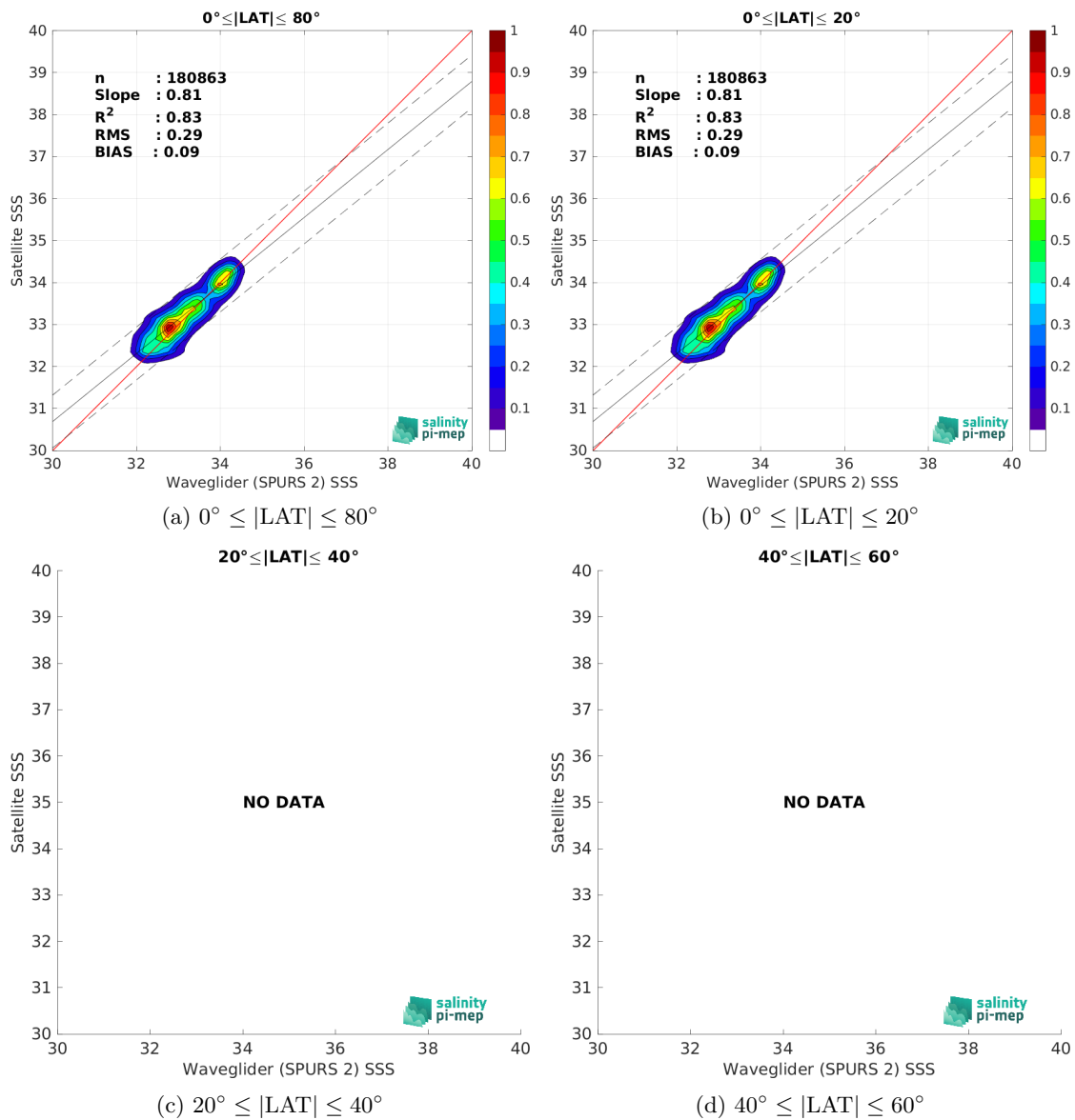
Figure 10: Contour maps of the concentration of CCI SSS L4 Merged-OI v5.5 - 30-day running (ESA) SSS (y-axis) versus Waveglider (SPURS 2) SSS (x-axis) at match-up pairs for different latitude bands. For each plot, the red line shows x=y . The black thin and dashed lines indicate a linear fit through the data cloud and the \pm 95\% confidence levels, respectively. The number match-up pairs n , the slope and R^2 coefficient of the linear fit, the root mean square (RMS) and the mean bias between satellite and in situ data are indicated for each latitude band in each plots.
