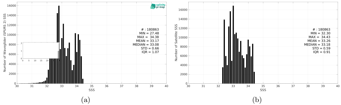
Figure 3: Histograms of SSS from Waveglider (SPURS 2) (a) and CCI SSS L4 Merged-OI v5.5 - 30-day running (ESA) (b) considering all match-up pairs per bins of 0.1 over the SPURS 2 Pi-MEP region and for the full satellite product period.
