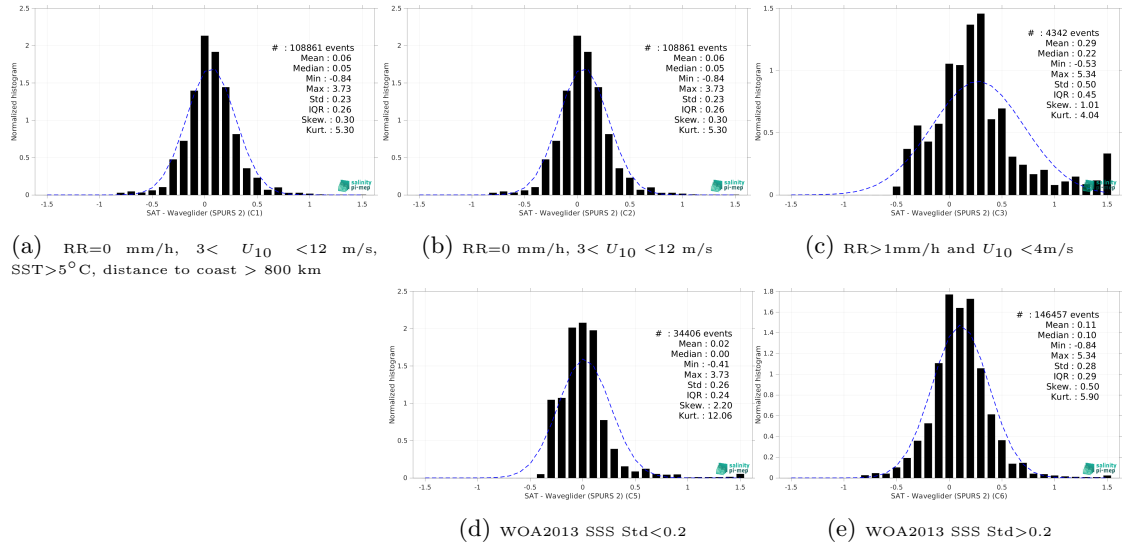
Figure 15: Normalized histogram of \Delta SSS (CCI SSS L4 Merged-OI v5.5 - 30-day running (ESA) - Waveglider (SPURS 2)) for 5 different subdatasets corresponding to: RR=0 mm/h, 3 < U_{10} < 12 m/s, SST>5°C, distance to coast > 800 km (a), RR=0 mm/h, 3 < U_{10} < 12 m/s (b), RR>1mm/h and U_{10} < 4 m/s (c), WOA2013 SSS Std<0.2 (d), WOA2013 SSS Std>0.2 (e).
