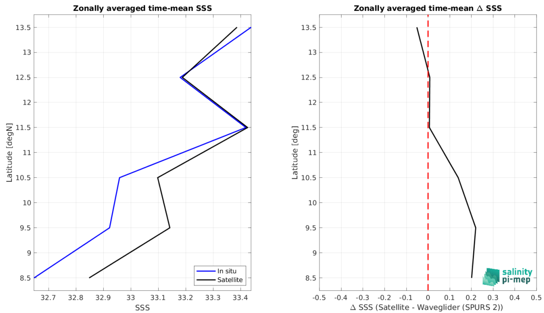
Figure 9: Left panel: Zonal mean SSS from CCI SSS L4 Merged-OI v5.5 - 30-day running (ESA) satellite product (black) and from Waveglider (SPURS 2) (blue). Right panel: Zonal mean of \Delta SSS (Satellite - Waveglider (SPURS 2)) for all the collected Pi-MEP match-up pairs estimated over the full satellite product period.
