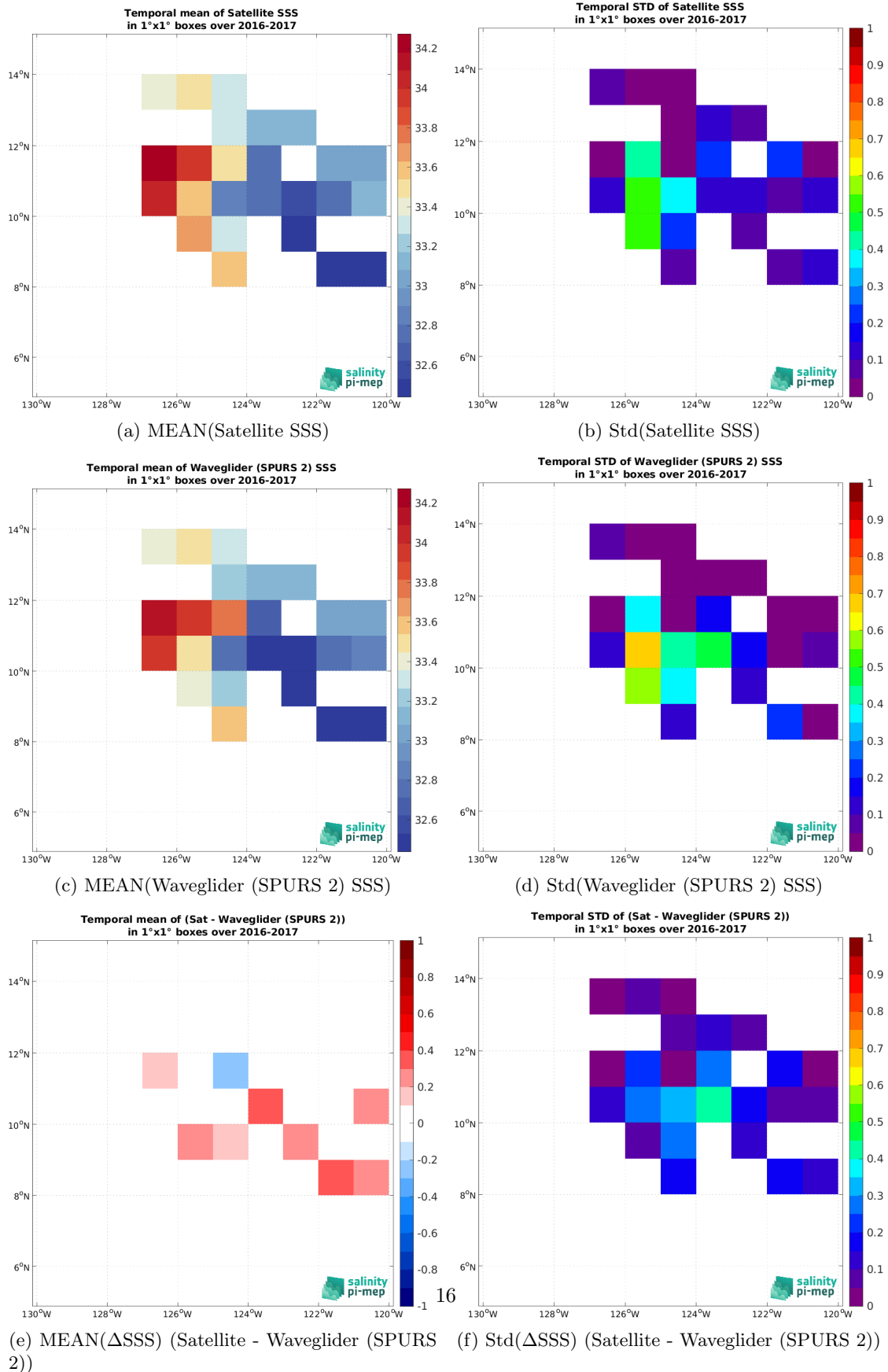
Figure 7: Temporal mean (left) and Std (right) of SSS from CCI SSS L4 Merged-OI v5.5 - 30-day running (ESA) (top), Waveglider (SPURS 2) (middle), and of \Delta SSS (Satellite - Waveglider (SPURS 2)). Only match-up pairs are used to generate these maps.
