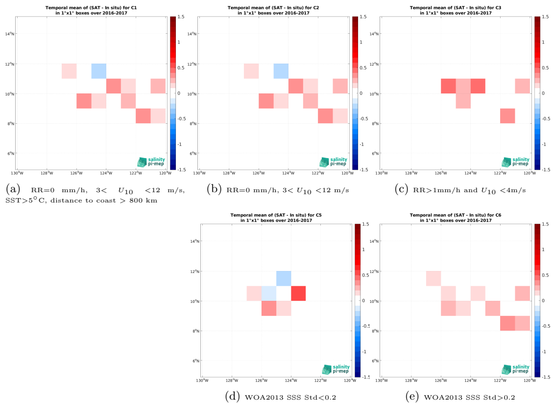
Figure 14: Temporal mean gridded over spatial boxes of size 1^\circ \times 1^\circ of \Delta SSS (CCI SSS L4 Merged-OI v5.5 - 30-day running (ESA) - Waveglider (SPURS 2)) for 5 different subdatasets corresponding to:RR=0 mm/h, 3 < U_{10} < 12 m/s, SST >5^\circ C, distance to coast > 800 km (a), RR=0 mm/h, 3 < U_{10} < 12 m/s (b), RR >1 mm/h and U_{10} < 4 m/s (c), WOA2013 SSS Std <0.2 (d), WOA2013 SSS Std >0.2 (e).
