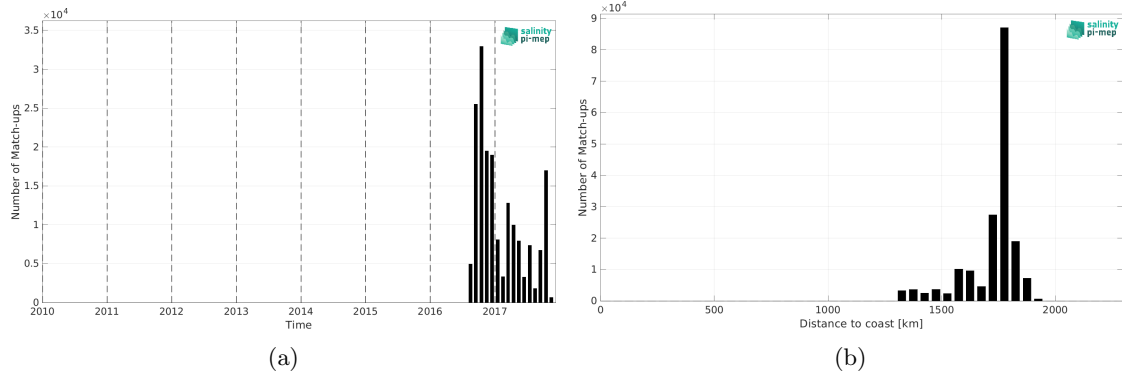
Figure 2: Number of match-ups between Waveglider (SPURS 2) and CCI SSS L4 Merged-OI v5.5 - 30-day running (ESA) SSS as a function of time (a) and as function of the distance to coast (b) over the SPURS 2 Pi-MEP region and for the full satellite product period.
