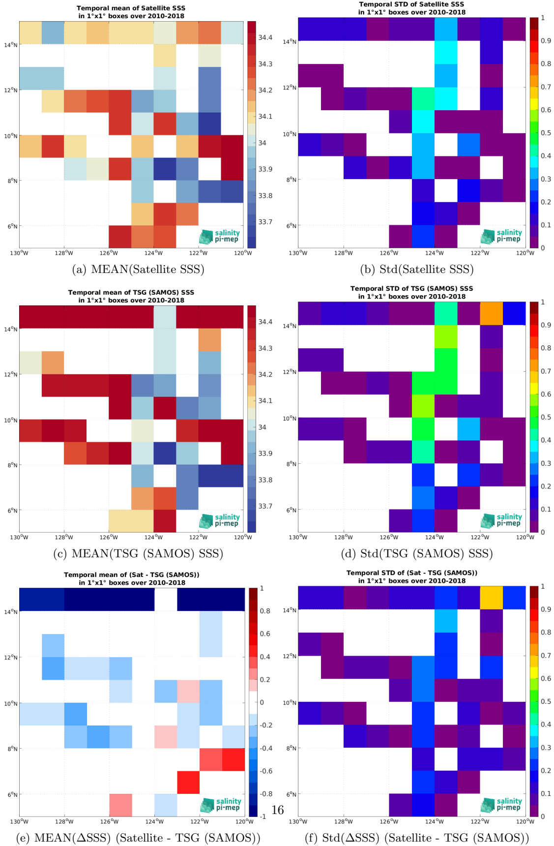
Figure 7: Temporal mean (left) and Std (right) of SSS from CCI SSS L4 Merged-OI v5.5 - 30-day running (ESA) (top), TSG (SAMOS) (middle), and of \Delta SSS (Satellite - TSG (SAMOS)). Only match-up pairs are used to generate these maps.
