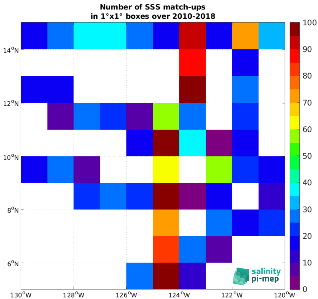
Figure 5: Number of SSS match-ups between TSG (SAMOS) SSS and the CCI SSS L4 Merged-OI v5.5 - 30-day running (ESA) SSS product for the SPURS 2 Pi-MEP region over 1°x1° boxes and for the full satellite product period.
