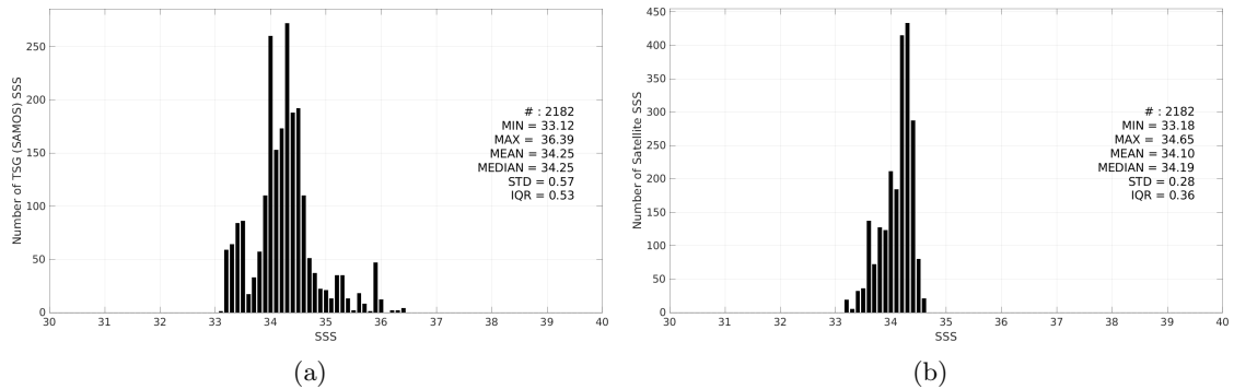
Figure 3: Histograms of SSS from TSG (SAMOS) (a) and CCI SSS L4 Merged-OI v5.5 - 30-day running (ESA) (b) considering all match-up pairs per bins of 0.1 over the SPURS 2 Pi-MEP region and for the full satellite product period.
