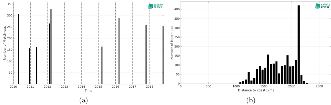
Figure 2: Number of match-ups between TSG (SAMOS) and CCI SSS L4 Merged-OI v5.5 - 30-day running (ESA) SSS as a function of time (a) and as function of the distance to coast (b) over the SPURS 2 Pi-MEP region and for the full satellite product period.
