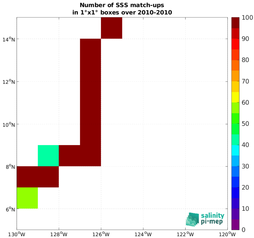
Figure 5: Number of SSS match-ups between TSG (GOSUD-Sailing-ship) SSS and the CCI SSS L4 Merged-OI v5.5 - 30-day running (ESA) SSS product for the SPURS 2 Pi-MEP region over 1^\circ \times 1^\circ boxes and for the full satellite product period.
