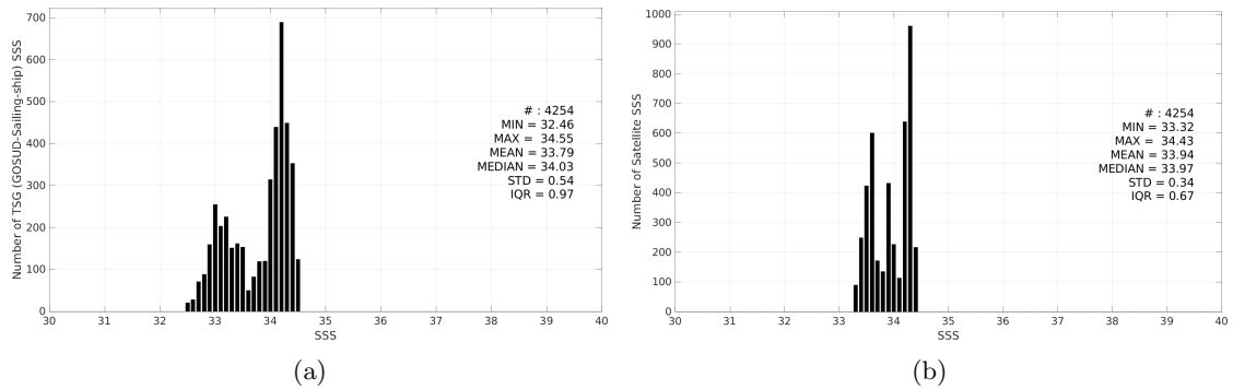
Figure 3: Histograms of SSS from TSG (GOSUD-Sailing-ship) (a) and CCI SSS L4 Merged-OI v5.5 - 30-day running (ESA) (b) considering all match-up pairs per bins of 0.1 over the SPURS 2 Pi-MEP region and for the full satellite product period.
