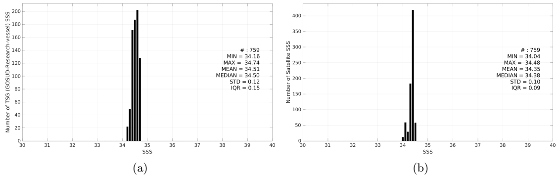
Figure 3: Histograms of SSS from TSG (GOSUD-Research-vessel) (a) and CCI SSS L4 Merged-OI v5.5 - 30-day running (ESA) (b) considering all match-up pairs per bins of 0.1 over the SPURS 2 Pi-MEP region and for the full satellite product period.
