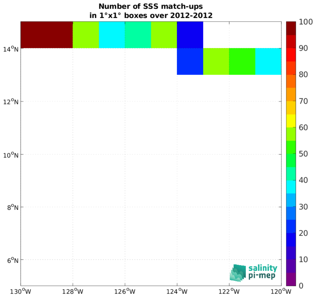
Figure 5: Number of SSS match-ups between TSG (GOSUD-Research-vessel) SSS and the CCI SSS L4 Merged-OI v5.5 - 30-day running (ESA) SSS product for the SPURS 2 Pi-MEP region over 1^\circ \times 1^\circ boxes and for the full satellite product period.
