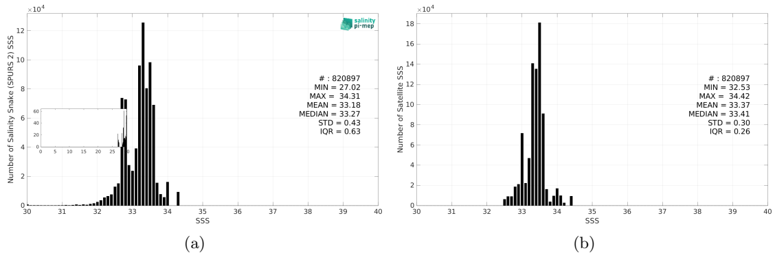
Figure 3: Histograms of SSS from Salinity Snake (SPURS 2) (a) and CCI SSS L4 Merged-OI v5.5 - 30-day running (ESA) (b) considering all match-up pairs per bins of 0.1 over the SPURS 2 Pi-MEP region and for the full satellite product period.
