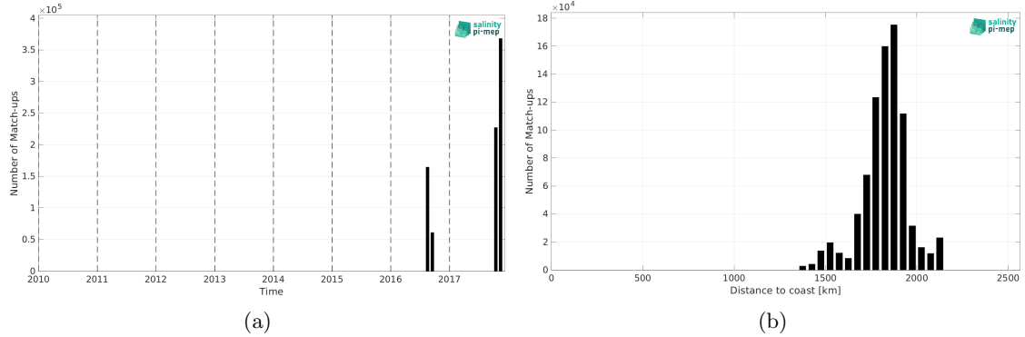
Figure 2: Number of match-ups between Salinity Snake (SPURS 2) and CCI SSS L4 Merged-OI v5.5 - 30-day running (ESA) SSS as a function of time (a) and as function of the distance to coast (b) over the SPURS 2 Pi-MEP region and for the full satellite product period.
