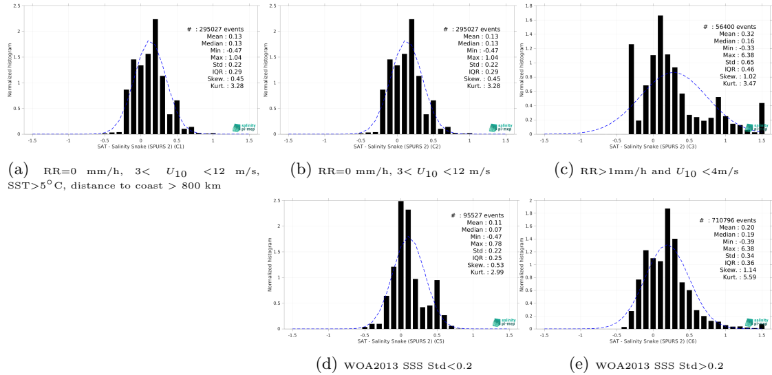
Figure 15: Normalized histogram of \Delta SSS (CCI SSS L4 Merged-OI v5.5 - 30-day running (ESA) - Salinity Snake (SPURS 2)) for 5 different subdatasets corresponding to: RR=0 mm/h, 3 < U_{10} < 12 m/s, SST>5°C, distance to coast > 800 km (a), RR=0 mm/h, 3 < U_{10} < 12 m/s (b), RR>1mm/h and U_{10} < 4 m/s (c), WOA2013 SSS Std<0.2 (d), WOA2013 SSS Std>0.2 (e).
