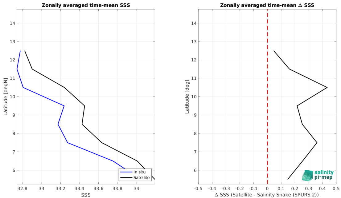
Figure 9: Left panel: Zonal mean SSS from CCI SSS L4 Merged-OI v5.5 - 30-day running (ESA) satellite product (black) and from Salinity Snake (SPURS 2) (blue). Right panel: Zonal mean of \Delta SSS (Satellite - Salinity Snake (SPURS 2)) for all the collected Pi-MEP match-up pairs estimated over the full satellite product period.
