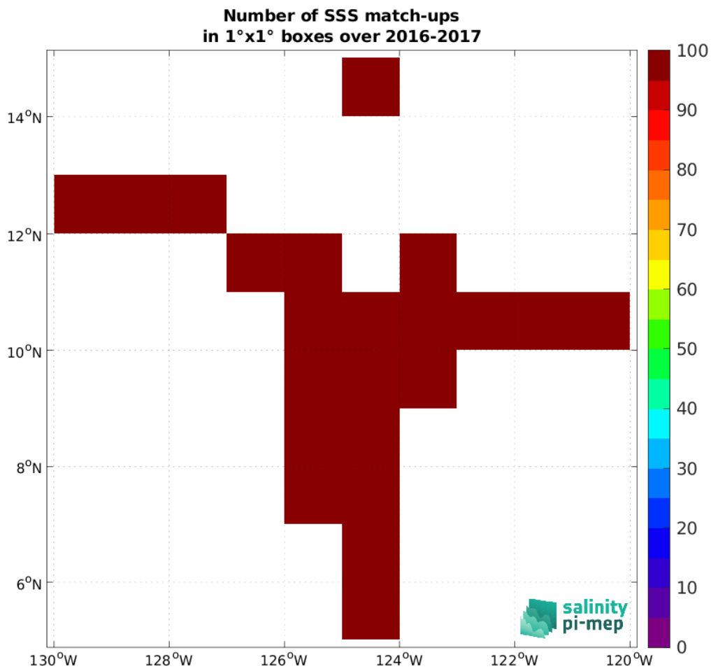
Figure 5: Number of SSS match-ups between Salinity Snake (SPURS 2) SSS and the CCI SSS L4 Merged-OI v5.5 - 30-day running (ESA) SSS product for the SPURS 2 Pi-MEP region over 1^\circ \times 1^\circ boxes and for the full satellite product period.
