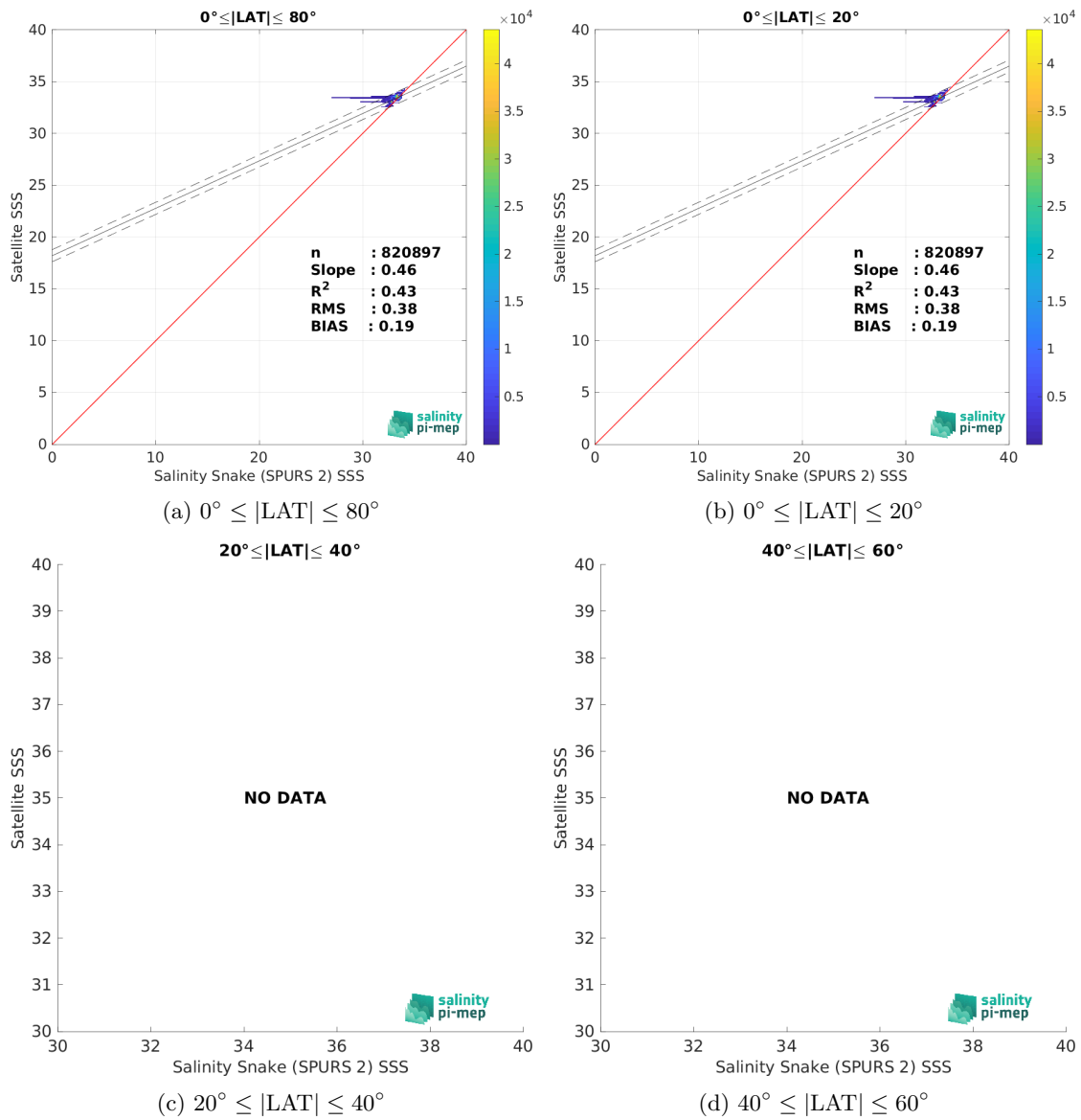
Figure 10: Contour maps of the concentration of CCI SSS L4 Merged-OI v5.5 - 30-day running (ESA) SSS (y-axis) versus Salinity Snake (SPURS 2) SSS (x-axis) at match-up pairs for different latitude bands. For each plot, the red line shows x=y . The black thin and dashed lines indicate a linear fit through the data cloud and the \pm 95\% confidence levels, respectively. The number match-up pairs n , the slope and R^2 coefficient of the linear fit, the root mean square (RMS) and the mean bias between satellite and in situ data are indicated for each latitude band in each plots.
