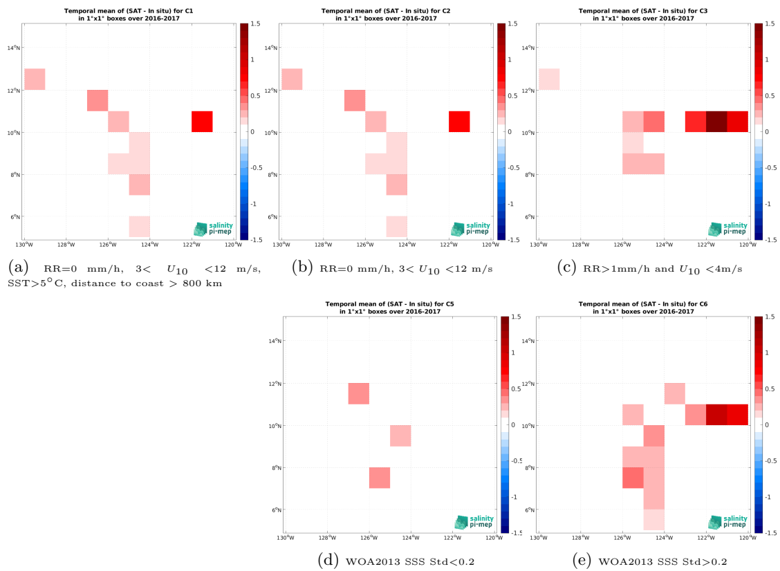
Figure 14: Temporal mean gridded over spatial boxes of size 1^\circ \times 1^\circ of \Delta\text{SSS} (CCI SSS L4 Merged-OI v5.5 - 30-day running (ESA) - Salinity Snake (SPURS 2)) for 5 different subdatasets corresponding to:RR=0 mm/h, 3 < U_{10} < 12 m/s, SST >5^\circ\text{C} , distance to coast > 800 km (a), RR=0 mm/h, 3 < U_{10} < 12 m/s (b), RR >1 mm/h and U_{10} < 4 m/s (c), WOA2013 SSS Std <0.2 (d), WOA2013 SSS Std >0.2 (e).
