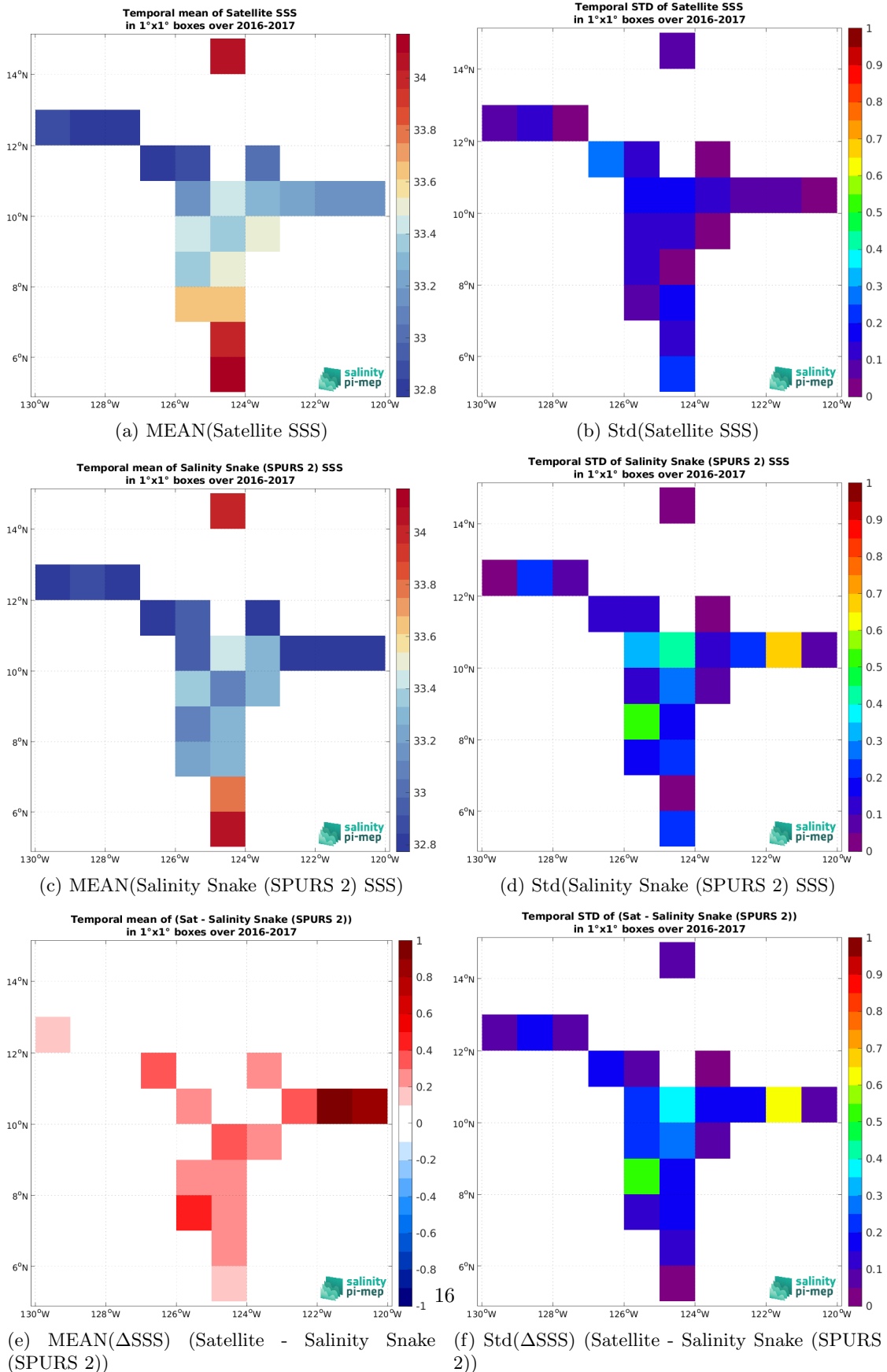
Figure 7: Temporal mean (left) and Std (right) of SSS from CCI SSS L4 Merged-OI v5.5 - 30-day running (ESA) (top), Salinity Snake (SPURS 2) (middle), and of \Delta SSS (Satellite - Salinity Snake (SPURS 2)). Only match-up pairs are used to generate these maps.
