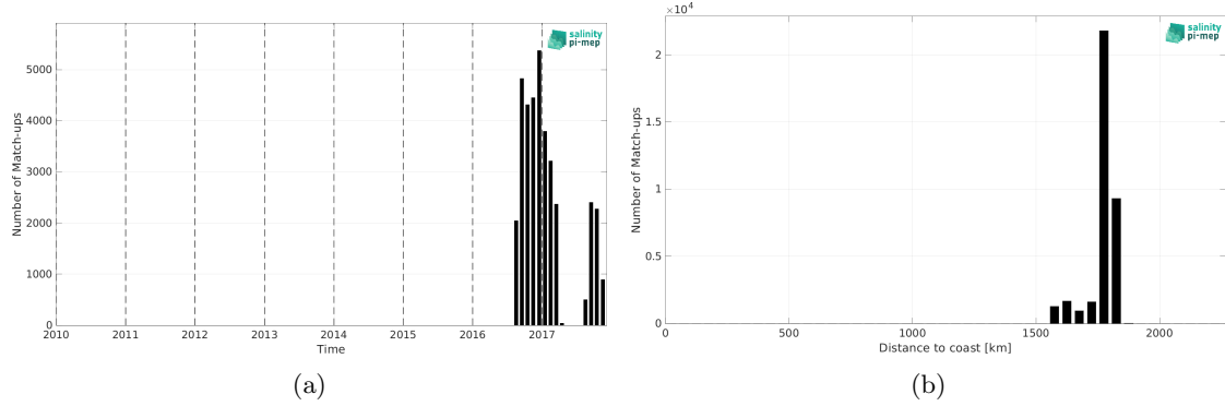
Figure 2: Number of match-ups between Seaglider (SPURS 2) and CCI SSS L4 Merged-OI v5.5 - 30-day running (ESA) SSS as a function of time (a) and as function of the distance to coast (b) over the SPURS 2 Pi-MEP region and for the full satellite product period.
