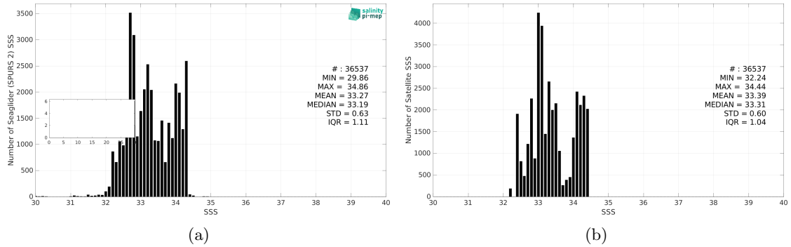
Figure 3: Histograms of SSS from Seaglider (SPURS 2) (a) and CCI SSS L4 Merged-OI v5.5 - 30-day running (ESA) (b) considering all match-up pairs per bins of 0.1 over the SPURS 2 Pi-MEP region and for the full satellite product period.
