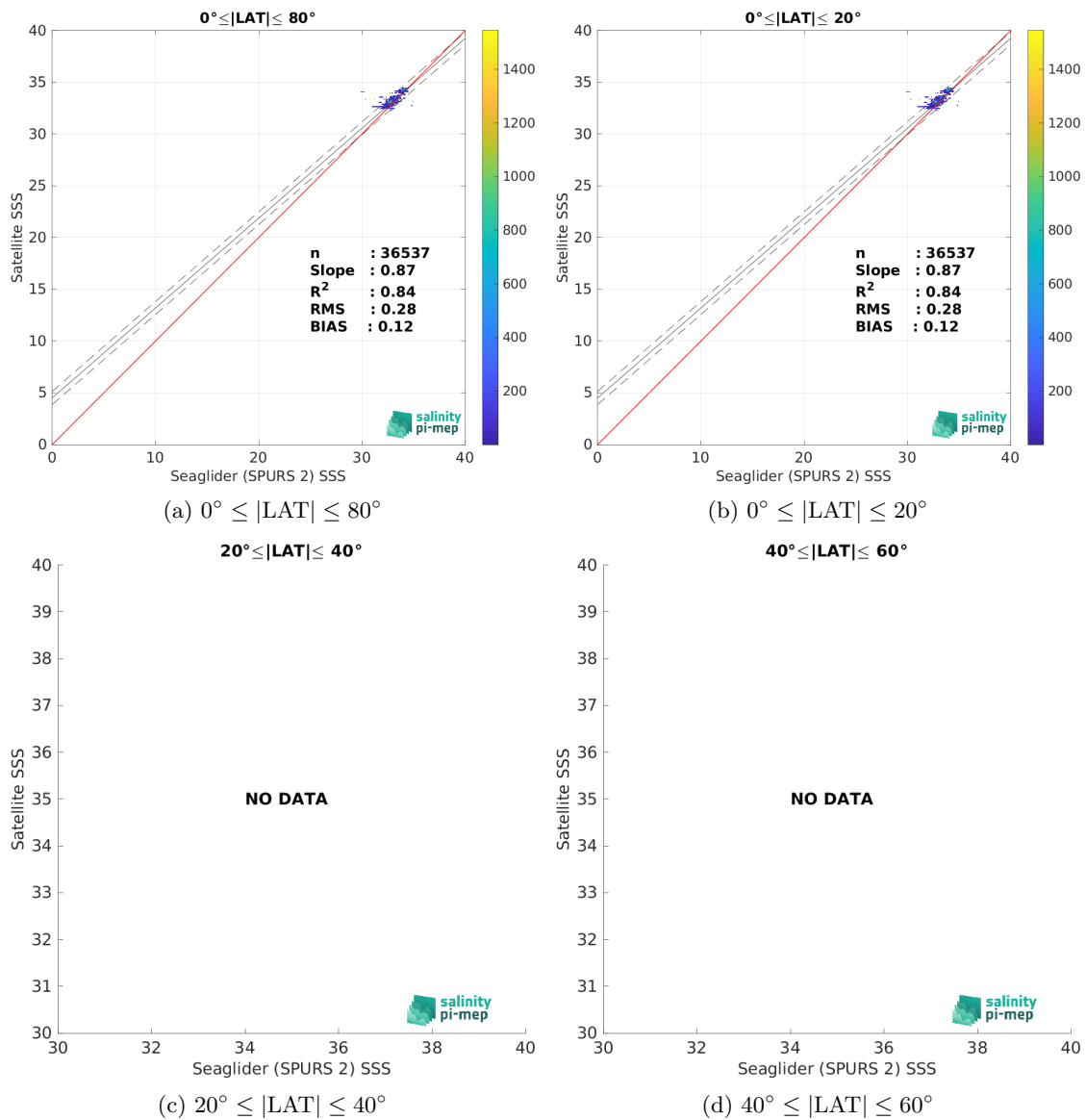
Figure 10: Contour maps of the concentration of CCI SSS L4 Merged-OI v5.5 - 30-day running (ESA) SSS (y-axis) versus Seaglider (SPURS 2) SSS (x-axis) at match-up pairs for different latitude bands. For each plot, the red line shows x=y . The black thin and dashed lines indicate a linear fit through the data cloud and the \pm 95\% confidence levels, respectively. The number match-up pairs n , the slope and R^2 coefficient of the linear fit, the root mean square (RMS) and the mean bias between satellite and in situ data are indicated for each latitude band in each plots.
