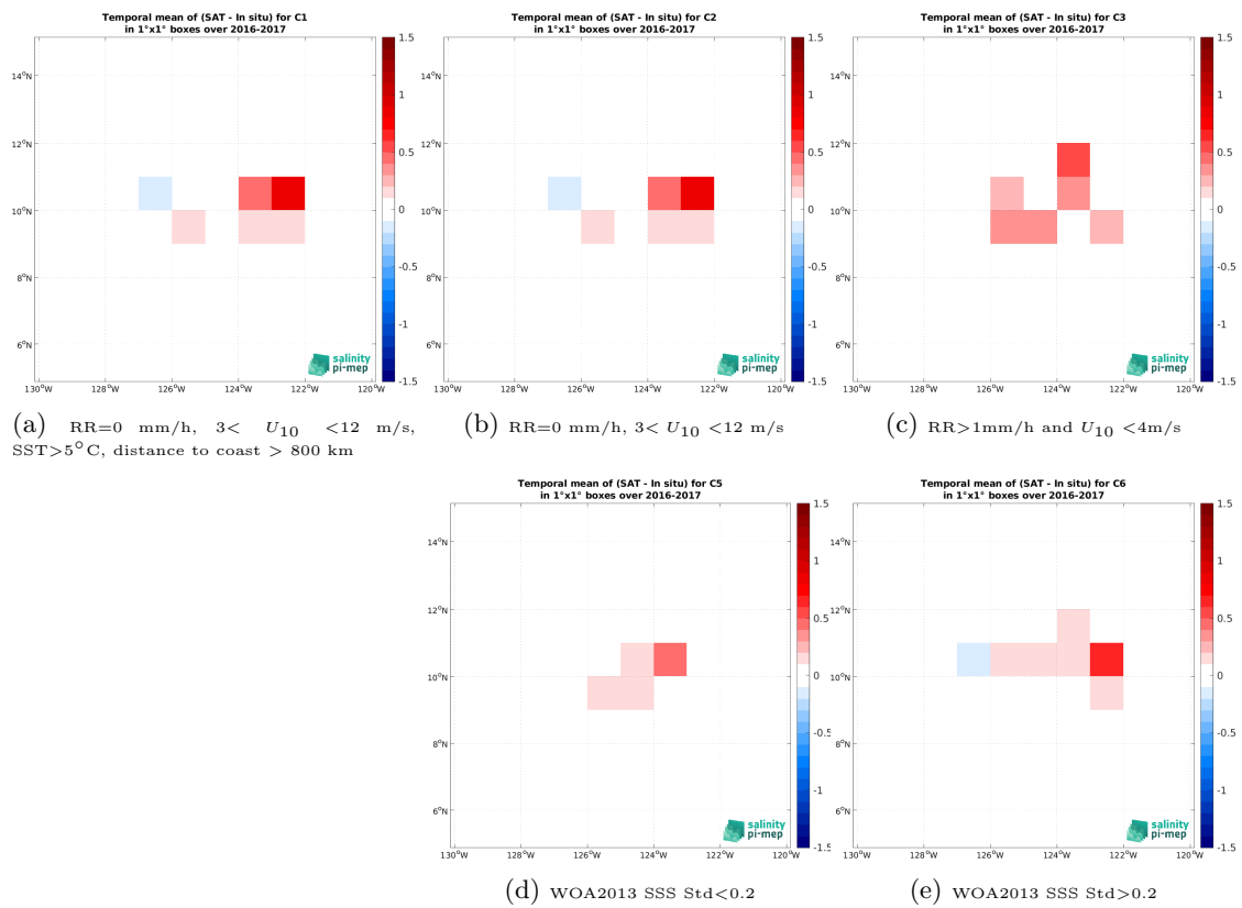
Figure 14: Temporal mean gridded over spatial boxes of size 1^\circ \times 1^\circ of \Delta SSS (CCI SSS L4 Merged-OI v5.5 - 30-day running (ESA) - Seaglider (SPURS 2)) for 5 different subdatasets corresponding to:RR=0 mm/h, 3 < U_{10} < 12 m/s, SST >5^\circ C, distance to coast > 800 km (a), RR=0 mm/h, 3 < U_{10} < 12 m/s (b), RR >1 mm/h and U_{10} < 4 m/s (c), WOA2013 SSS Std <0.2 (d), WOA2013 SSS Std >0.2 (e).
