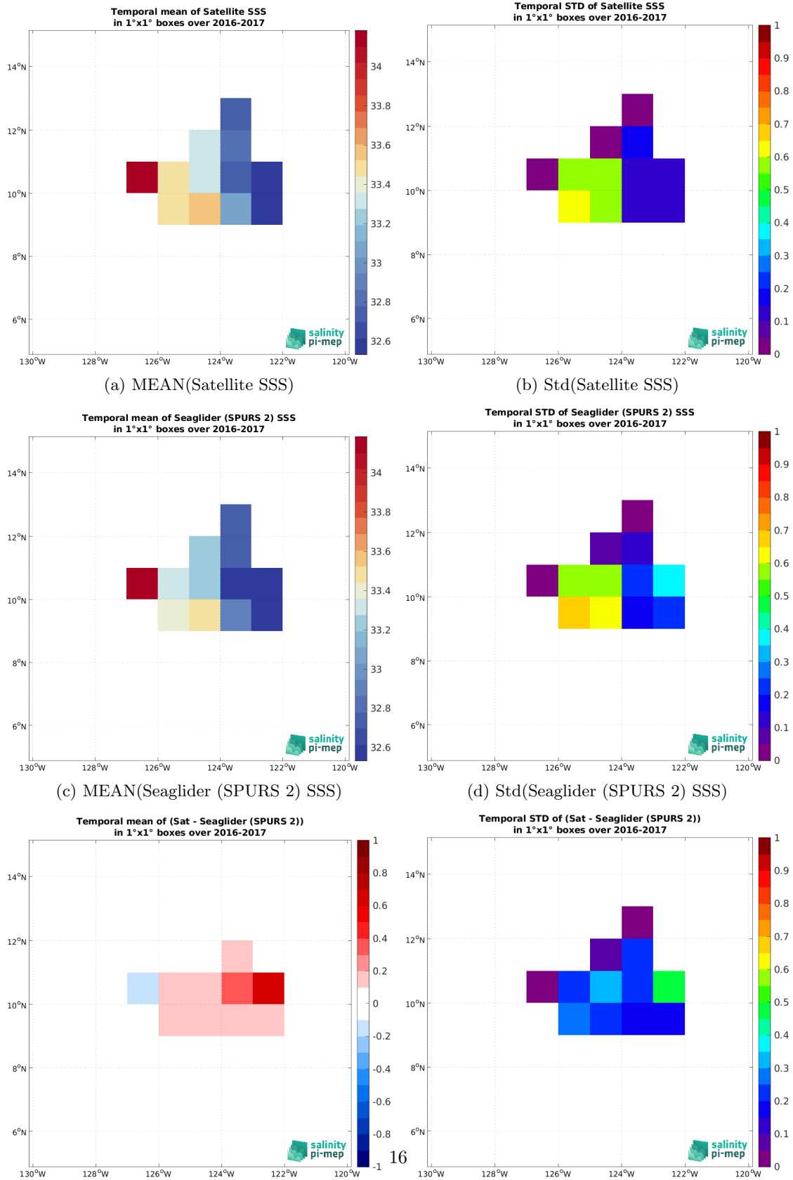
Figure 7: Temporal mean (left) and Std (right) of SSS from CCI SSS L4 Merged-OI v5.5 - 30-day running (ESA) (top), Seaglider (SPURS 2) (middle), and of \Delta SSS (Satellite - Seaglider (SPURS 2)). Only match-up pairs are used to generate these maps.
