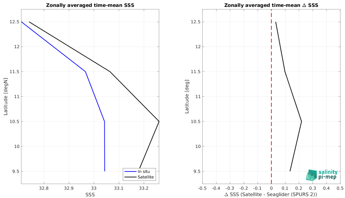
Figure 9: Left panel: Zonal mean SSS from CCI SSS L4 Merged-OI v5.5 - 30-day running (ESA) satellite product (black) and from Seaglider (SPURS 2) (blue). Right panel: Zonal mean of \Delta SSS (Satellite - Seaglider (SPURS 2)) for all the collected Pi-MEP match-up pairs estimated over the full satellite product period.
