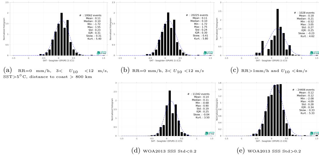
Figure 15: Normalized histogram of \Delta SSS (CCI SSS L4 Merged-OI v5.5 - 30-day running (ESA) - Seaglider (SPURS 2)) for 5 different subdatasets corresponding to: RR=0 mm/h, 3 < U_{10} < 12 m/s, SST>5°C, distance to coast > 800 km (a), RR=0 mm/h, 3 < U_{10} < 12 m/s (b), RR>1mm/h and U_{10} < 4 m/s (c), WOA2013 SSS Std<0.2 (d), WOA2013 SSS Std>0.2 (e).
