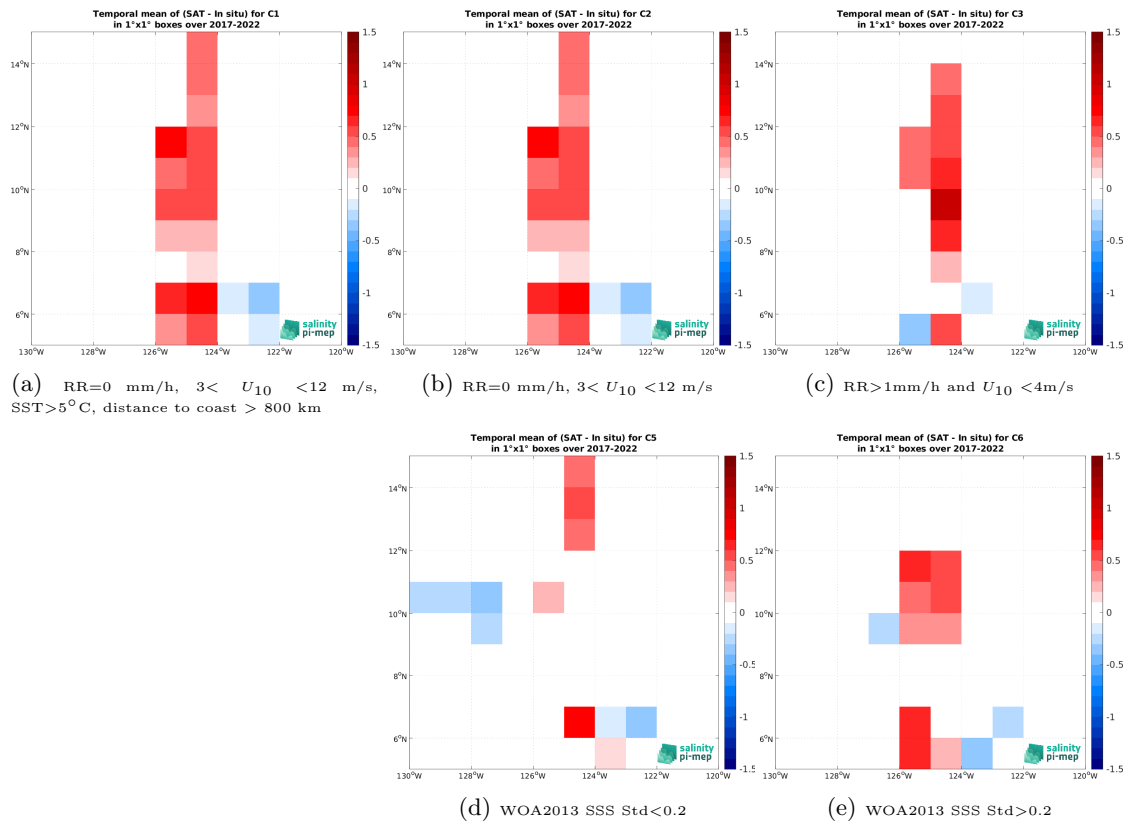
Figure 14: Temporal mean gridded over spatial boxes of size 1^\circ \times 1^\circ of \Delta\text{SSS} (CCI SSS L4 Merged-OI v5.5 - 30-day running (ESA) - Saildrone) for 5 different subdatasets corresponding to:RR=0 mm/h, 3 < U_{10} < 12 m/s, SST>5°C, distance to coast > 800 km (a), RR=0 mm/h, 3 < U_{10} < 12 m/s (b), RR>1mm/h and U_{10} < 4 m/s (c), WOA2013 SSS Std<0.2 (d), WOA2013 SSS Std>0.2 (e).
