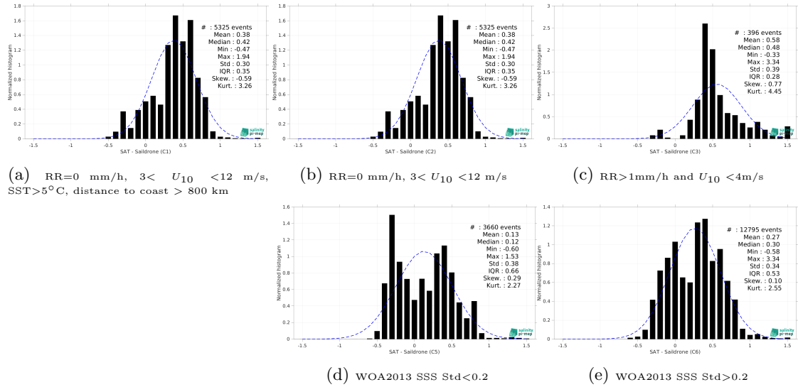
Figure 15: Normalized histogram of \Delta SSS (CCI SSS L4 Merged-OI v5.5 - 30-day running (ESA) - Saildrone) for 5 different subdatasets corresponding to: RR=0 mm/h, 3 < U_{10} < 12 m/s, SST > 5°C, distance to coast > 800 km (a), RR=0 mm/h, 3 < U_{10} < 12 m/s (b), RR > 1mm/h and U_{10} < 4 m/s (c), WOA2013 SSS Std < 0.2 (d), WOA2013 SSS Std > 0.2 (e).
