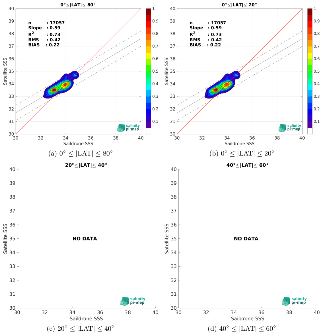
Figure 10: Contour maps of the concentration of CCI SSS L4 Merged-OI v5.5 - 30-day running (ESA) SSS (y-axis) versus Saldrone SSS (x-axis) at match-up pairs for different latitude bands. For each plot, the red line shows x=y . The black thin and dashed lines indicate a linear fit through the data cloud and the \pm 95\% confidence levels, respectively. The number match-up pairs n , the slope and R^2 coefficient of the linear fit, the root mean square (RMS) and the mean bias between satellite and in situ data are indicated for each latitude band in each plots.
