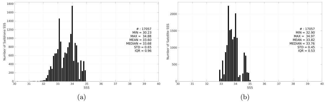
Figure 3: Histograms of SSS from Saildrone (a) and CCI SSS L4 Merged-OI v5.5 - 30-day running (ESA) (b) considering all match-up pairs per bins of 0.1 over the SPURS 2 Pi-MEP region and for the full satellite product period.
