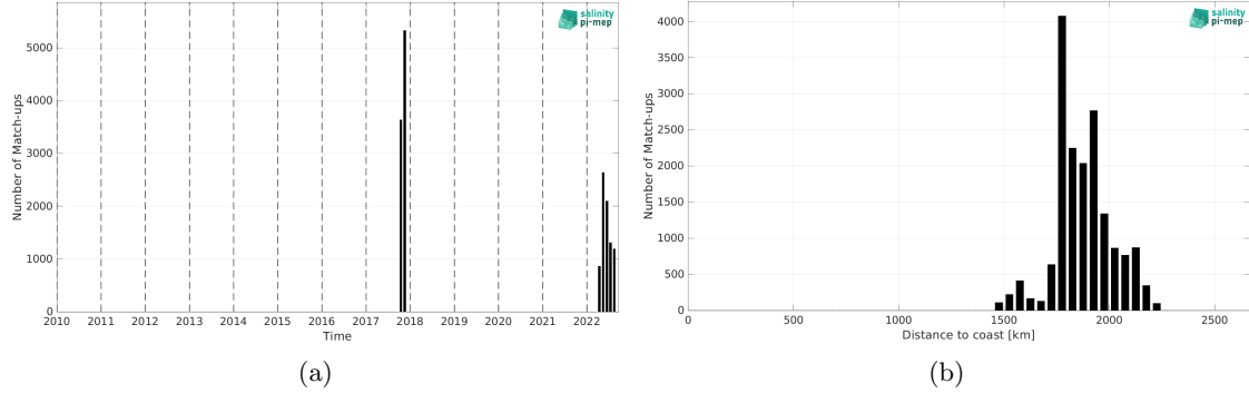
Figure 2: Number of match-ups between Saildrone and CCI SSS L4 Merged-OI v5.5 - 30-day running (ESA) SSS as a function of time (a) and as function of the distance to coast (b) over the SPURS 2 Pi-MEP region and for the full satellite product period.
