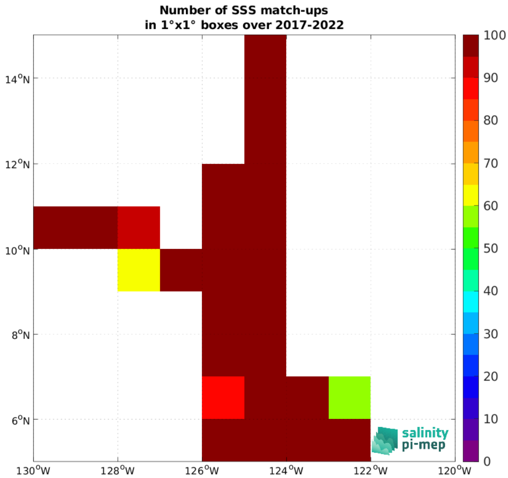
Figure 5: Number of SSS match-ups between Saildrone SSS and the CCI SSS L4 Merged-OI v5.5 - 30-day running (ESA) SSS product for the SPURS 2 Pi-MEP region over 1°x1° boxes and for the full satellite product period.
