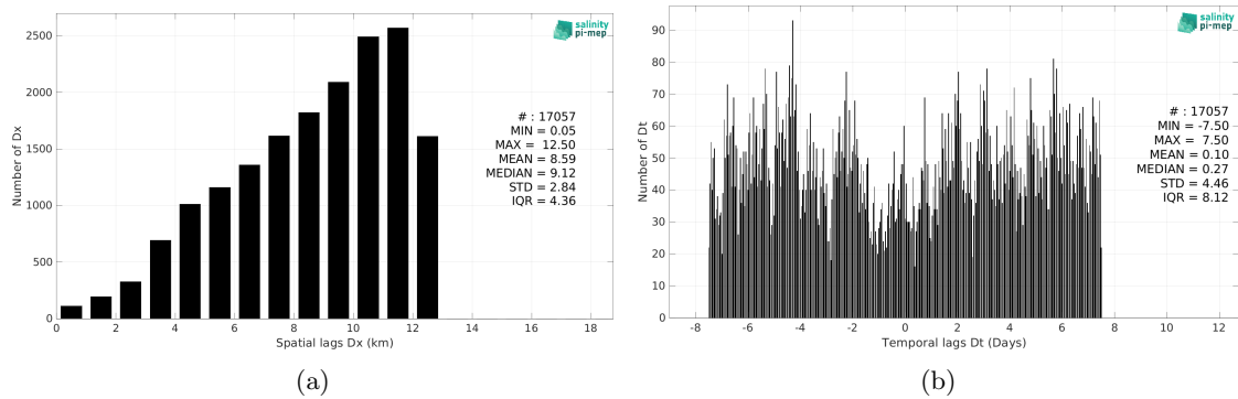
Figure 6: Histograms of the spatial (a) and temporal (b) lags between the location/time of the Saildrone measurement and the date of the corresponding CCI SSS L4 Merged-OI v5.5 - 30-day running (ESA) SSS pixel.
