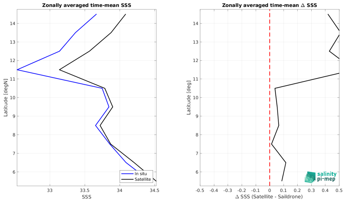
Figure 9: Left panel: Zonal mean SSS from CCI SSS L4 Merged-OI v5.5 - 30-day running (ESA) satellite product (black) and from Sairdrone (blue). Right panel: Zonal mean of \Delta SSS (Satellite - Sairdrone) for all the collected Pi-MEP match-up pairs estimated over the full satellite product period.
