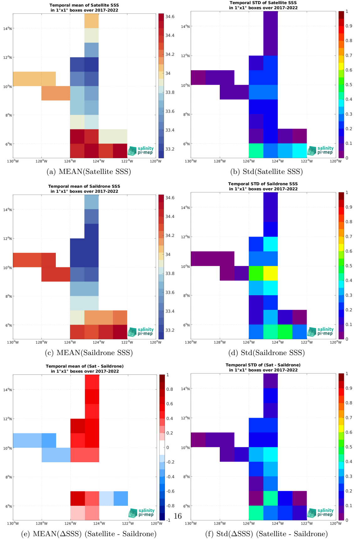
Figure 7: Temporal mean (left) and Std (right) of SSS from CCI SSS L4 Merged-OI v5.5 - 30-day running (ESA) (top), Saildrone (middle), and of \Delta SSS (Satellite - Saildrone). Only match-up pairs are used to generate these maps.
