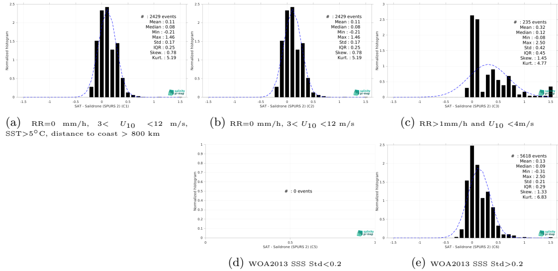
Figure 15: Normalized histogram of \Delta SSS (CCI SSS L4 Merged-OI v5.5 - 30-day running (ESA) - Saildrone (SPURS 2)) for 5 different subdatasets corresponding to: RR=0 mm/h, 3 < U_{10} < 12 m/s, SST>5°C, distance to coast > 800 km (a), RR=0 mm/h, 3 < U_{10} < 12 m/s (b), RR>1mm/h and U_{10} < 4 m/s (c), WOA2013 SSS Std<0.2 (d), WOA2013 SSS Std>0.2 (e).
