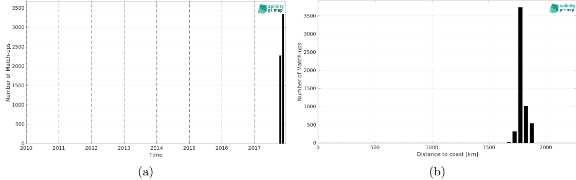
Figure 2: Number of match-ups between Saildrone (SPURS 2) and CCI SSS L4 Merged-OI v5.5 - 30-day running (ESA) SSS as a function of time (a) and as function of the distance to coast (b) over the SPURS 2 Pi-MEP region and for the full satellite product period.
