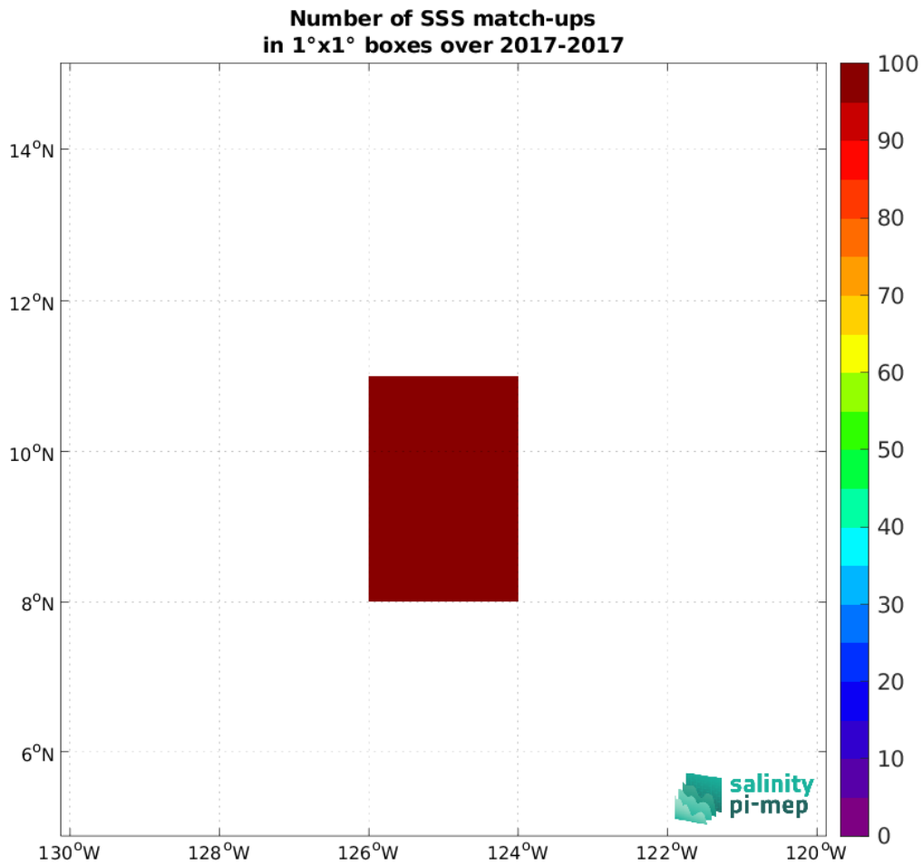
Figure 5: Number of SSS match-ups between Saildrone (SPURS 2) SSS and the CCI SSS L4 Merged-OI v5.5 - 30-day running (ESA) SSS product for the SPURS 2 Pi-MEP region over 1^\circ \times 1^\circ boxes and for the full satellite product period.
