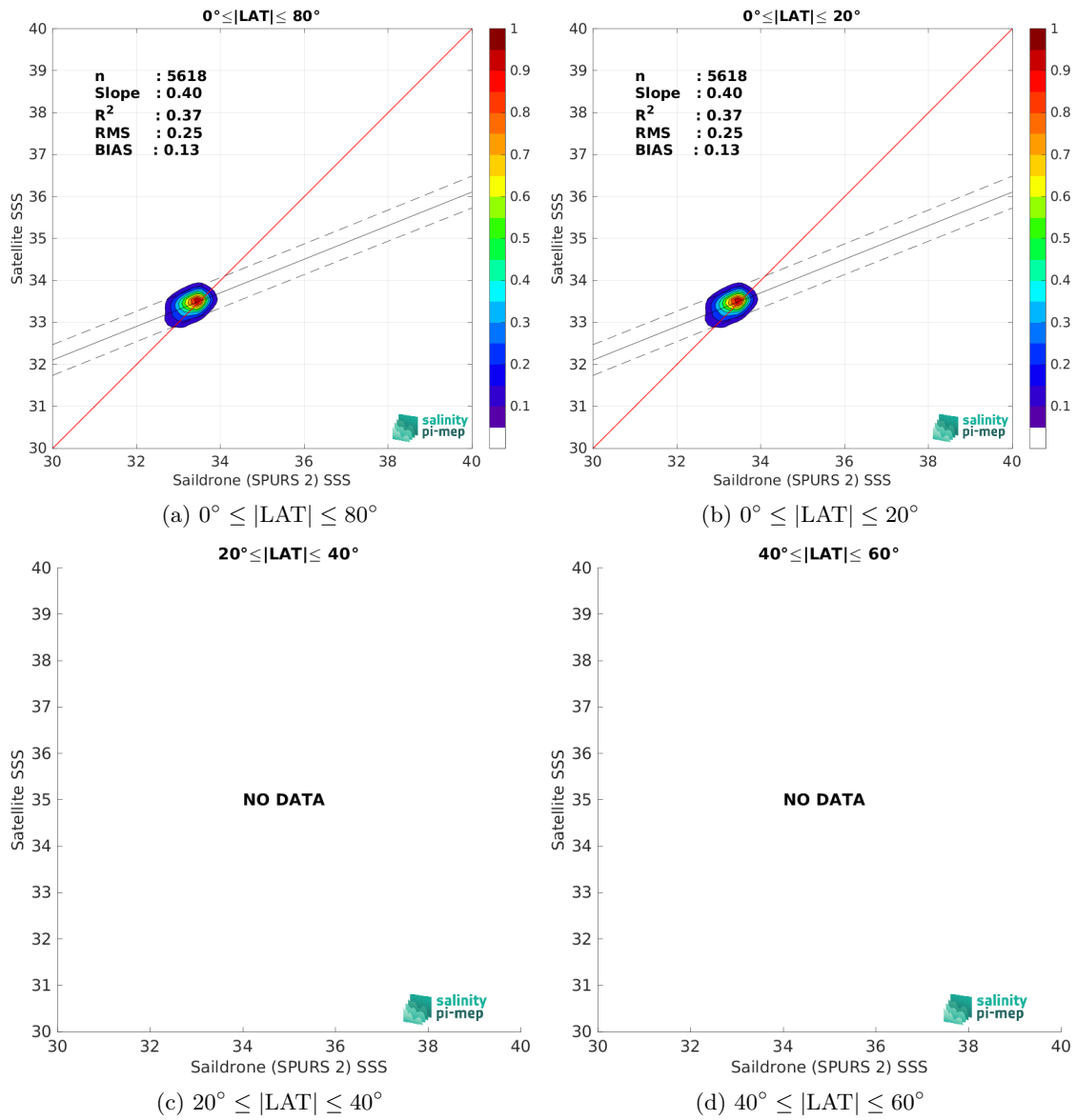
Figure 10: Contour maps of the concentration of CCI SSS L4 Merged-OI v5.5 - 30-day running (ESA) SSS (y-axis) versus Saildrone (SPURS 2) SSS (x-axis) at match-up pairs for different latitude bands. For each plot, the red line shows x=y . The black thin and dashed lines indicate a linear fit through the data cloud and the \pm 95\% confidence levels, respectively. The number match-up pairs n , the slope and R^2 coefficient of the linear fit, the root mean square (RMS) and the mean bias between satellite and in situ data are indicated for each latitude band in each plots.
