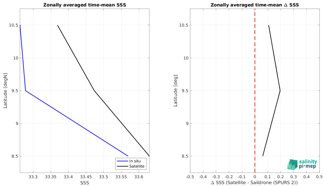
Figure 9: Left panel: Zonal mean SSS from CCI SSS L4 Merged-OI v5.5 - 30-day running (ESA) satellite product (black) and from Saildrone (SPURS 2) (blue). Right panel: Zonal mean of \Delta SSS (Satellite - Saildrone (SPURS 2)) for all the collected Pi-MEP match-up pairs estimated over the full satellite product period.
