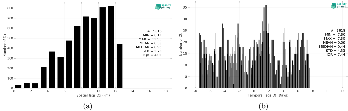
Figure 6: Histograms of the spatial (a) and temporal (b) lags between the location/time of the Saildrone (SPURS 2) measurement and the date of the corresponding CCI SSS L4 Merged-OI v5.5 - 30-day running (ESA) SSS pixel.
