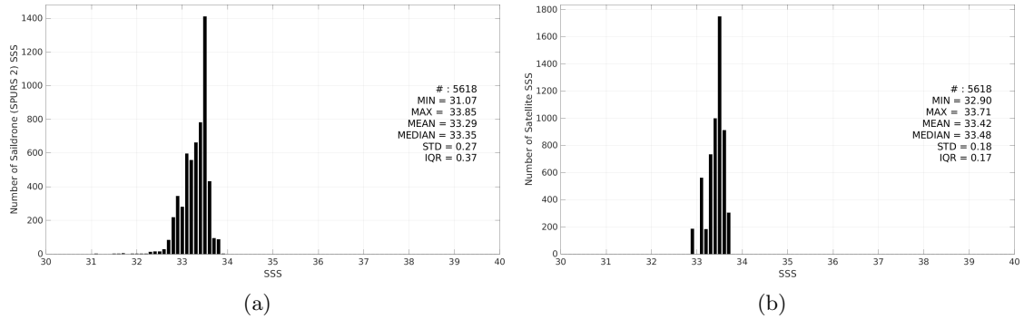
Figure 3: Histograms of SSS from Saildrone (SPURS 2) (a) and CCI SSS L4 Merged-OI v5.5 - 30-day running (ESA) (b) considering all match-up pairs per bins of 0.1 over the SPURS 2 Pi-MEP region and for the full satellite product period.
