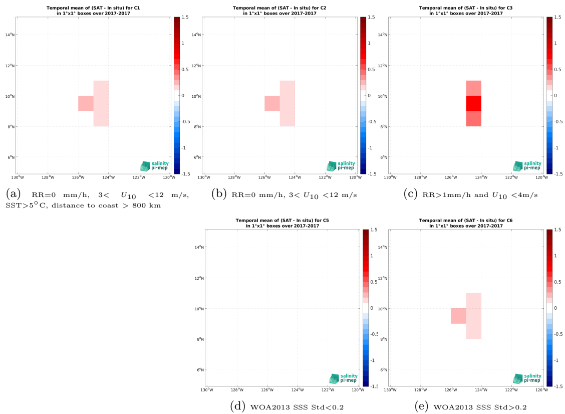
Figure 14: Temporal mean gridded over spatial boxes of size 1^\circ \times 1^\circ of \Delta SSS (CCI SSS L4 Merged-OI v5.5 - 30-day running (ESA) - Saildrone (SPURS 2)) for 5 different subdatasets corresponding to:RR=0 mm/h, 3 < U_{10} < 12 m/s, SST >5^\circ C, distance to coast > 800 km (a), RR=0 mm/h, 3 < U_{10} < 12 m/s (b), RR >1 mm/h and U_{10} < 4 m/s (c), WOA2013 SSS Std <0.2 (d), WOA2013 SSS Std >0.2 (e).
