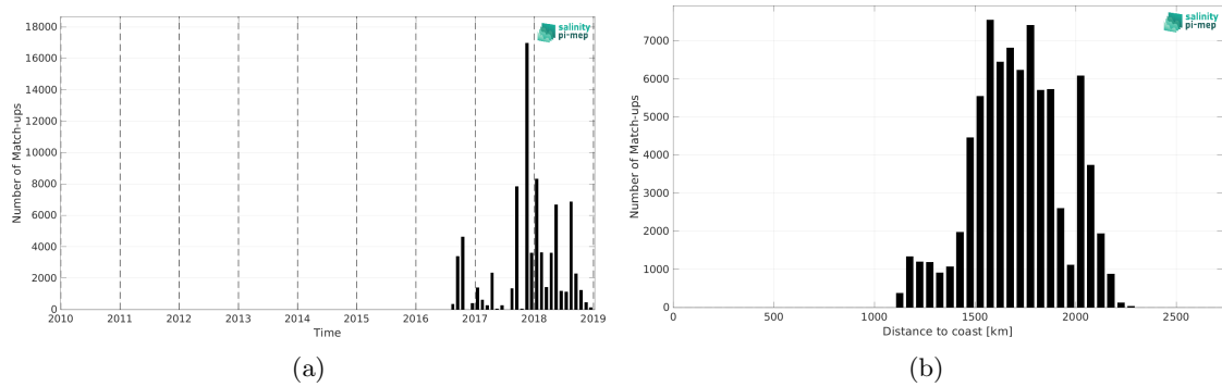
Figure 2: Number of match-ups between Surface drifters and CCI SSS L4 Merged-OI v5.5 - 30-day running (ESA) SSS as a function of time (a) and as function of the distance to coast (b) over the SPURS 2 Pi-MEP region and for the full satellite product period.
