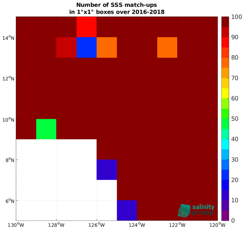
Figure 4: Number of SSS match-ups between Surface drifters SSS and the CCI SSS L4 Merged-OI v5.5 - 30-day running (ESA) SSS product for the SPURS 2 Pi-MEP region over 1°x1° boxes and for the full satellite product period.
