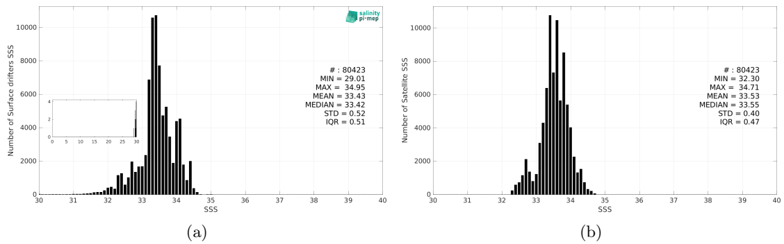
Figure 3: Histograms of SSS from Surface drifters (a) and CCI SSS L4 Merged-OI v5.5 - 30-day running (ESA) (b) considering all match-up pairs per bins of 0.1 over the SPURS 2 Pi-MEP region and for the full satellite product period.
