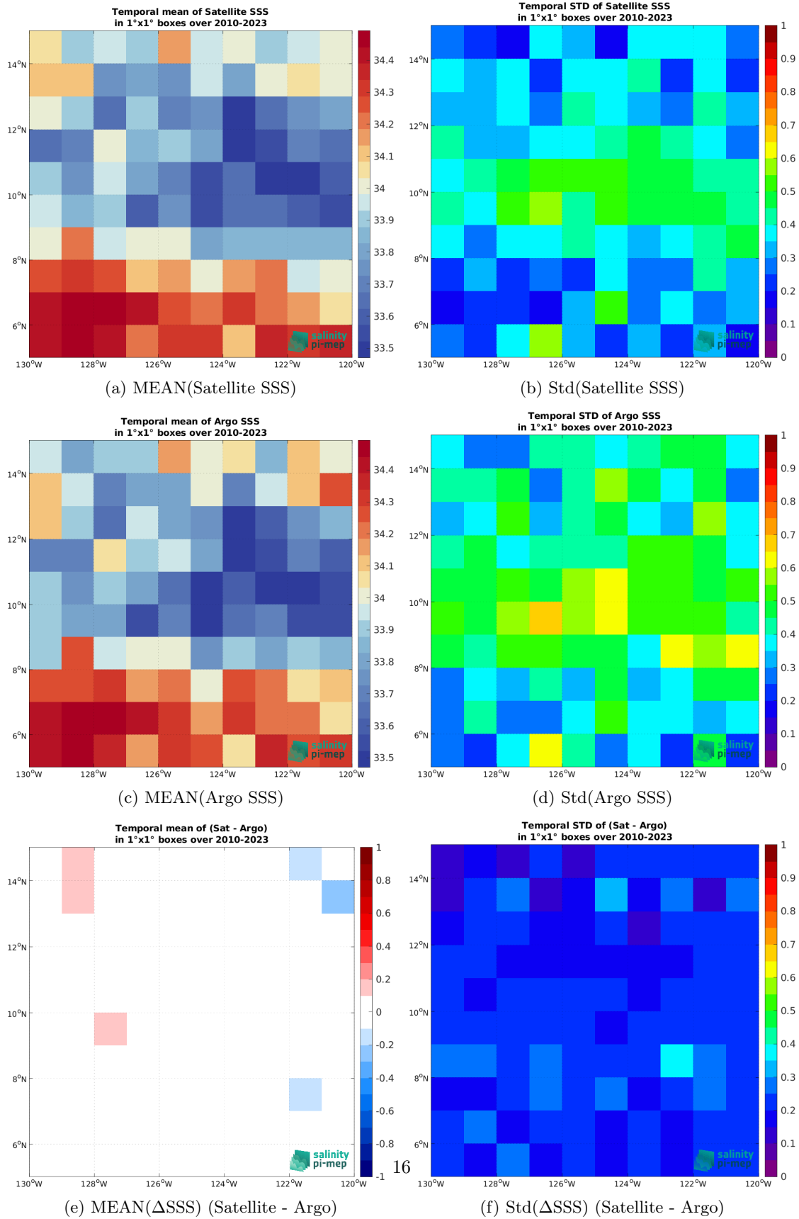
Figure 7: Temporal mean (left) and Std (right) of SSS from CCI SSS L4 Merged-OI v5.5 - 30-day running (ESA) (top), Argo (middle), and of \Delta SSS (Satellite - Argo). Only match-up pairs are used to generate these maps.
