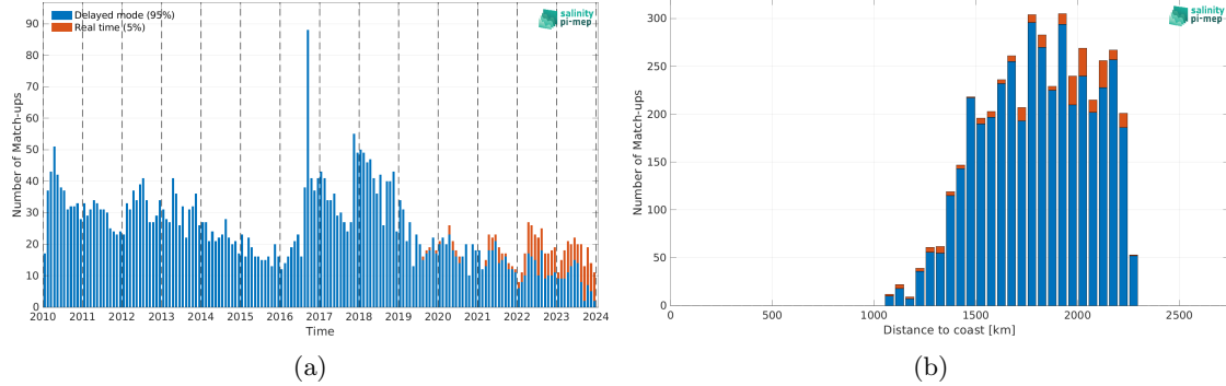
Figure 2: Number of match-ups between Argo and CCI SSS L4 Merged-OI v5.5 - 30-day running (ESA) SSS as a function of time (a) and as function of the distance to coast (b) over the SPURS 2 Pi-MEP region and for the full satellite product period.
