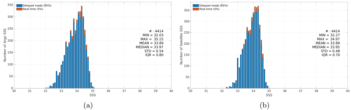
Figure 3: Histograms of SSS from Argo (a) and CCI SSS L4 Merged-OI v5.5 - 30-day running (ESA) (b) considering all match-up pairs per bins of 0.1 over the SPURS 2 Pi-MEP region and for the full satellite product period.
