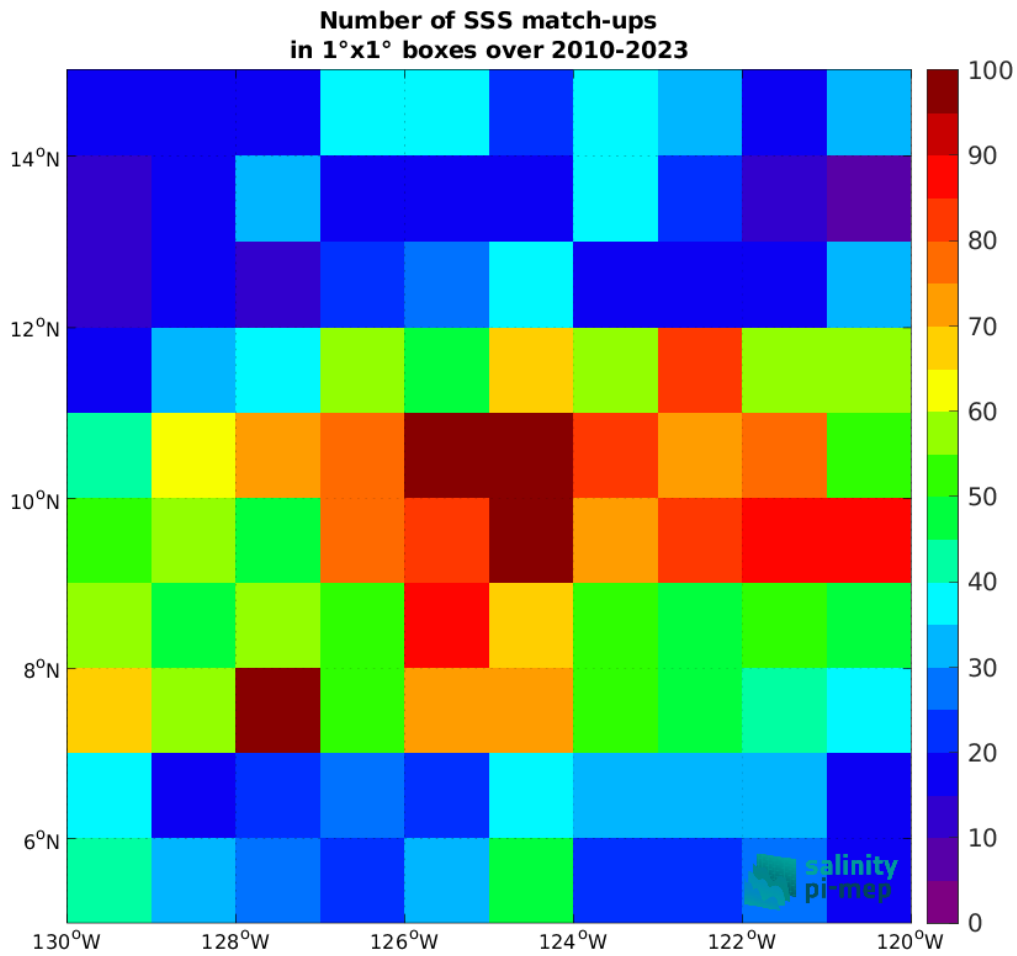
Figure 5: Number of SSS match-ups between Argo SSS and the CCI SSS L4 Merged-OI v5.5 - 30-day running (ESA) SSS product for the SPURS 2 Pi-MEP region over 1°x1° boxes and for the full satellite product period.
