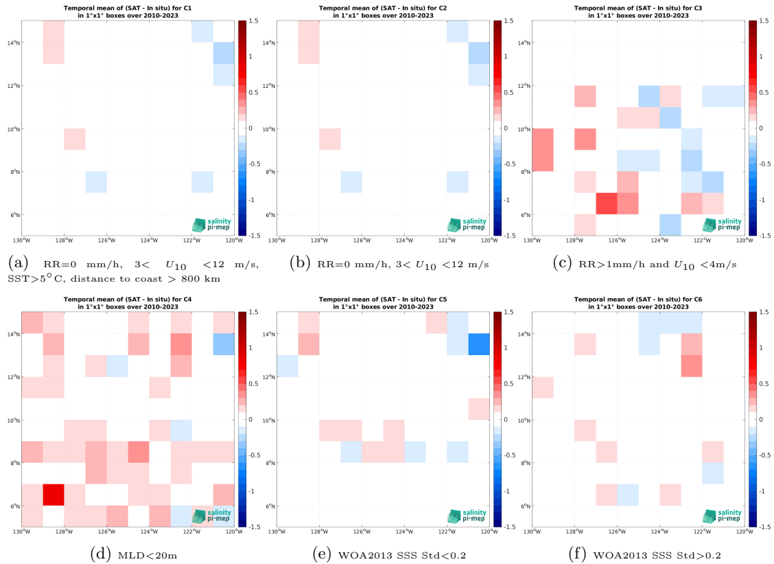
Figure 14: Temporal mean gridded over spatial boxes of size 1^\circ \times 1^\circ of \Delta SSS (CCI SSS L4 Merged-OI v5.5 - 30-day running (ESA) - Argo) for 6 different subdatasets corresponding to:RR=0 mm/h, 3 < U_{10} < 12 m/s, SST >5^\circ C, distance to coast > 800 km (a), RR=0 mm/h, 3 < U_{10} < 12 m/s (b), RR >1 mm/h and U_{10} < 4 m/s (c),MLD <20 m (d),WOA2013 SSS Std <0.2 (e),WOA2013 SSS Std >0.2 (f).
