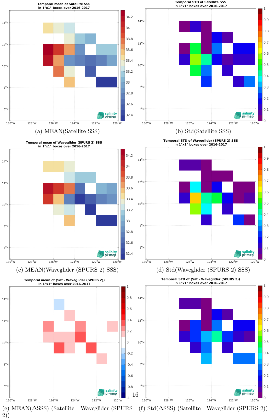
Figure 7: Temporal mean (left) and Std (right) of SSS from CCI SSS L4 Merged-OI v4.41 - 7-day running (ESA) (top), Waveglider (SPURS 2) (middle), and of \Delta SSS (Satellite - Waveglider (SPURS 2)). Only match-up pairs are used to generate these maps.
