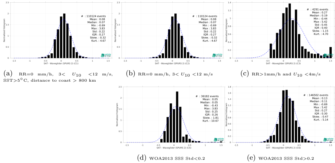
Figure 15: Normalized histogram of \Delta\text{SSS} (CCI SSS L4 Merged-OI v4.41 - 7-day running (ESA) - Waveglider (SPURS 2)) for 5 different subdatasets corresponding to: RR=0 mm/h, 3 < U_{10} < 12 m/s, SST>5°C, distance to coast > 800 km (a), RR=0 mm/h, 3 < U_{10} < 12 m/s (b), RR>1mm/h and U_{10} < 4 m/s (c), WOA2013 SSS Std<0.2 (d), WOA2013 SSS Std>0.2 (e).
