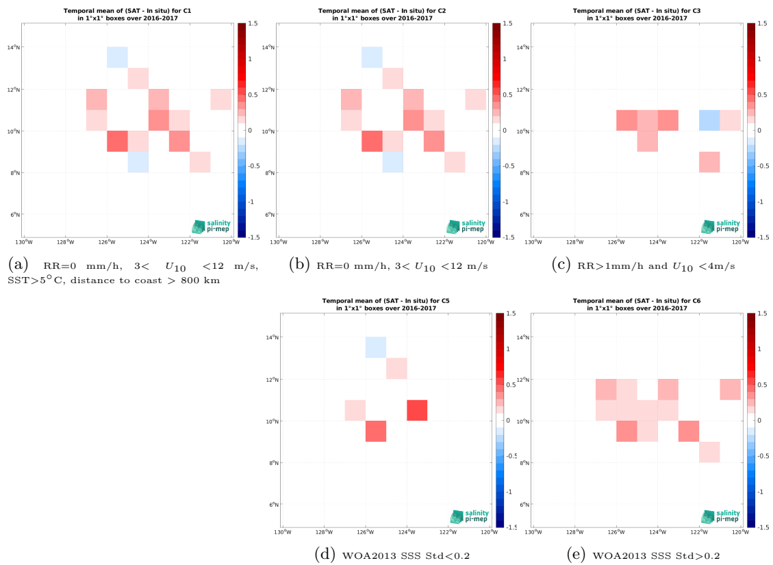
Figure 14: Temporal mean gridded over spatial boxes of size 1^\circ \times 1^\circ of \Delta SSS (CCI SSS L4 Merged-OI v4.41 - 7-day running (ESA) - Waveglider (SPURS 2)) for 5 different subdatasets corresponding to:RR=0 mm/h, 3 < U_{10} < 12 m/s, SST >5^\circ C, distance to coast > 800 km (a), RR=0 mm/h, 3 < U_{10} < 12 m/s (b), RR >1 mm/h and U_{10} < 4 m/s (c), WOA2013 SSS Std <0.2 (d), WOA2013 SSS Std >0.2 (e).
