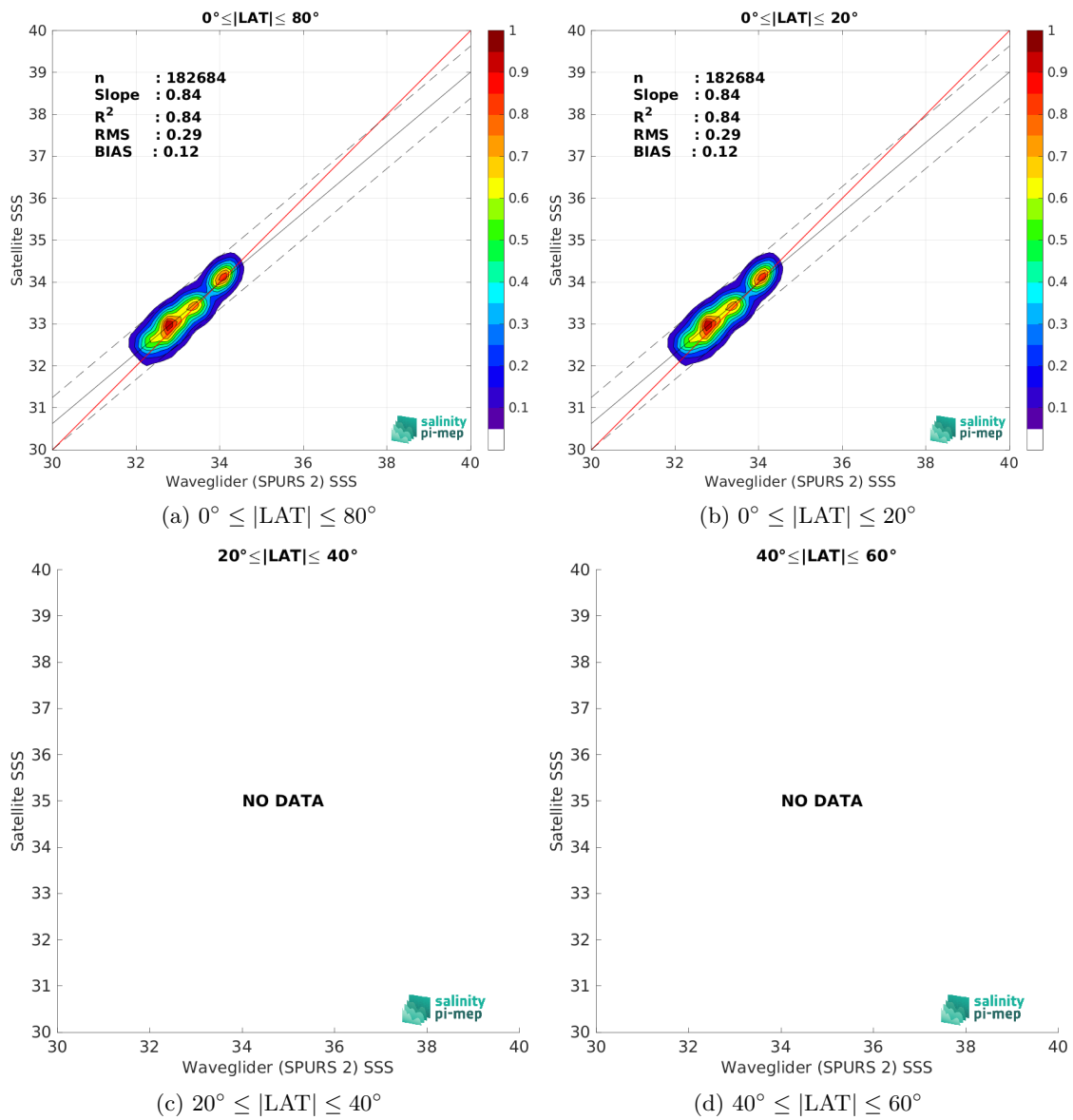
Figure 10: Contour maps of the concentration of CCI SSS L4 Merged-OI v4.41 - 7-day running (ESA) SSS (y-axis) versus Waveglider (SPURS 2) SSS (x-axis) at match-up pairs for different latitude bands. For each plot, the red line shows x=y . The black thin and dashed lines indicate a linear fit through the data cloud and the \pm 95\% confidence levels, respectively. The number match-up pairs n , the slope and R^2 coefficient of the linear fit, the root mean square (RMS) and the mean bias between satellite and in situ data are indicated for each latitude band in each plots.
