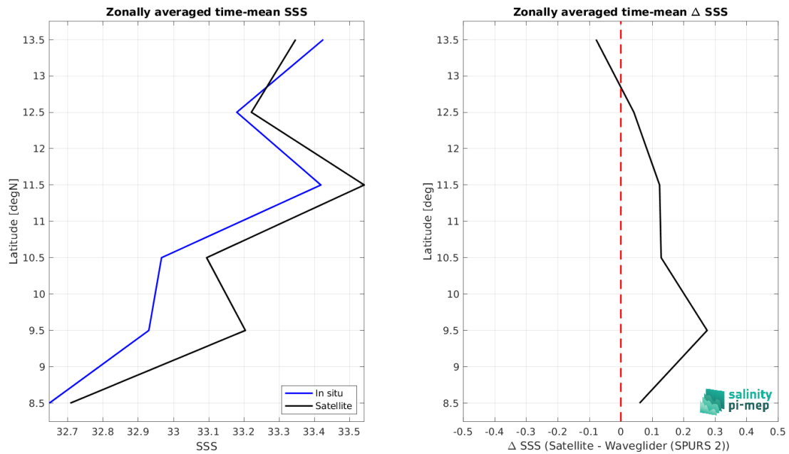
Figure 9: Left panel: Zonal mean SSS from CCI SSS L4 Merged-OI v4.41 - 7-day running (ESA) satellite product (black) and from Waveglider (SPURS 2) (blue). Right panel: Zonal mean of \Delta SSS (Satellite - Waveglider (SPURS 2)) for all the collected Pi-MEP match-up pairs estimated over the full satellite product period.
