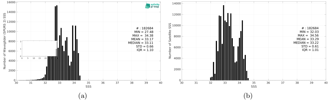
Figure 3: Histograms of SSS from Waveglider (SPURS 2) (a) and CCI SSS L4 Merged-OI v4.41 - 7-day running (ESA) (b) considering all match-up pairs per bins of 0.1 over the SPURS 2 Pi-MEP region and for the full satellite product period.
