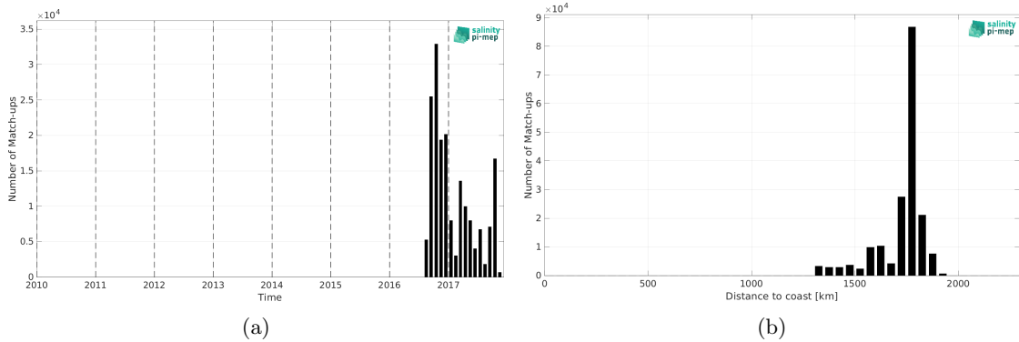
Figure 2: Number of match-ups between Waveglider (SPURS 2) and CCI SSS L4 Merged-OI v4.41 - 7-day running (ESA) SSS as a function of time (a) and as function of the distance to coast (b) over the SPURS 2 Pi-MEP region and for the full satellite product period.
